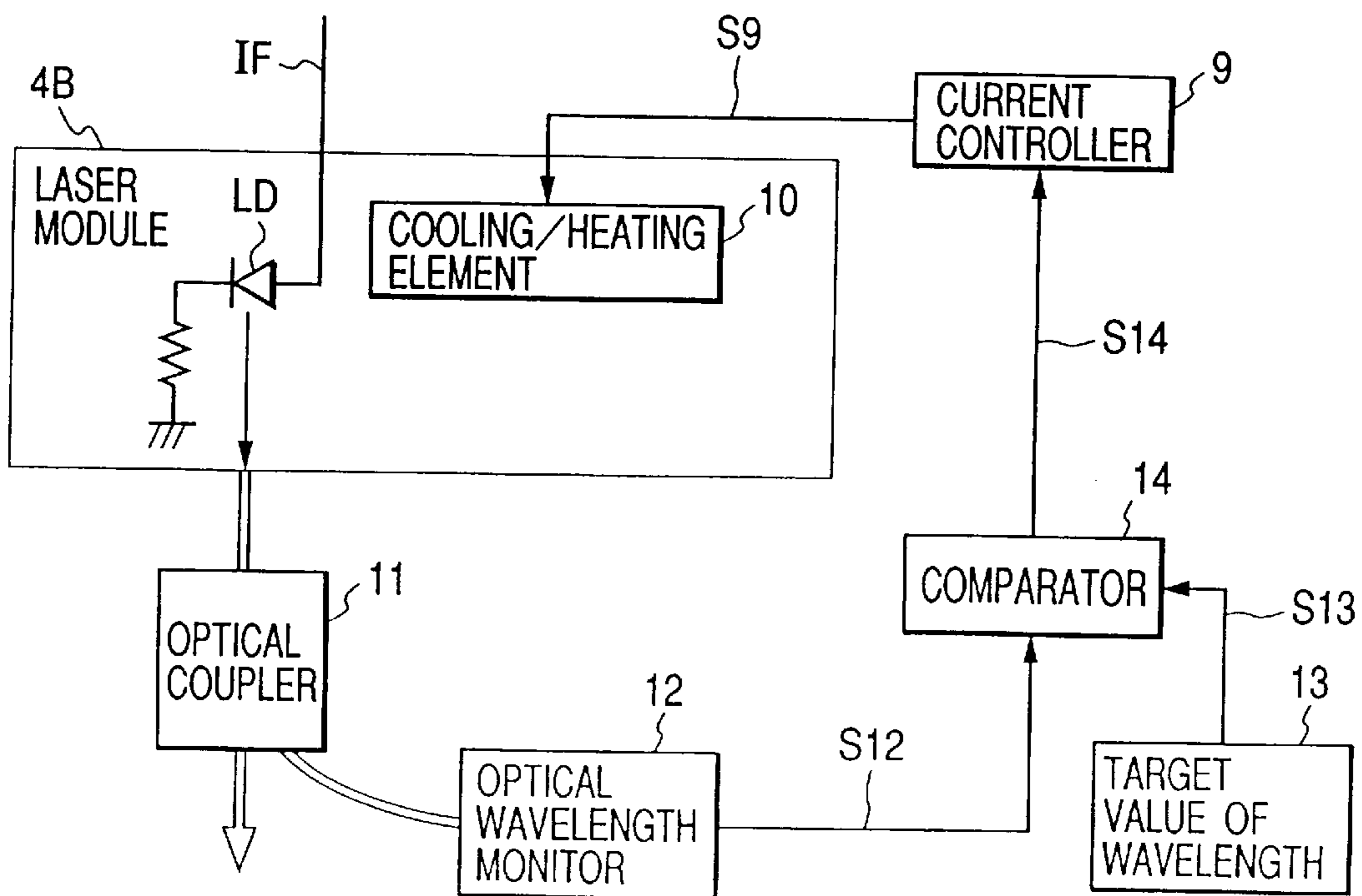
FIG. 2 PRIOR ART
