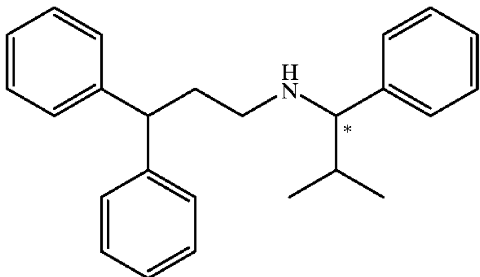
Compound 159
