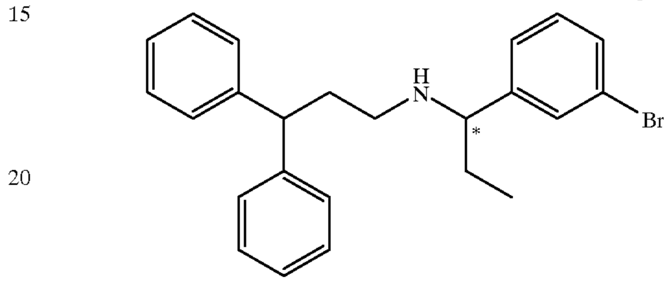
Compound 161
