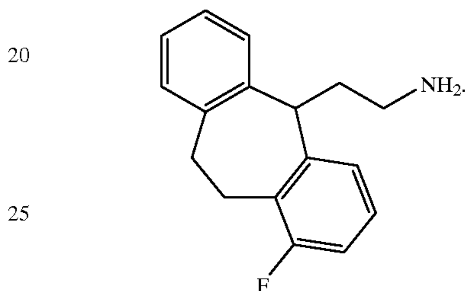
Compound 197
