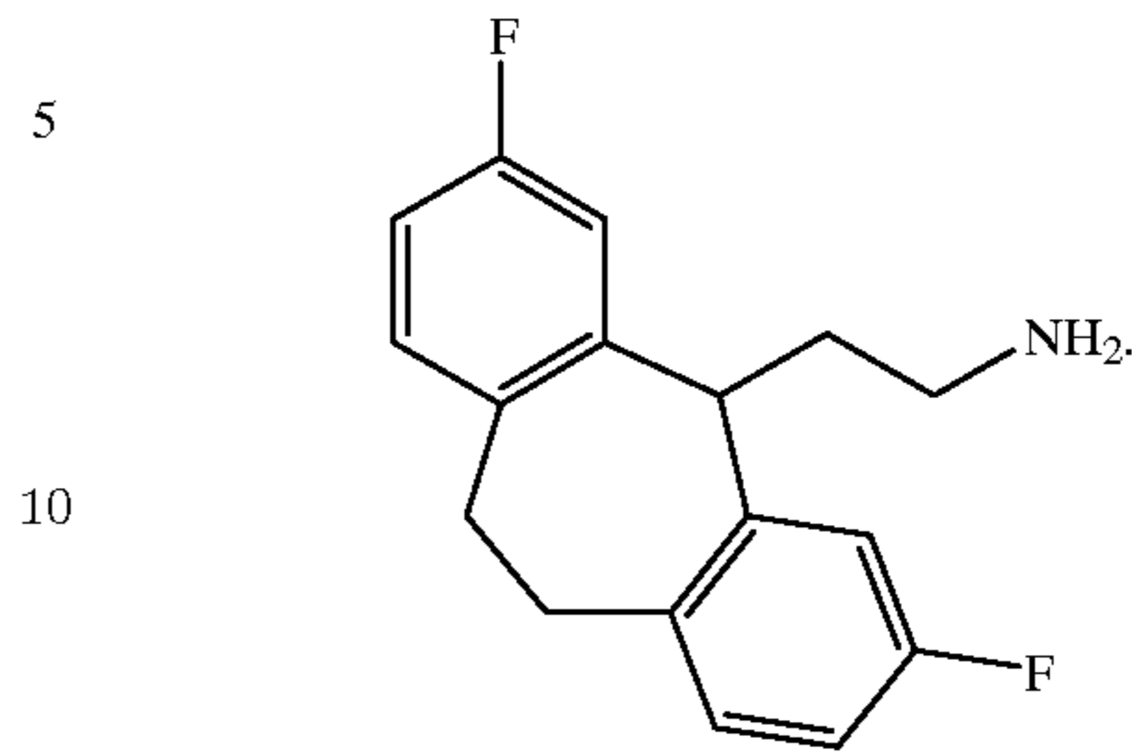
Compound 196
