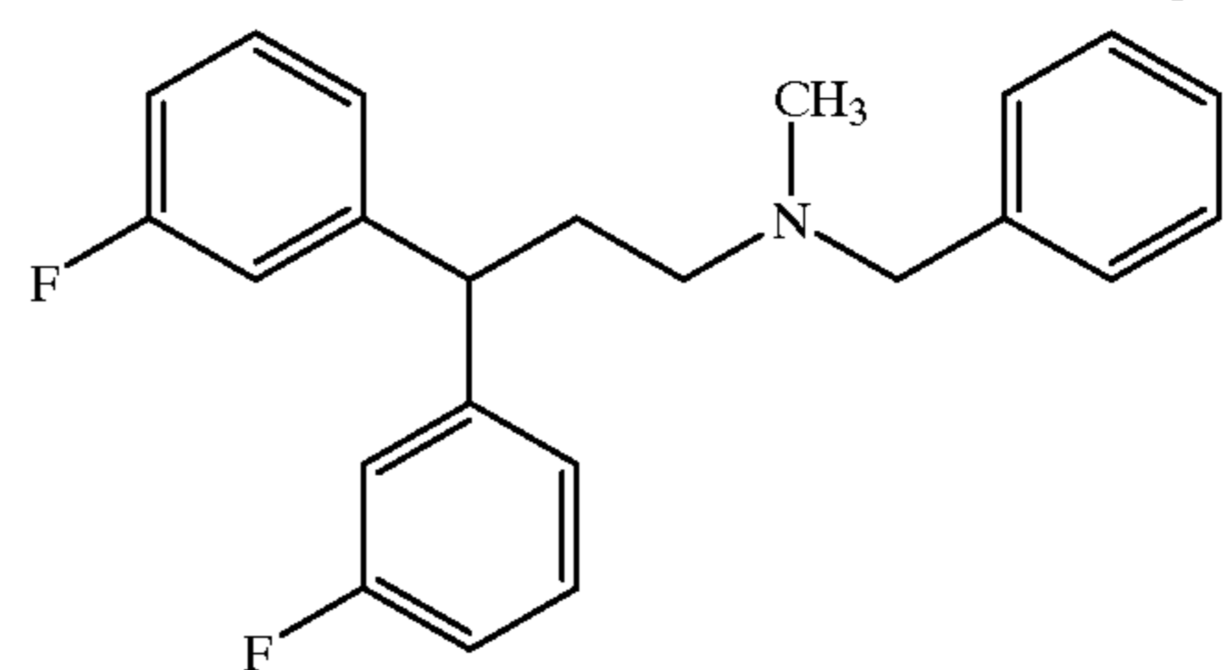
Compound 106
