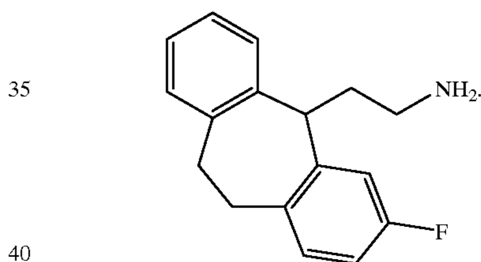
Compound 193
