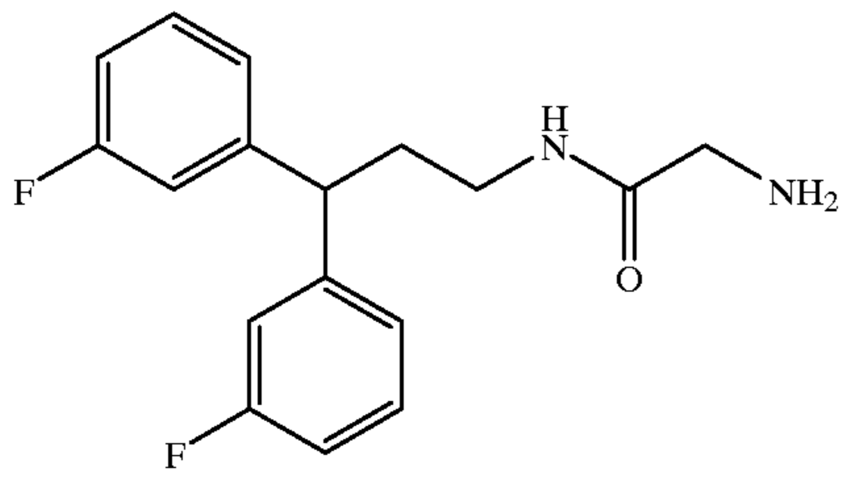
Compound 190
