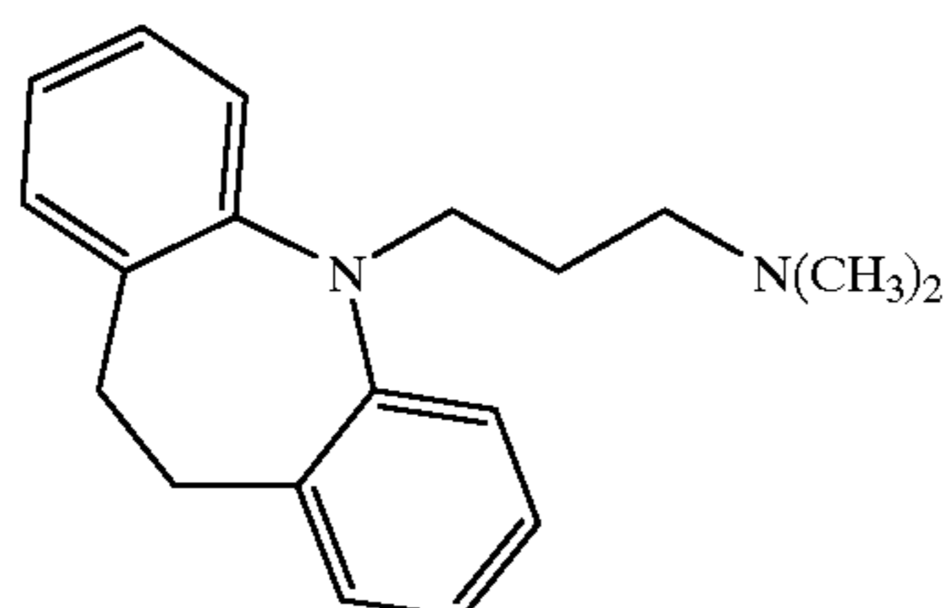
Imipramine
