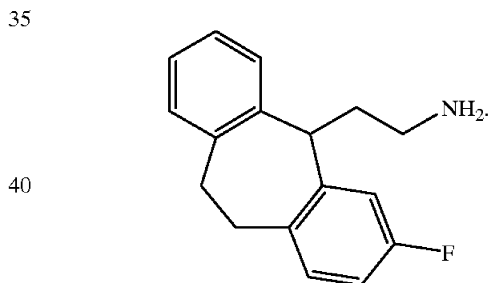
Compound 193
