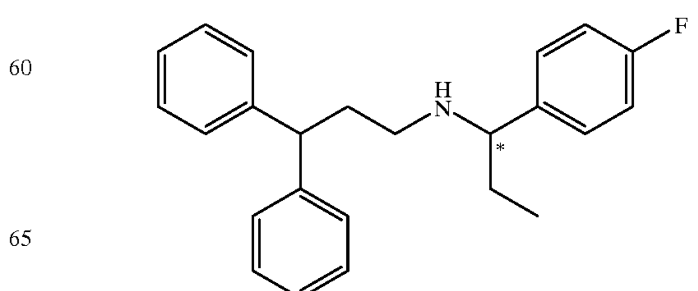
Compound 165
