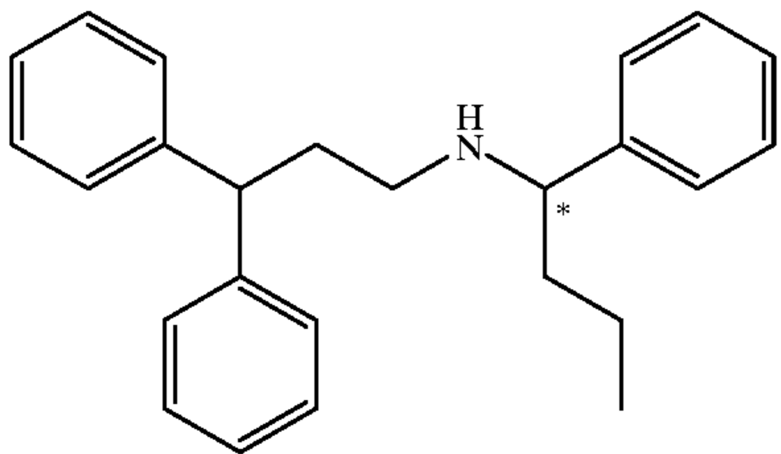
Compound 158
