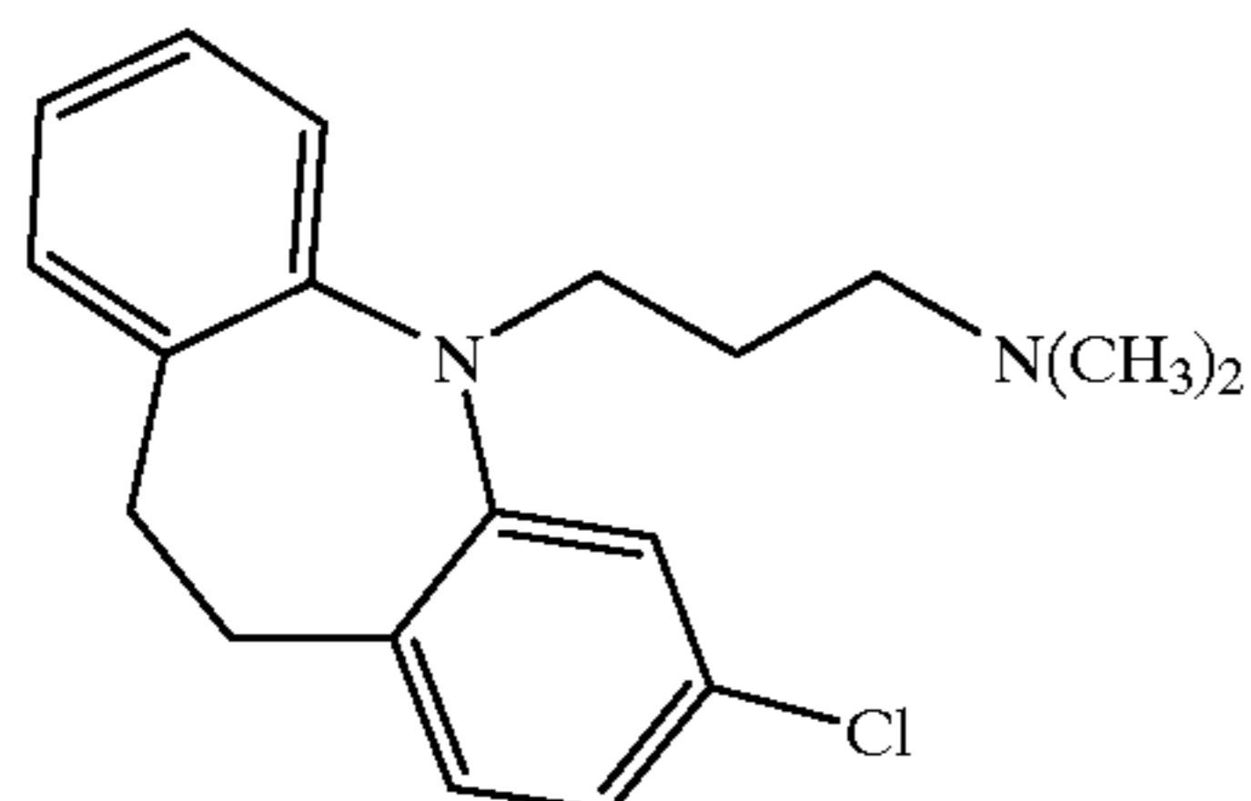
Clomipramine
