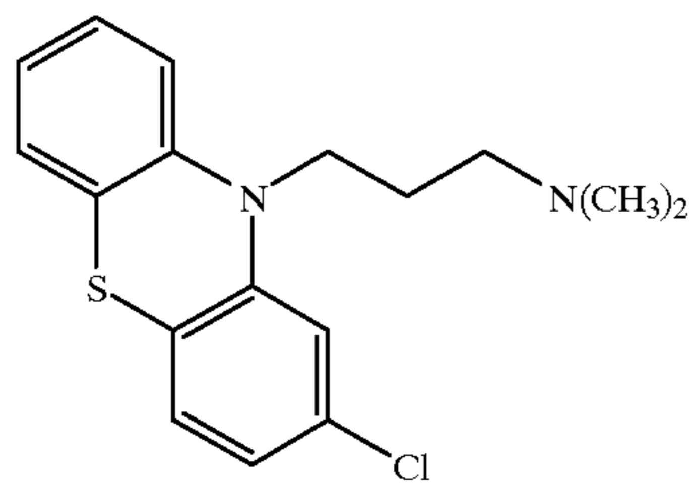
Chlorpromazine
