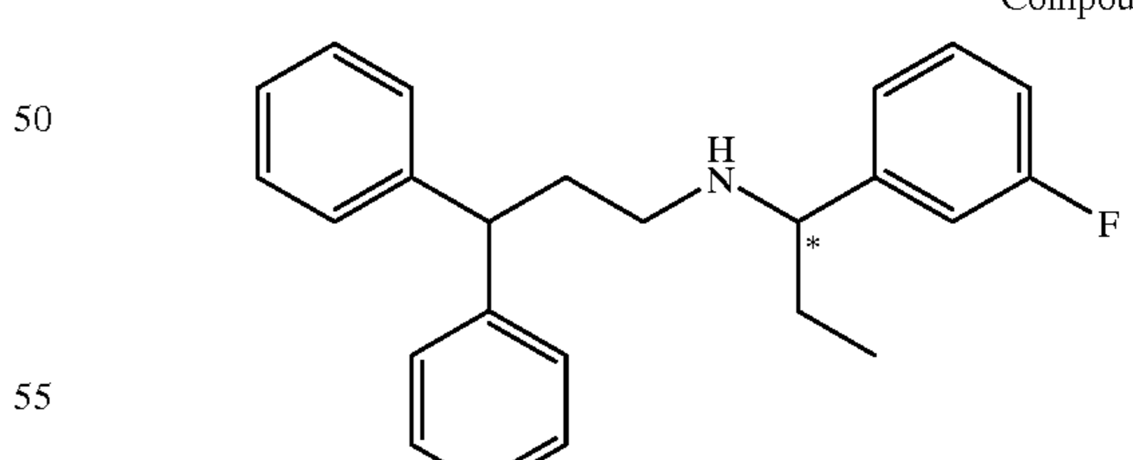
Compound 165
