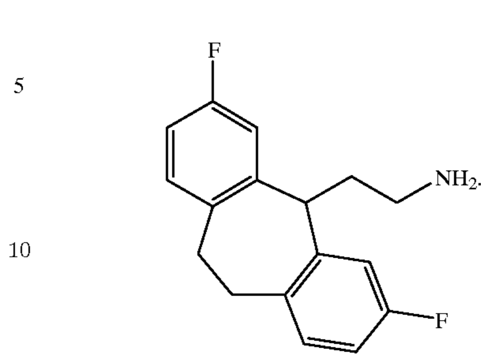
Compound 196
