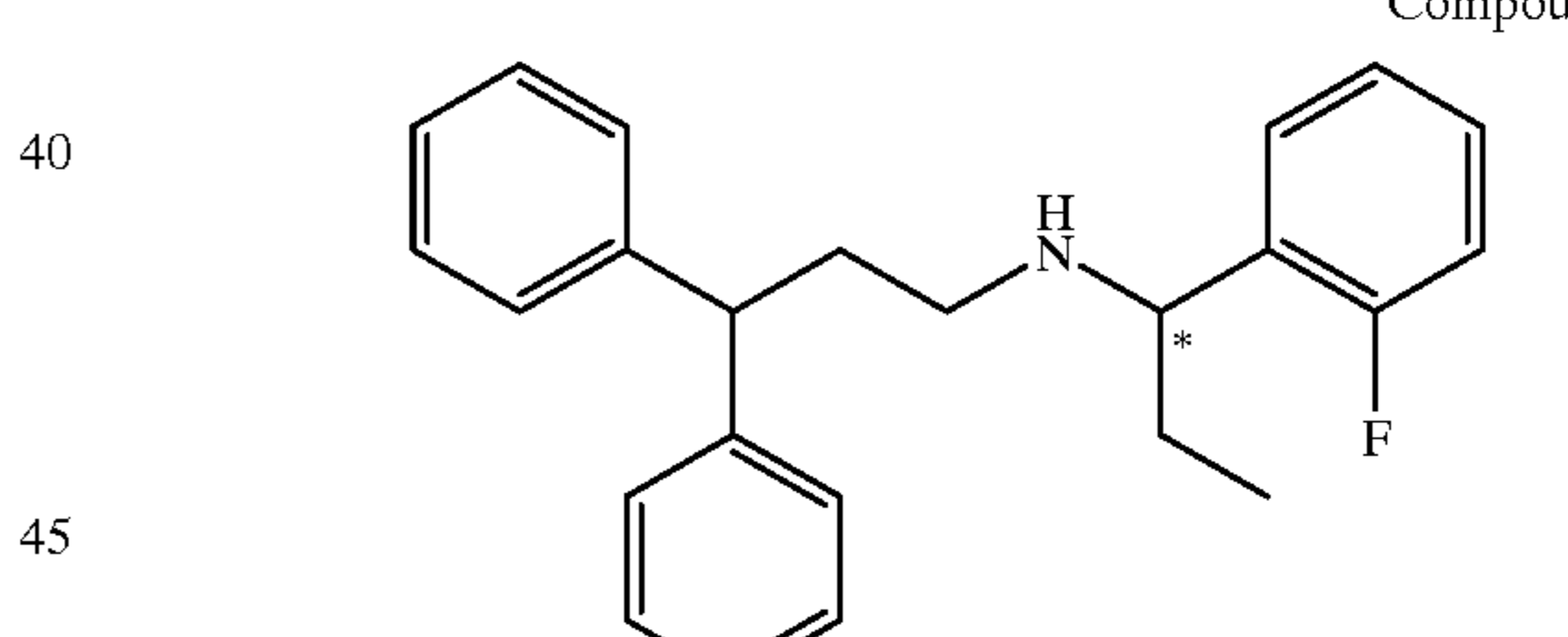
Compound 164
