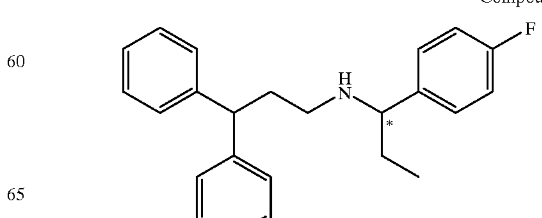
Compound 165
