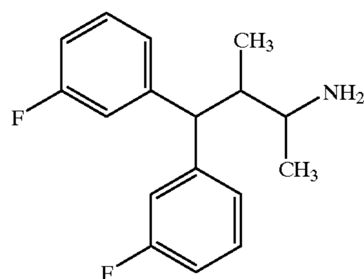
Compound 38
