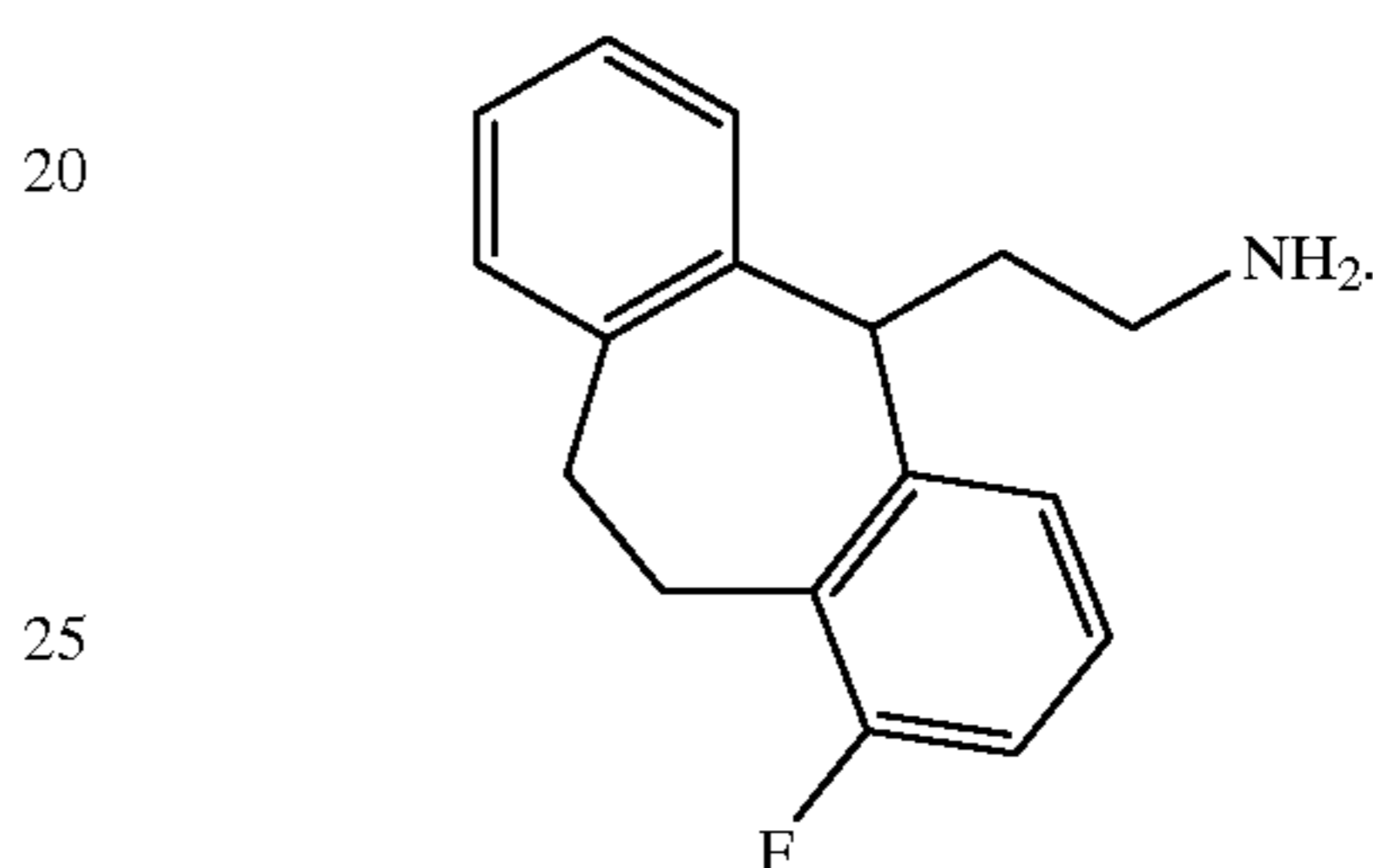
Compound 197
