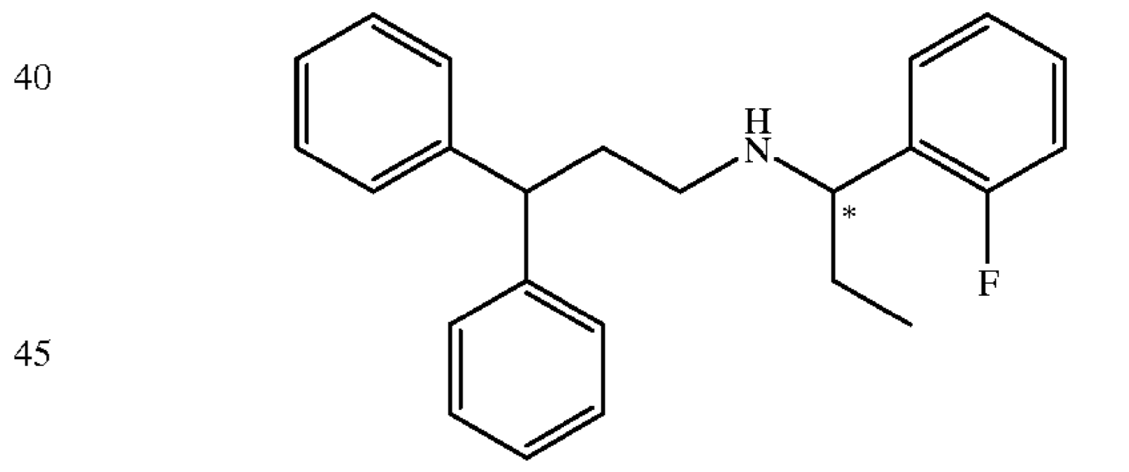
Compound 164
