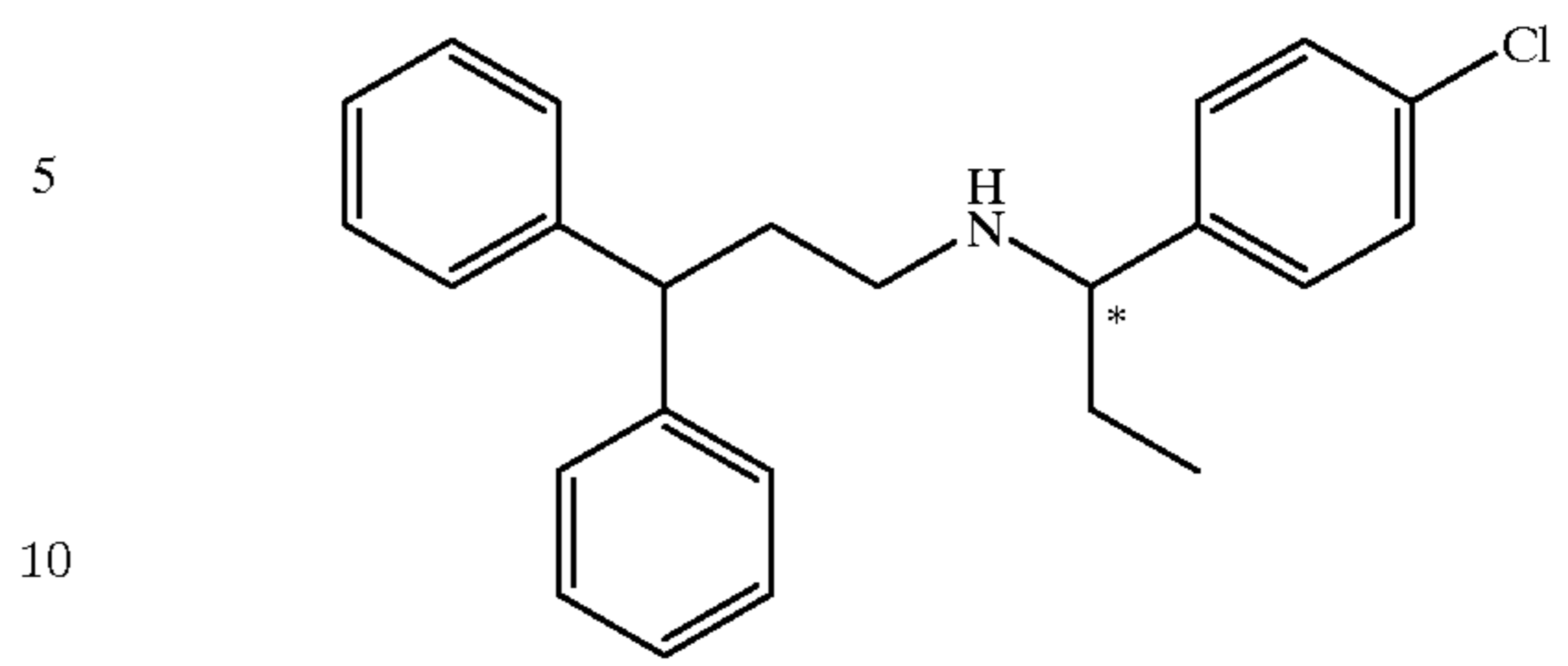
Compound 160
