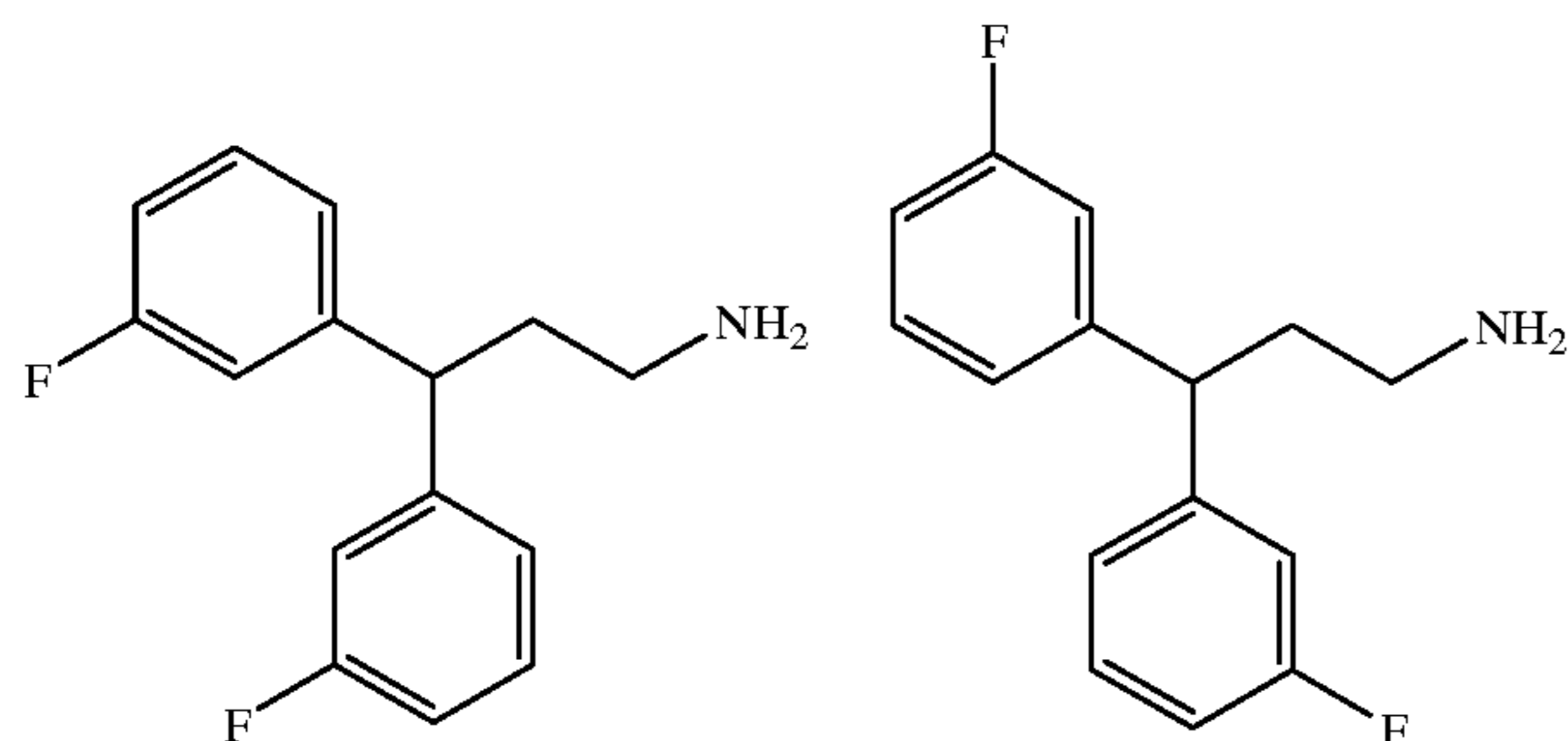
Compound 20 IC 50 (MK-801) = 252 nM
