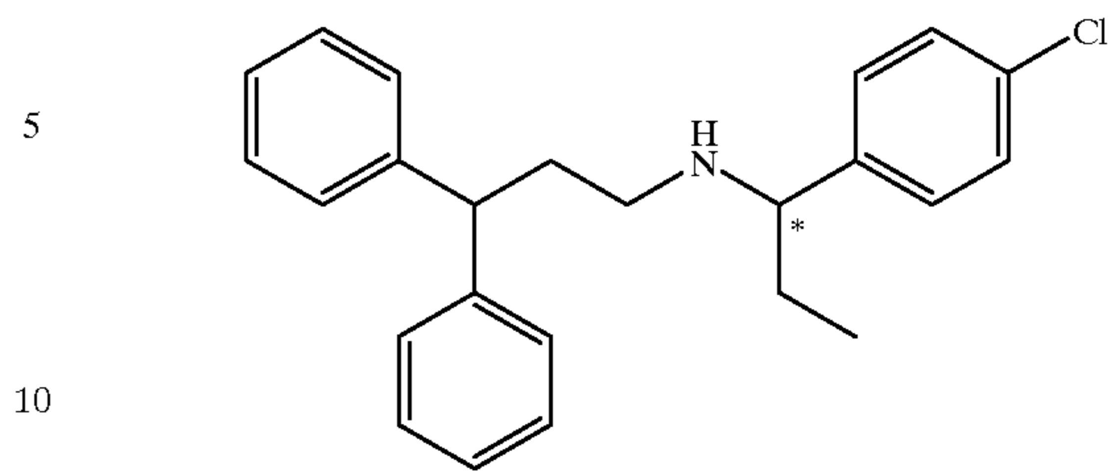
Compound 160
