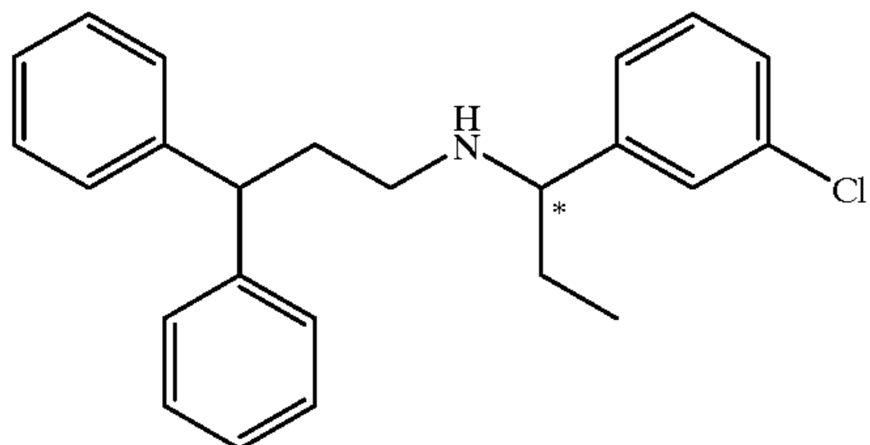
Compound 159
