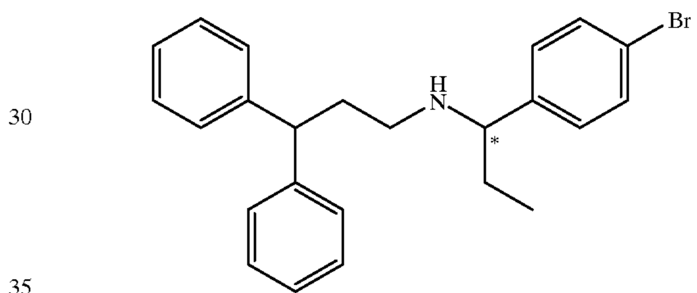
Compound 162
