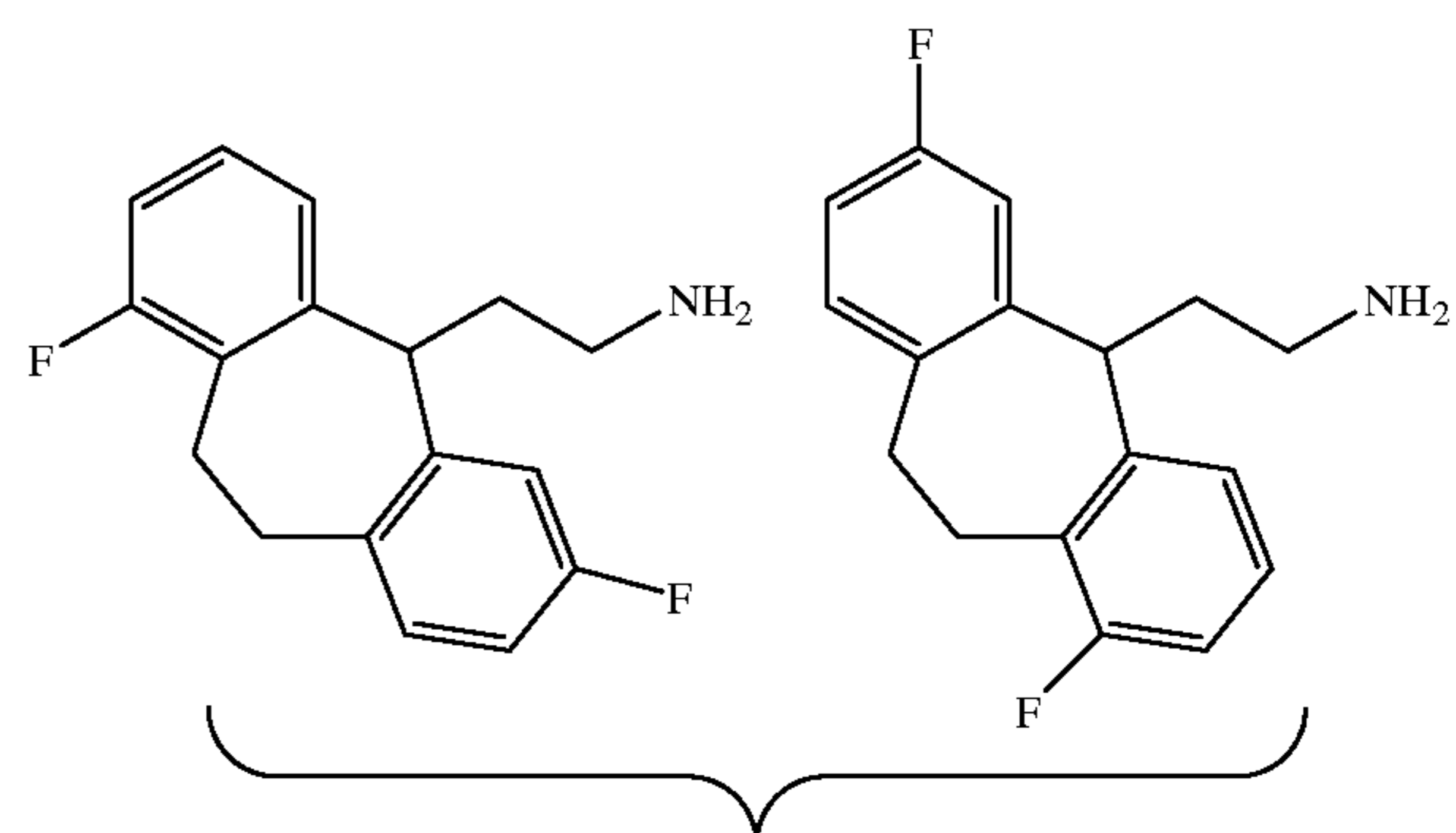
Compound 194 IC 50 (MK -801) = 339 nM
