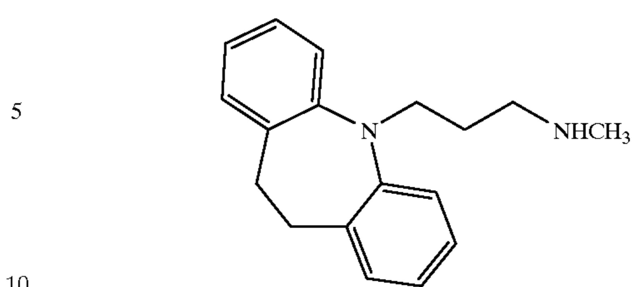
Desipramine
