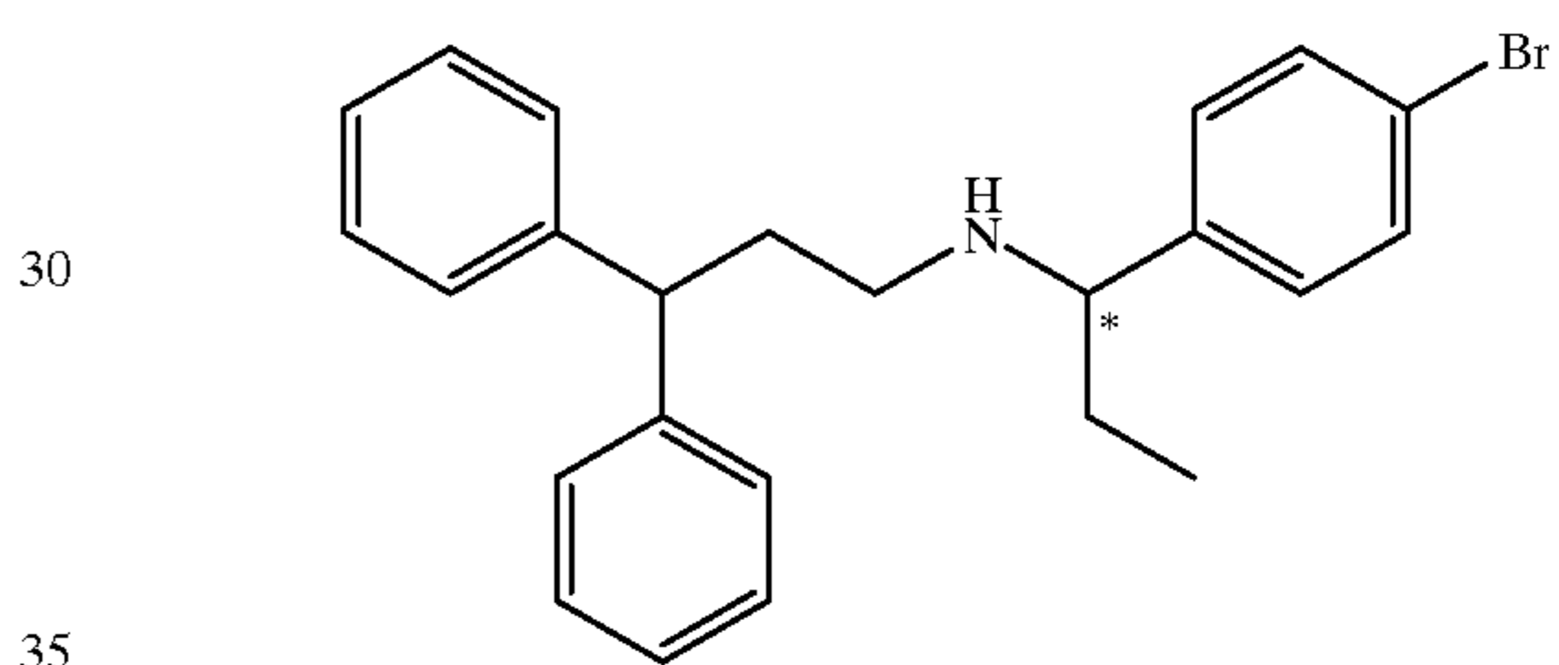
Compound 162
