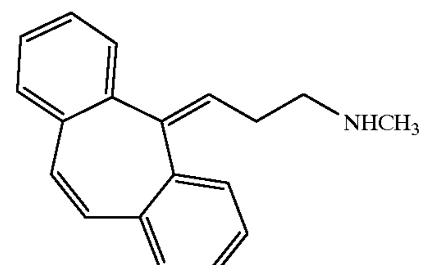
Nortriptyline
