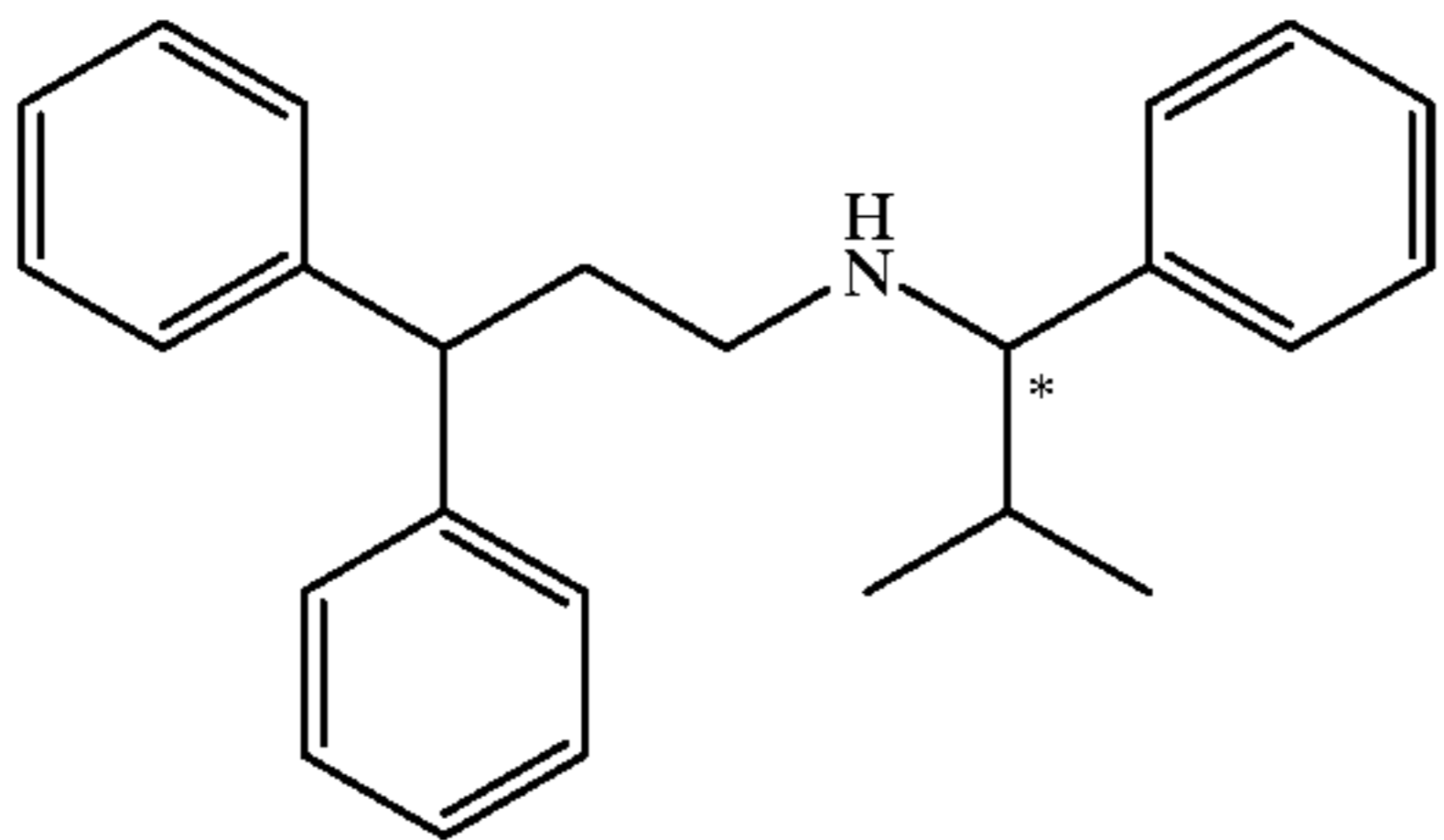
Compound 159
