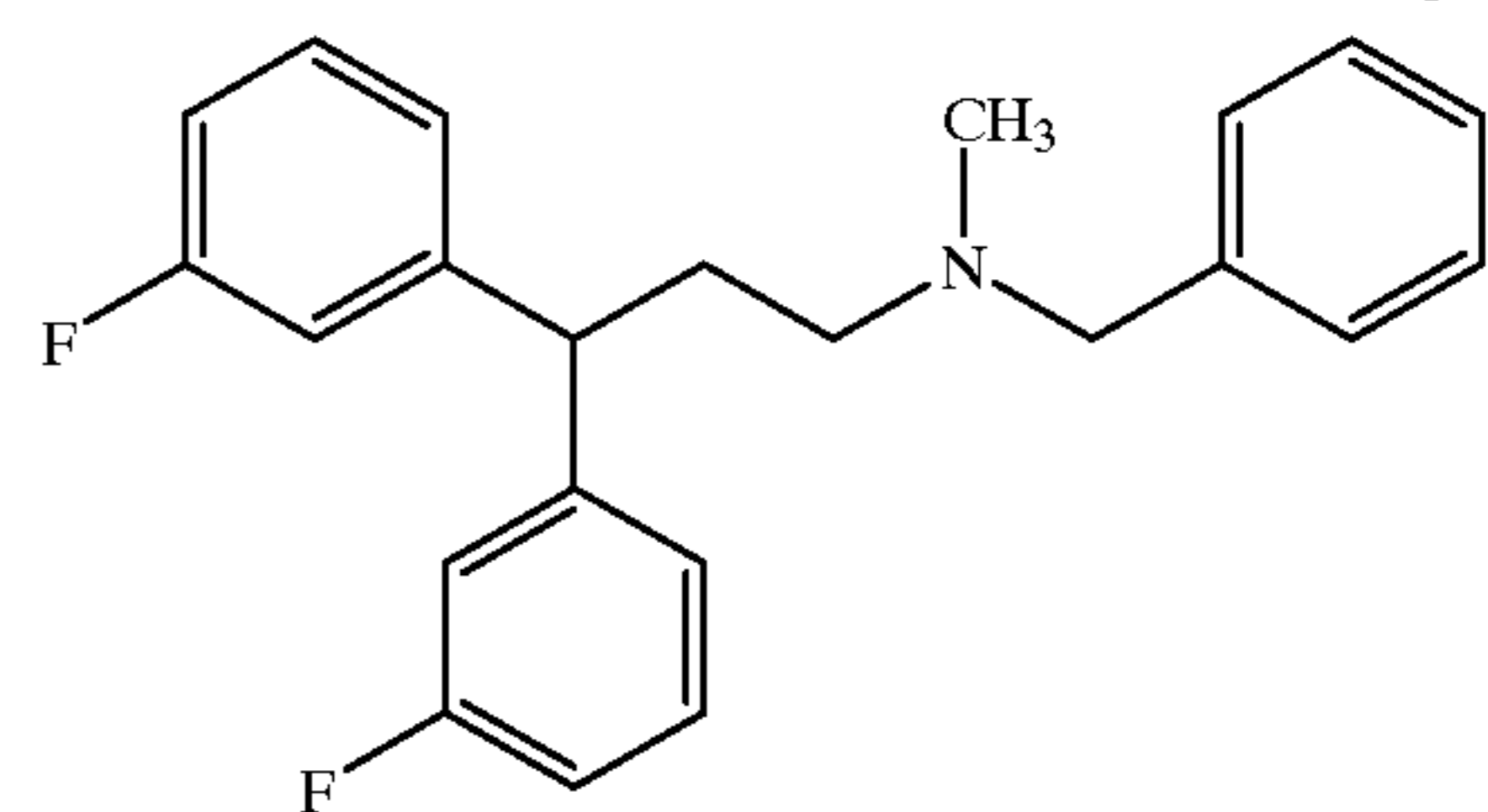
Compound 106
