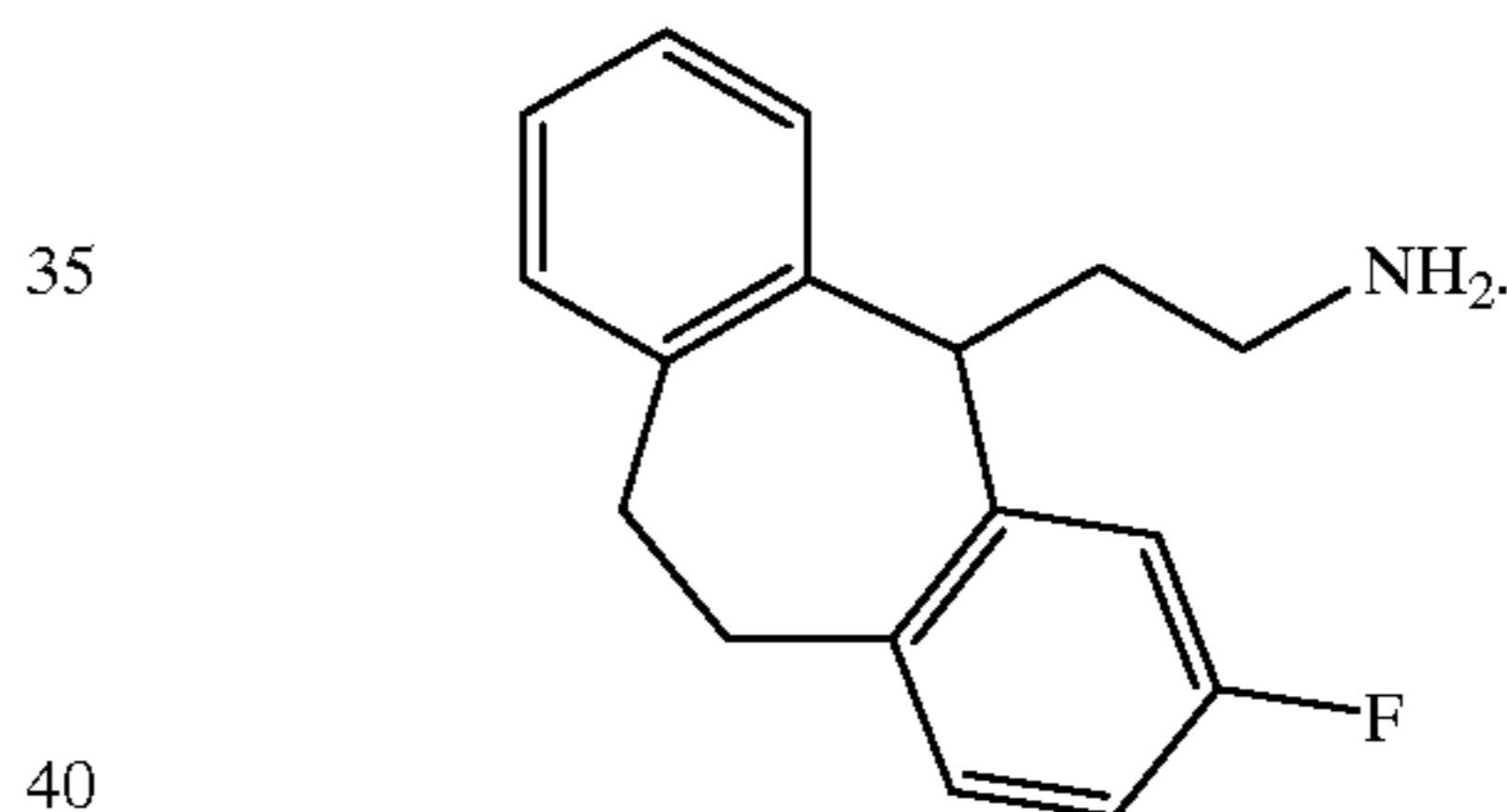
Compound 193
