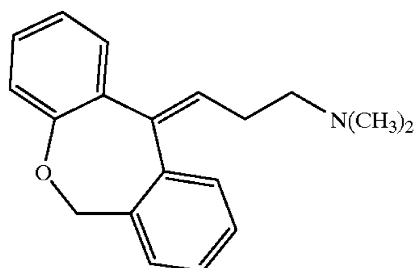
Doxepin
