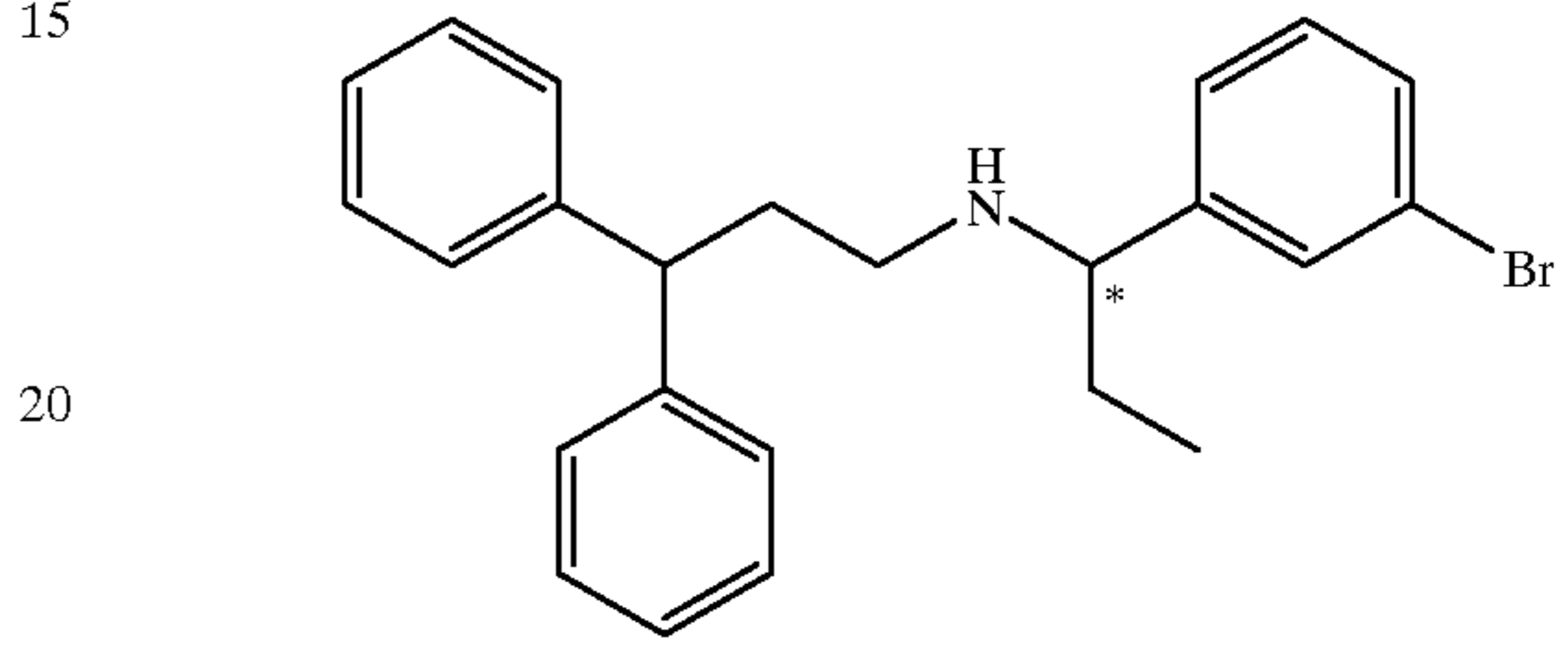
Compound 161
