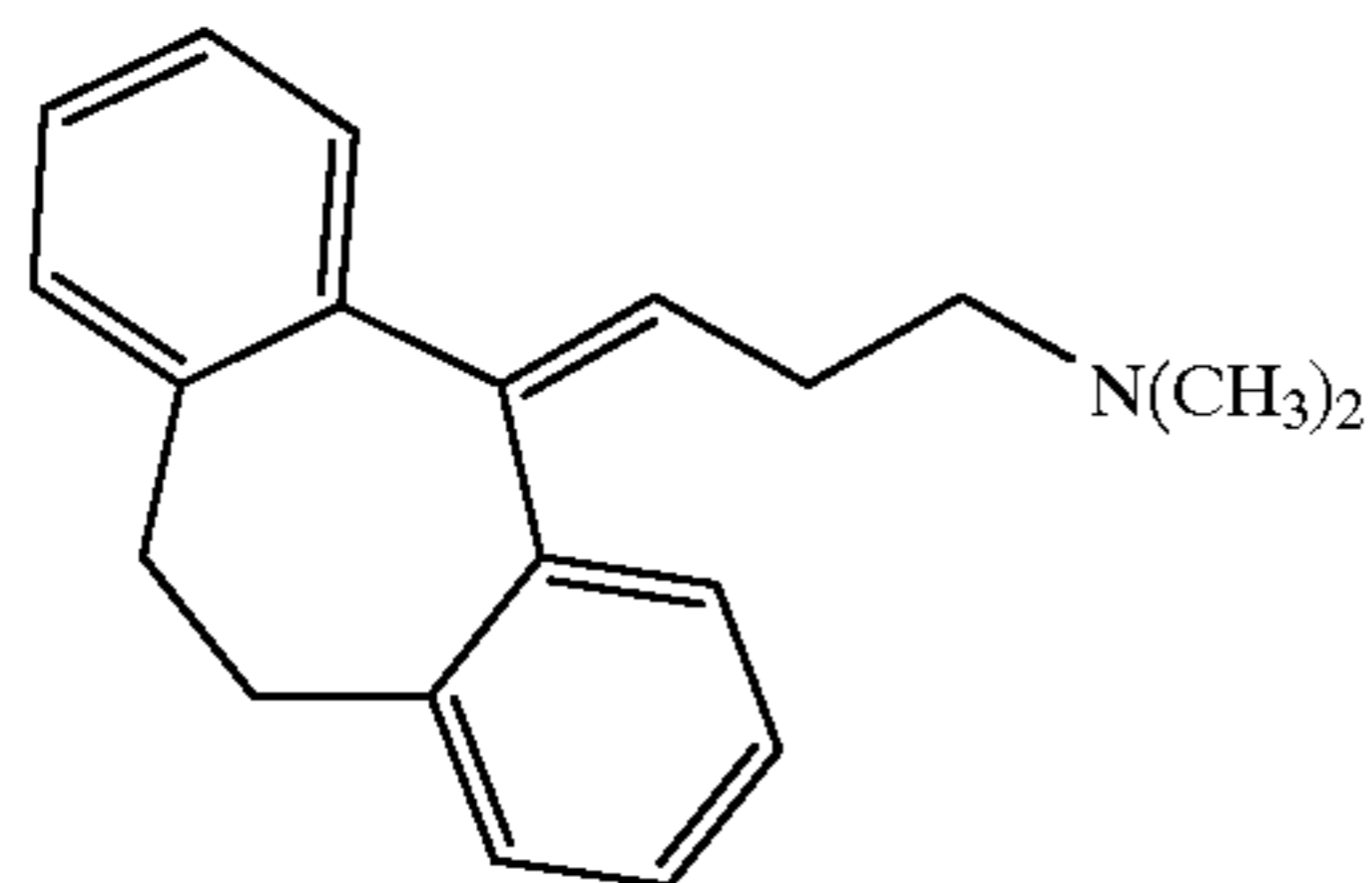
Amitriptyline
