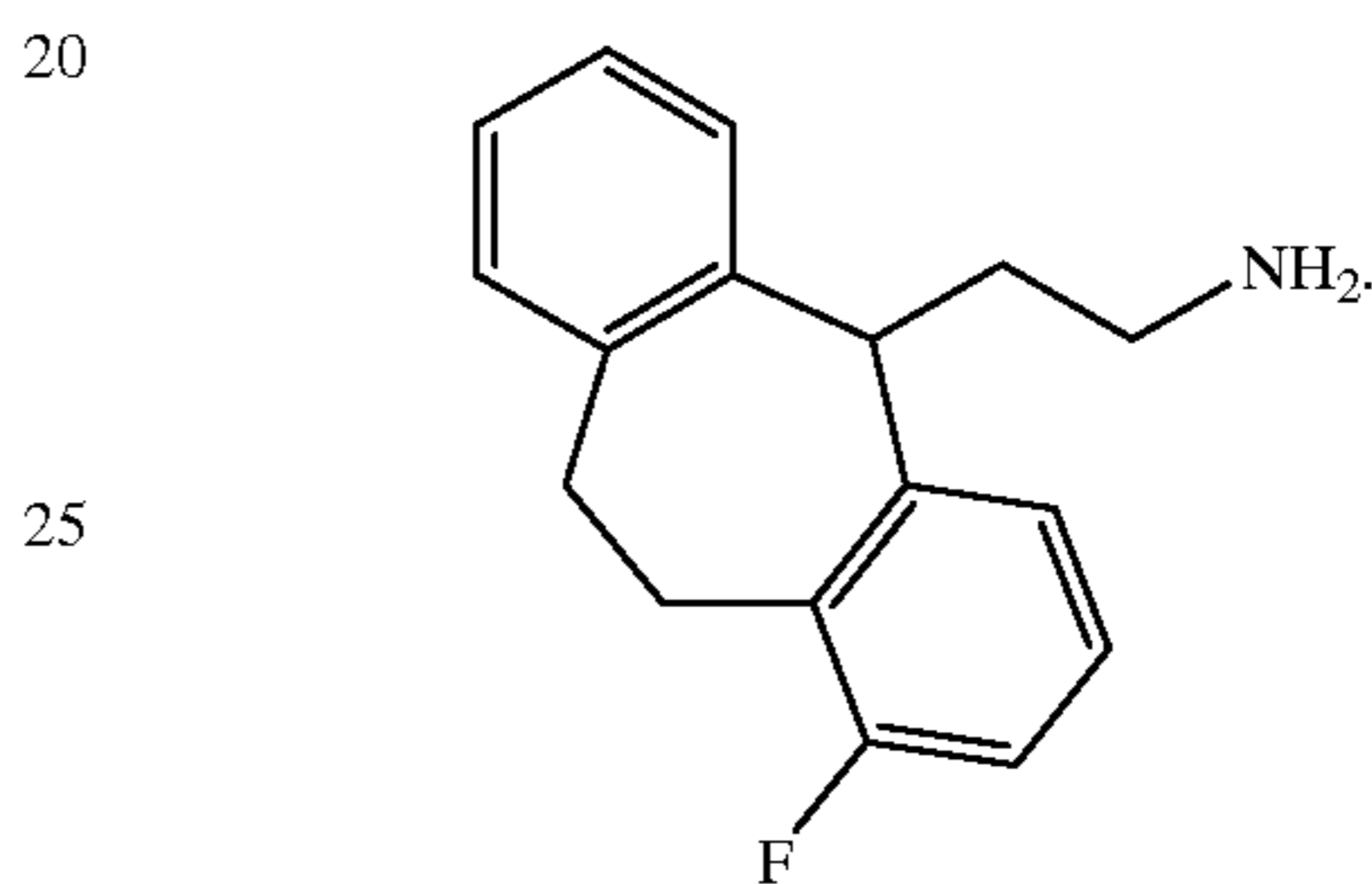
Compound 197
