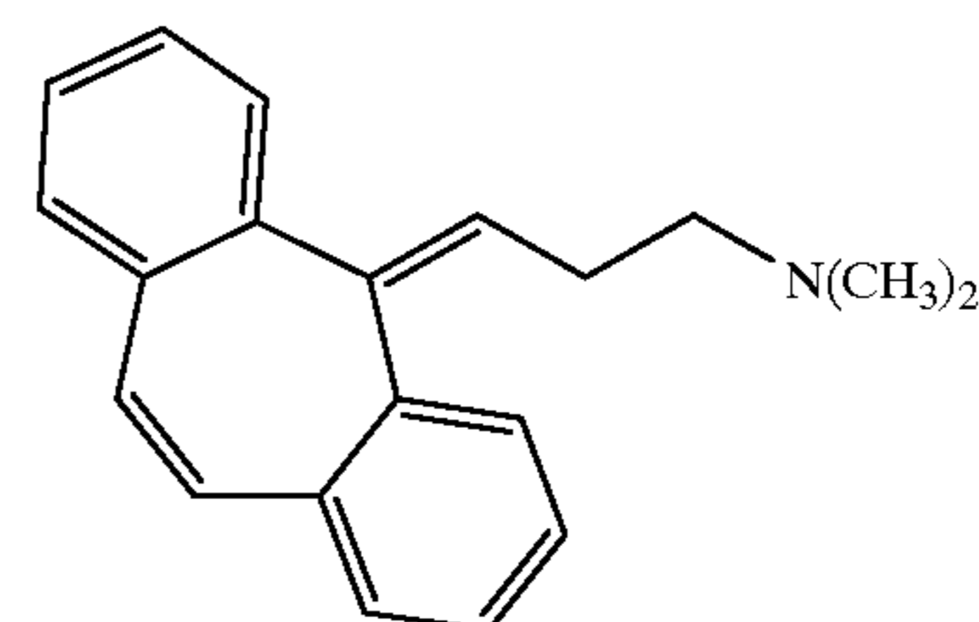
Cyclobenzaprine
