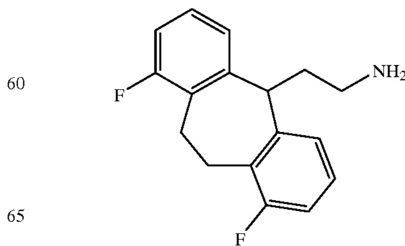
Compound 193
