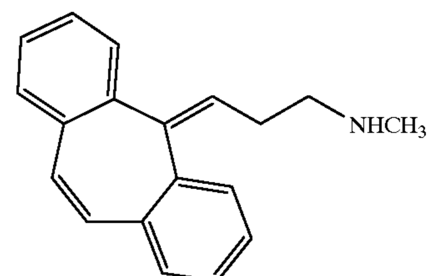
Nortriptyline
