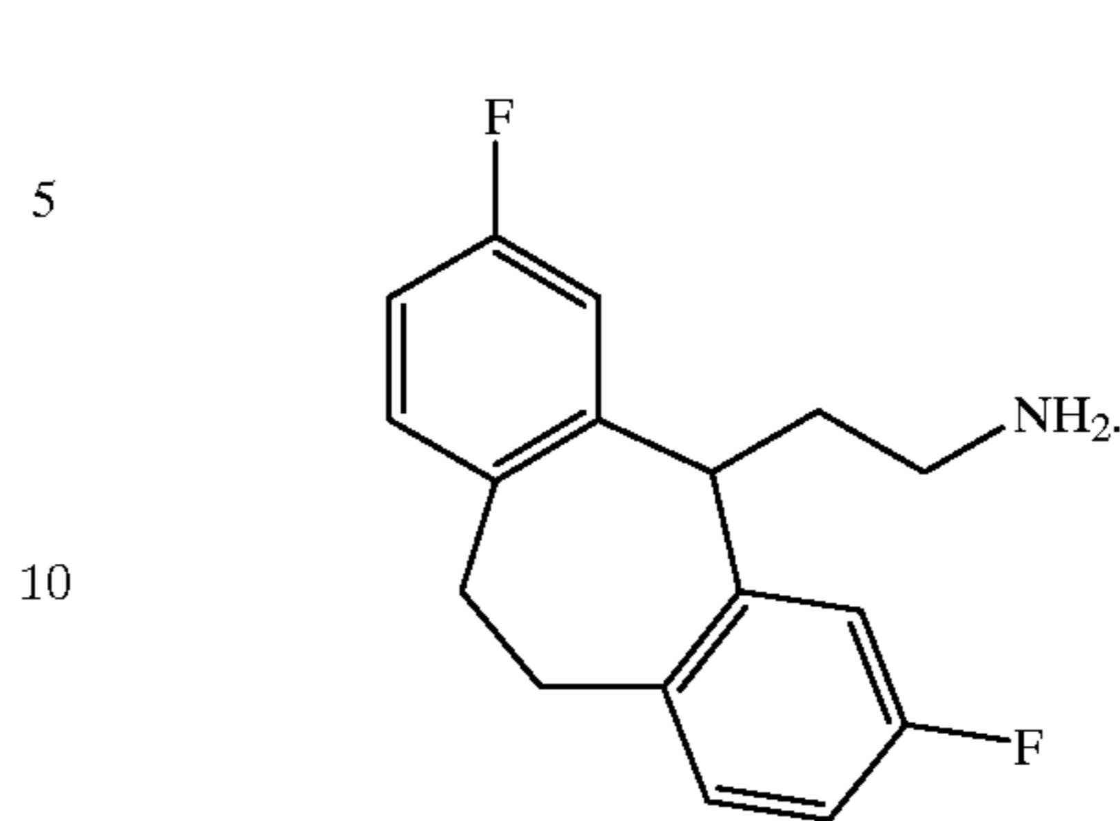
Compound 196
