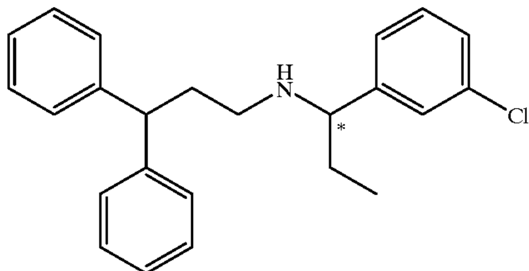
Compound 159
