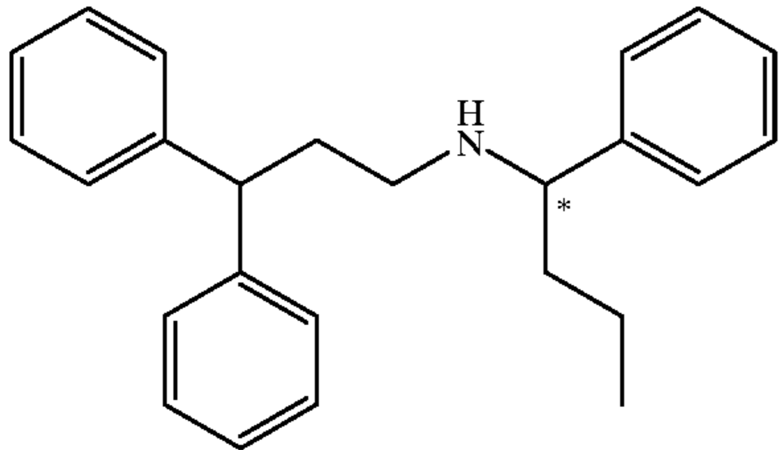
Compound 158
