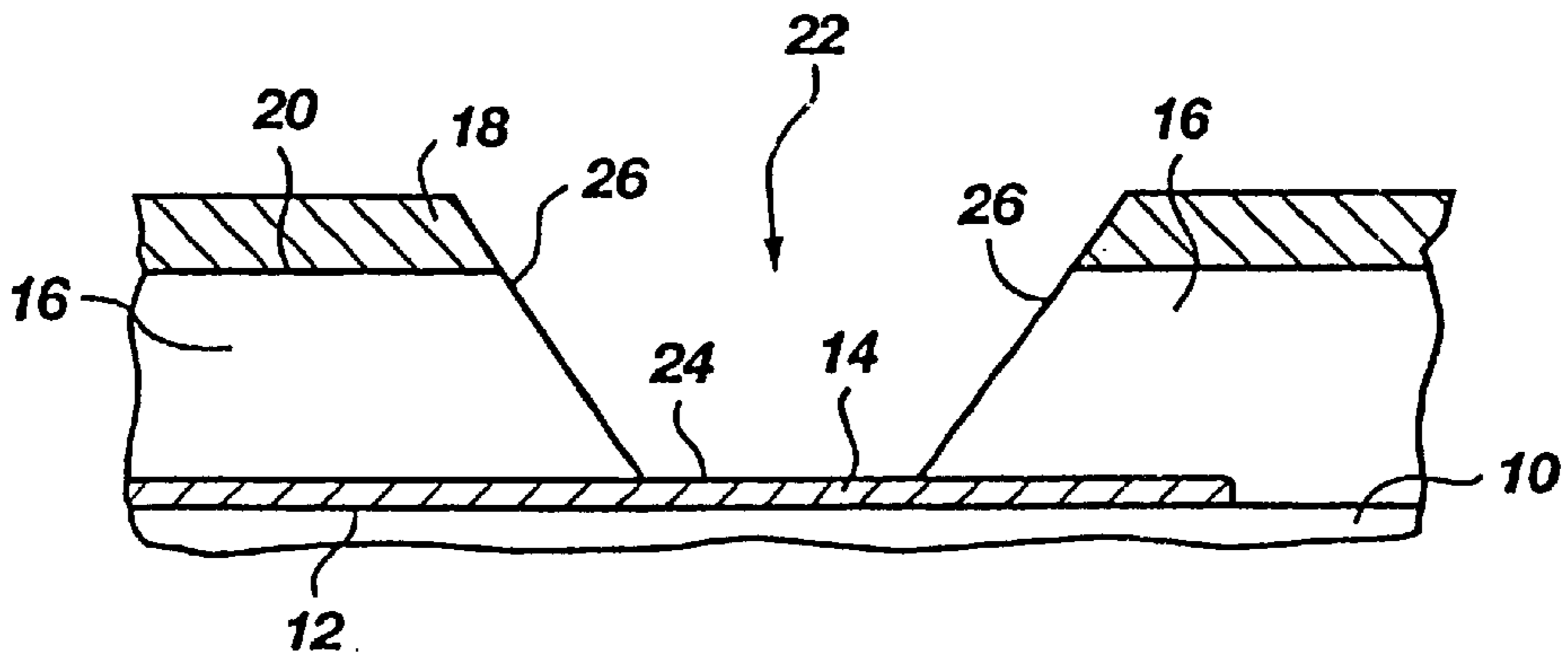
Fig. 1c (PRIOR ART)
