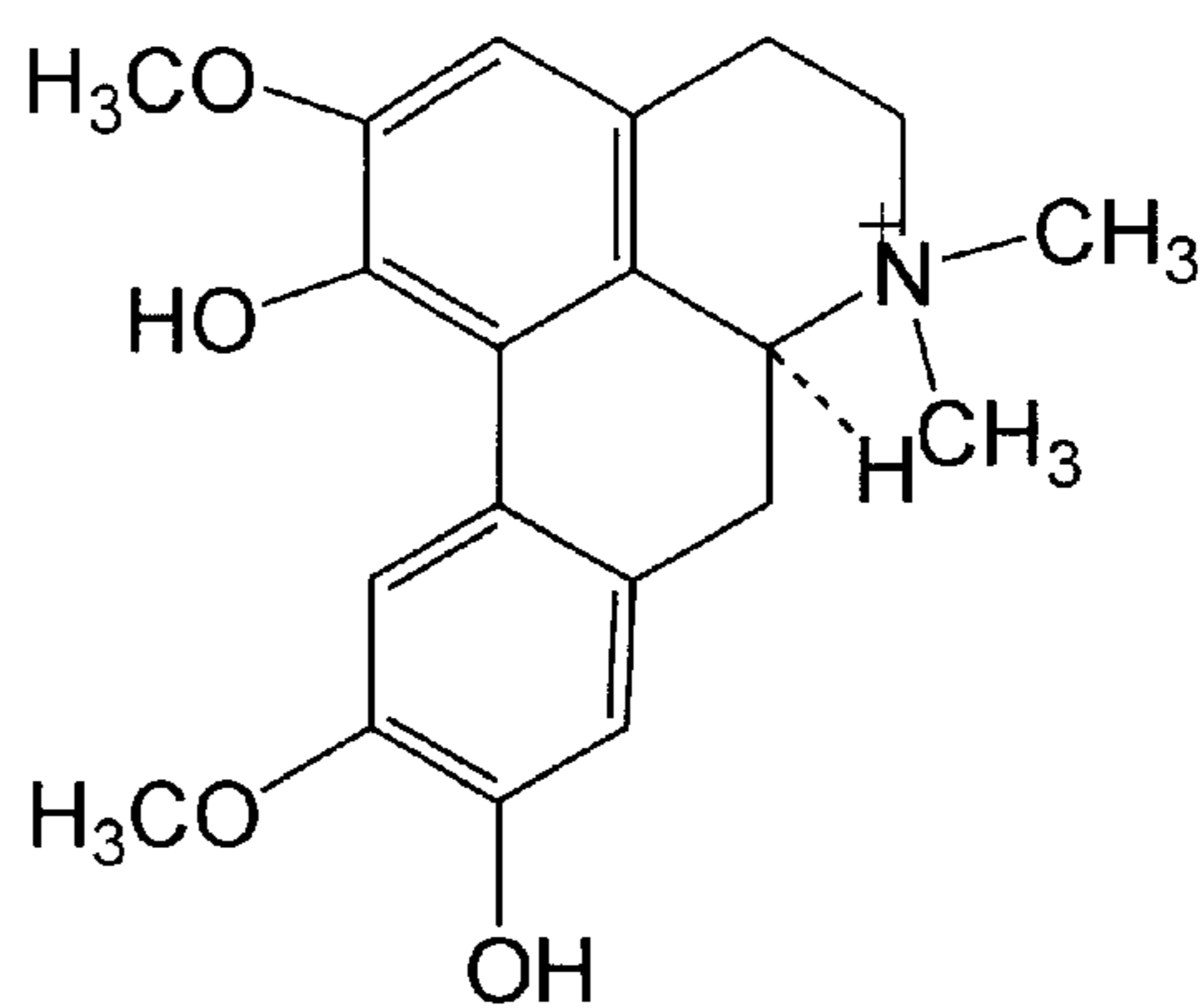
LAURIFOLINE
