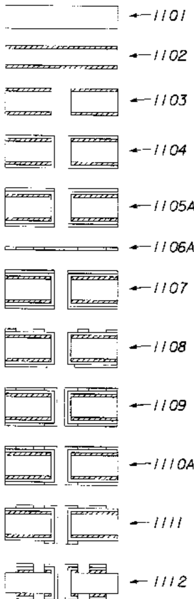
Conventional Subtractive Process of PWB Fabrication
