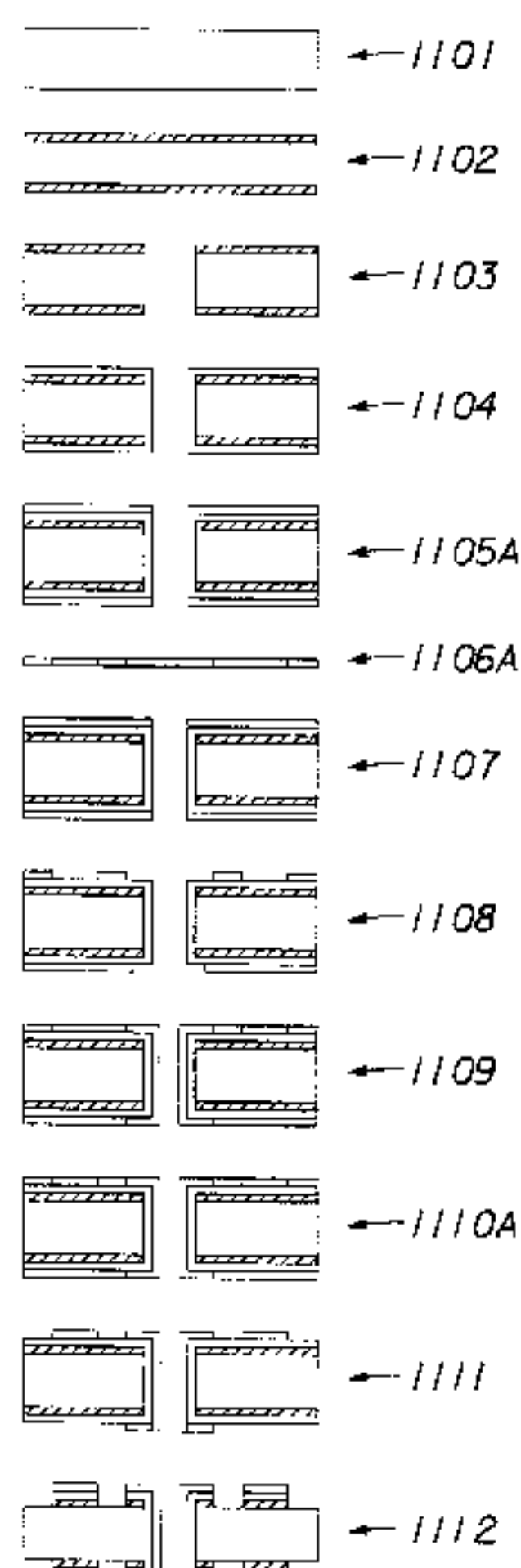
Conventional Subtractive Process of PWB Fabrication
