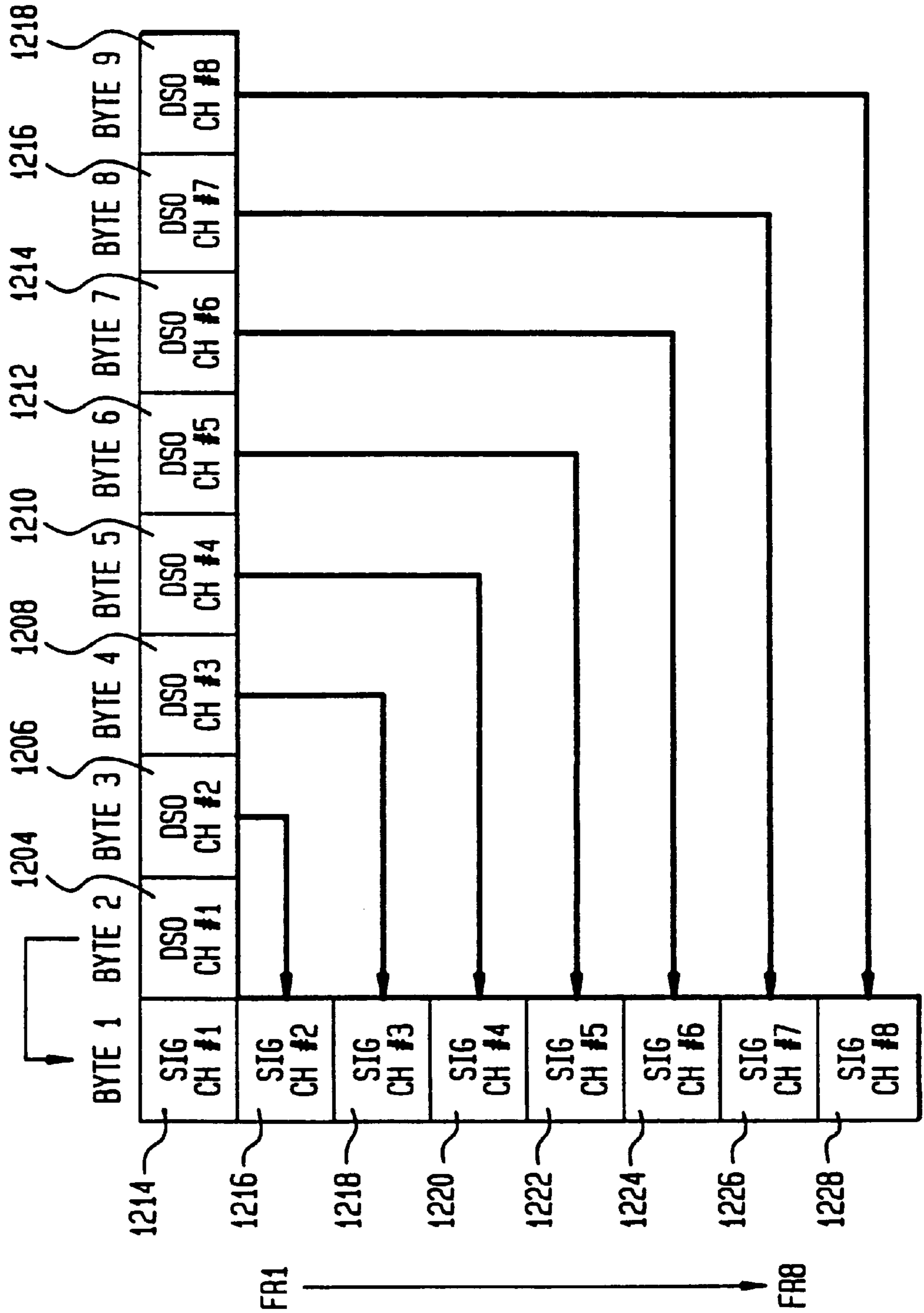
BASIC TDM BLOCK DSO MAPPING
