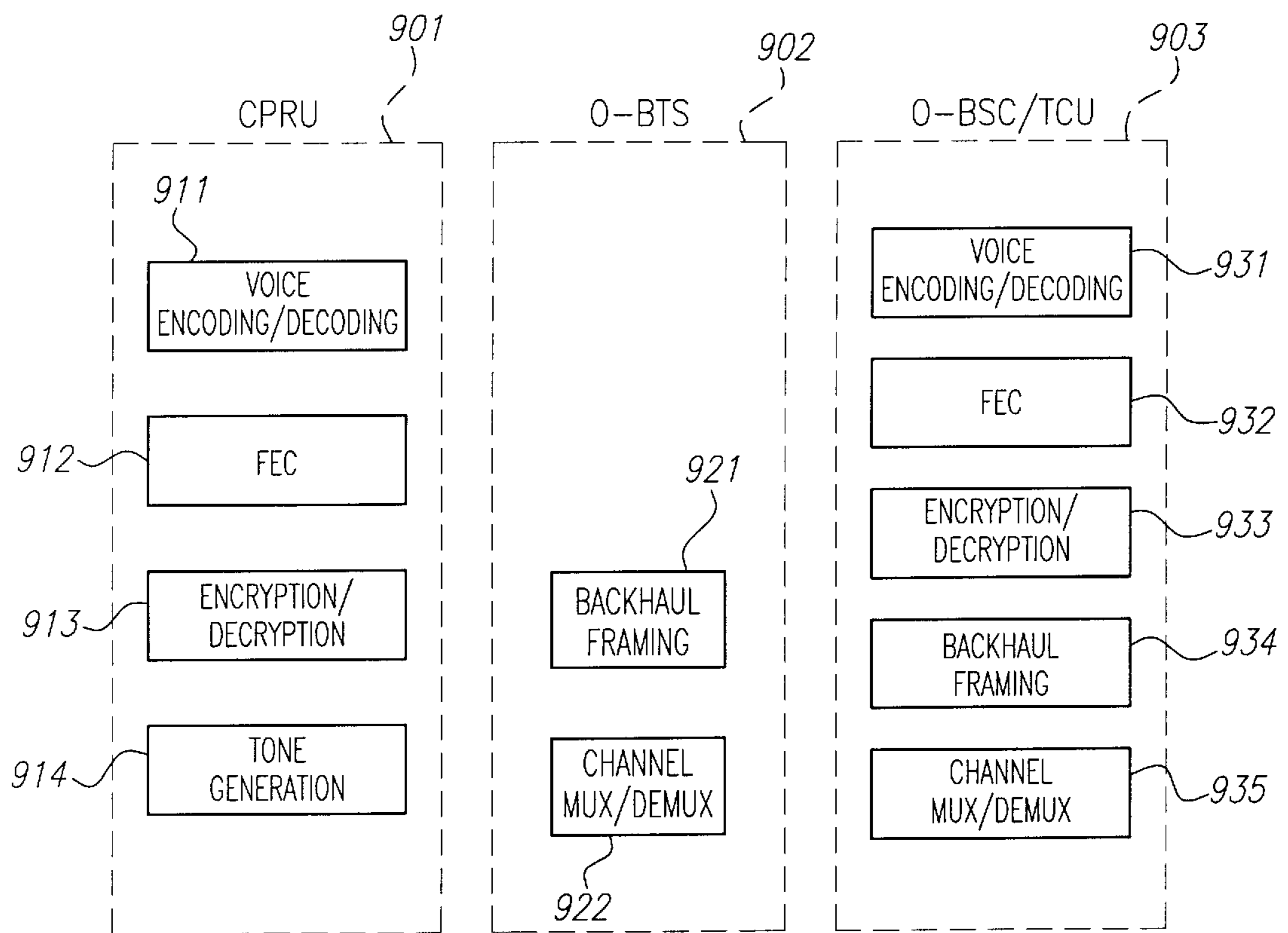
BEARER PATH FUNCTIONS
