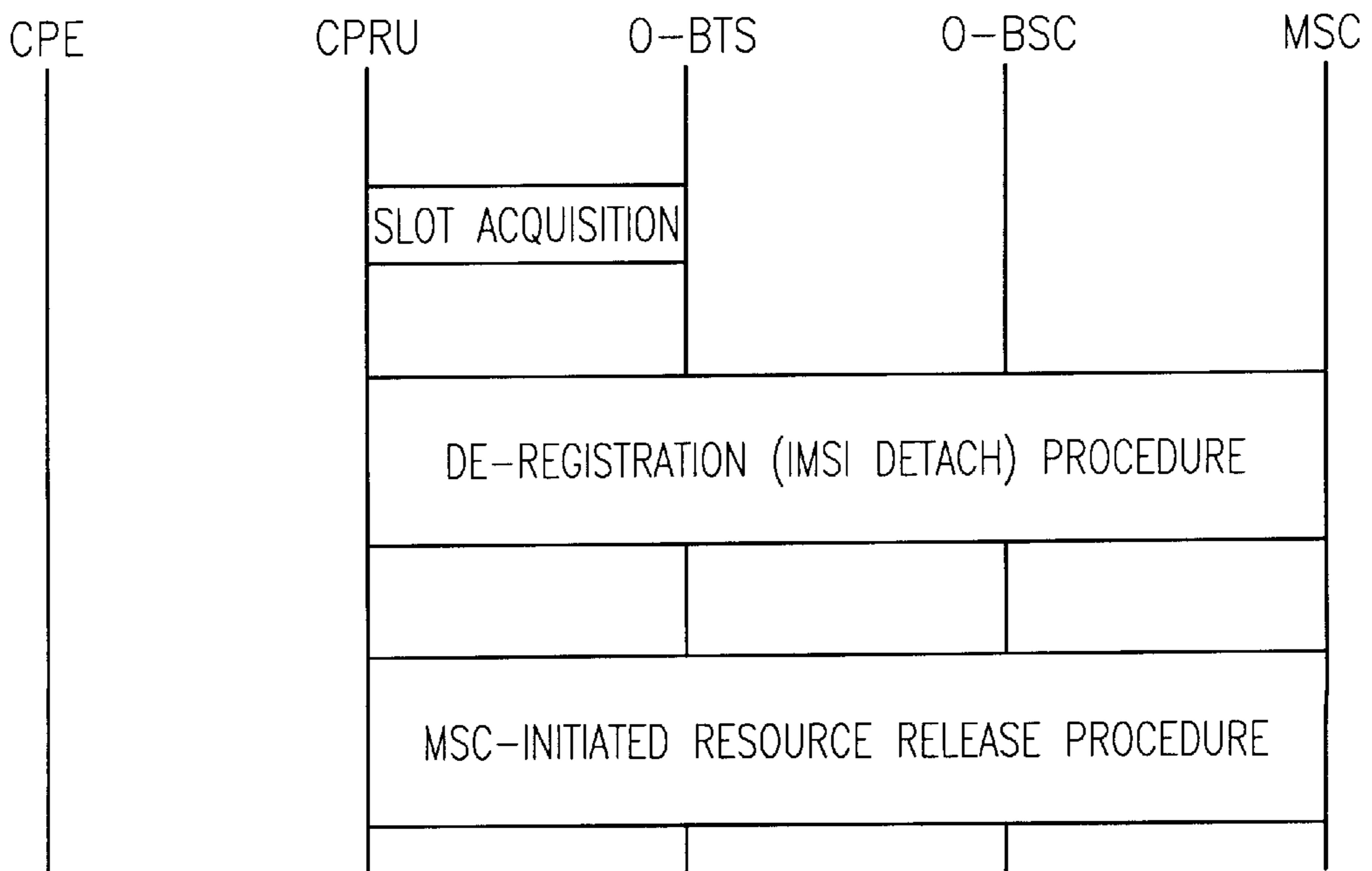
DE-REGISTRATION
