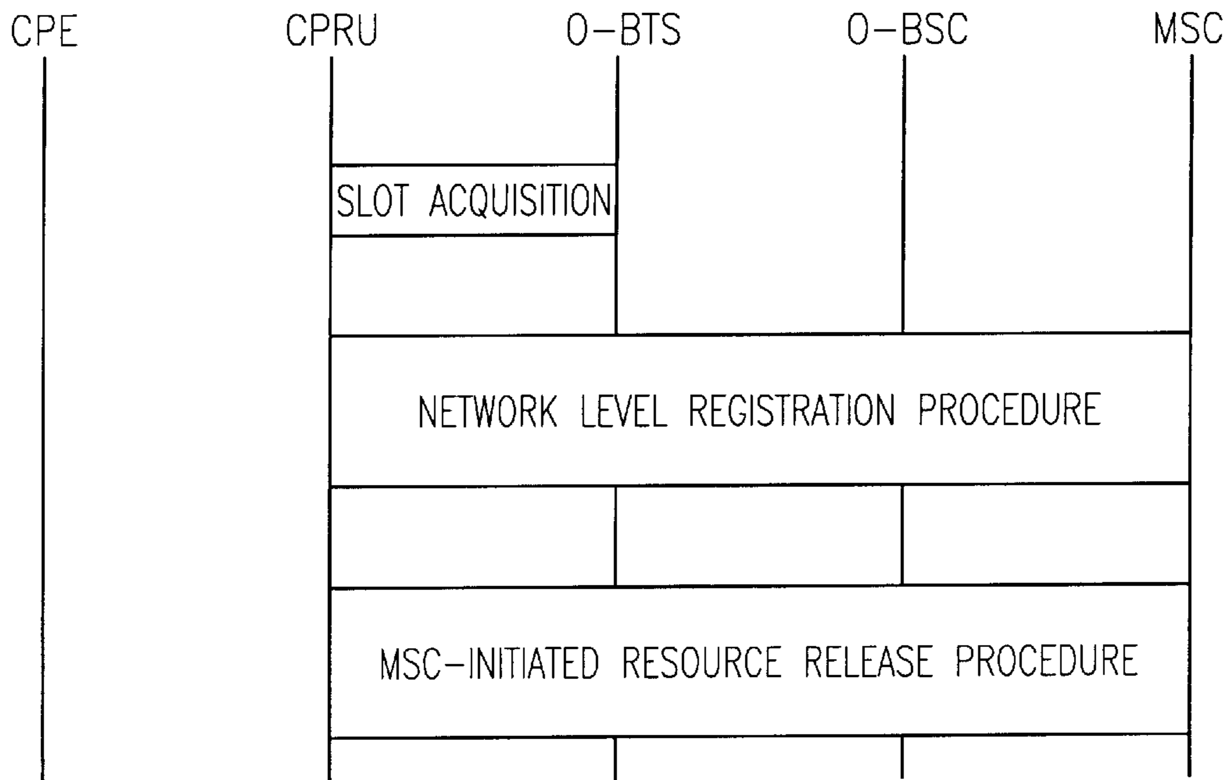
NETWORK-LEVEL REGISTRATION
