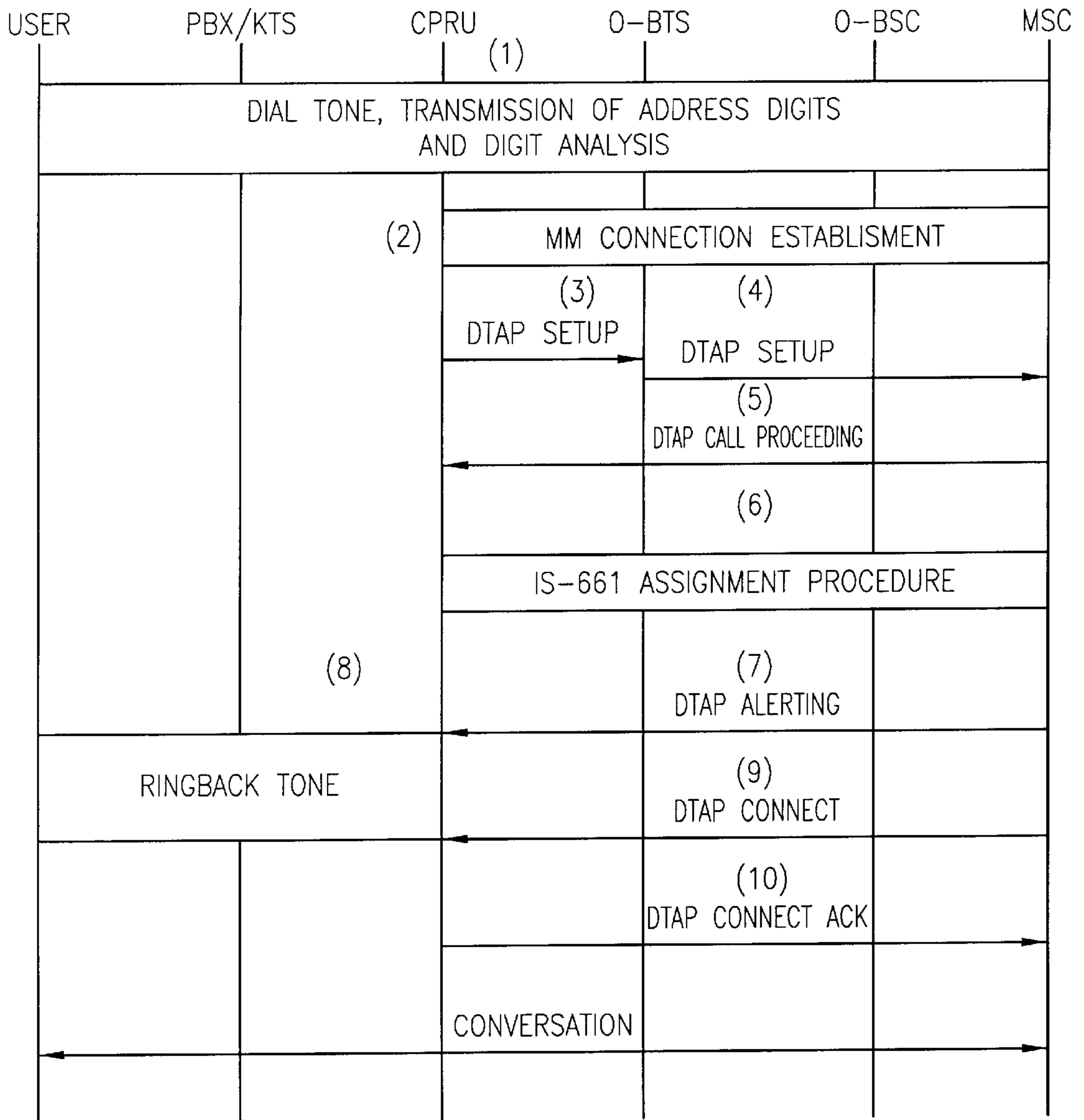
SUCCESSFUL OUTGOING CALL SETUP (NON-PSTN INTERWORKING)
