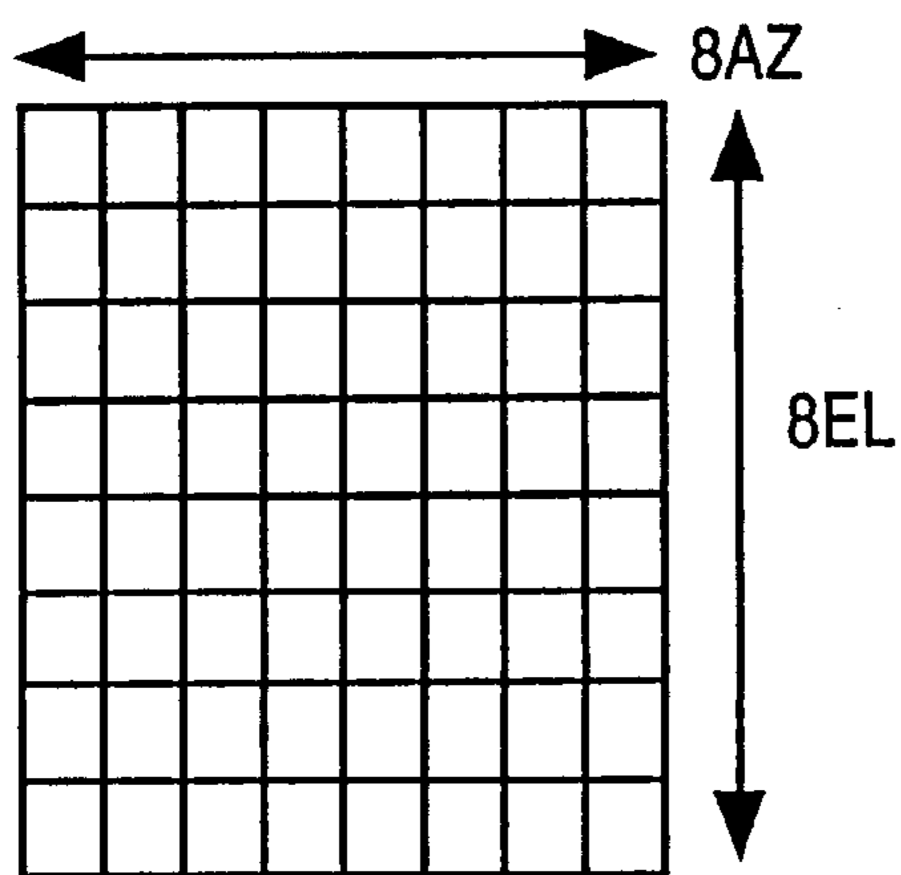
NORMAL BEAMFORMER
