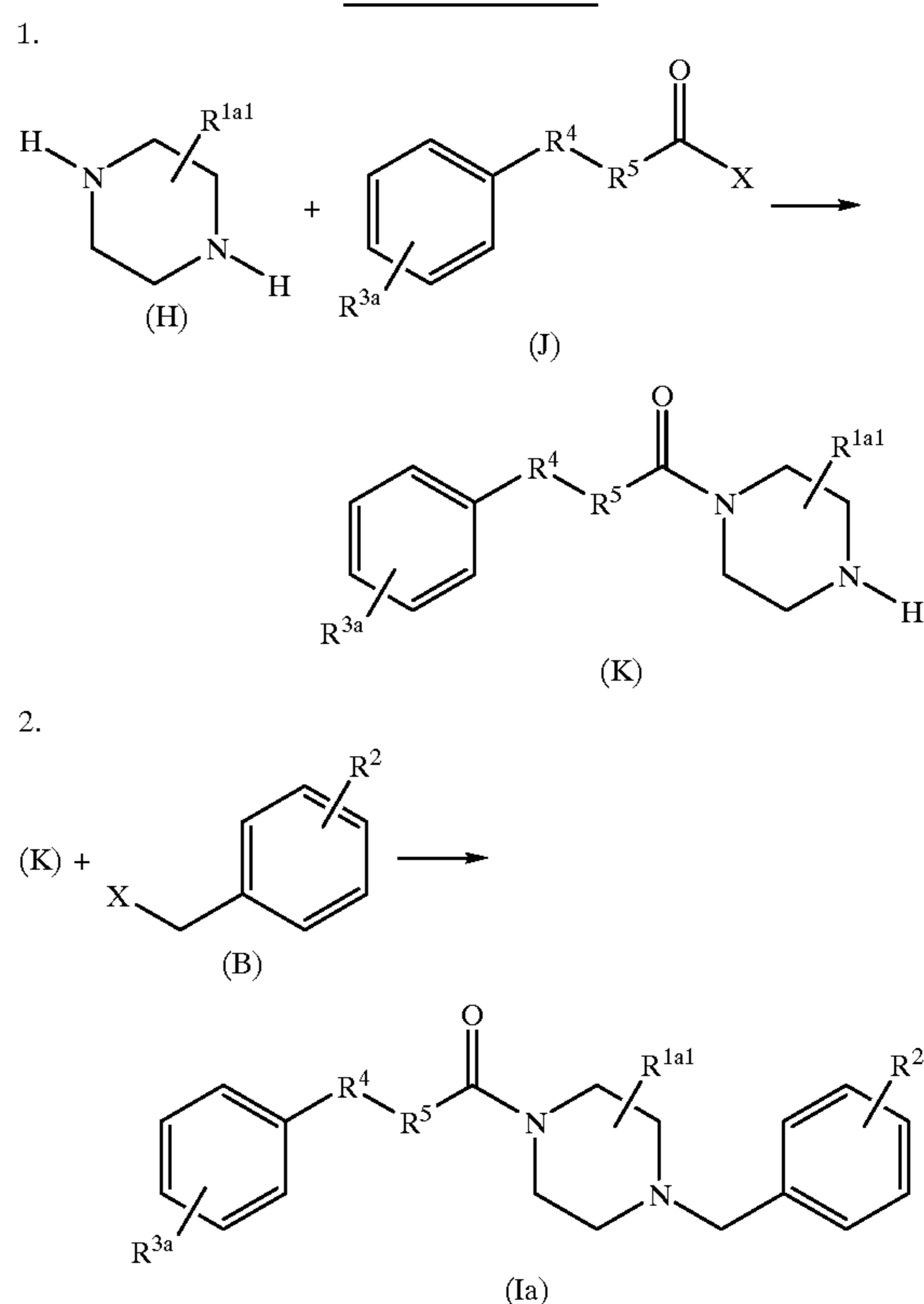
Reaction Scheme 3
