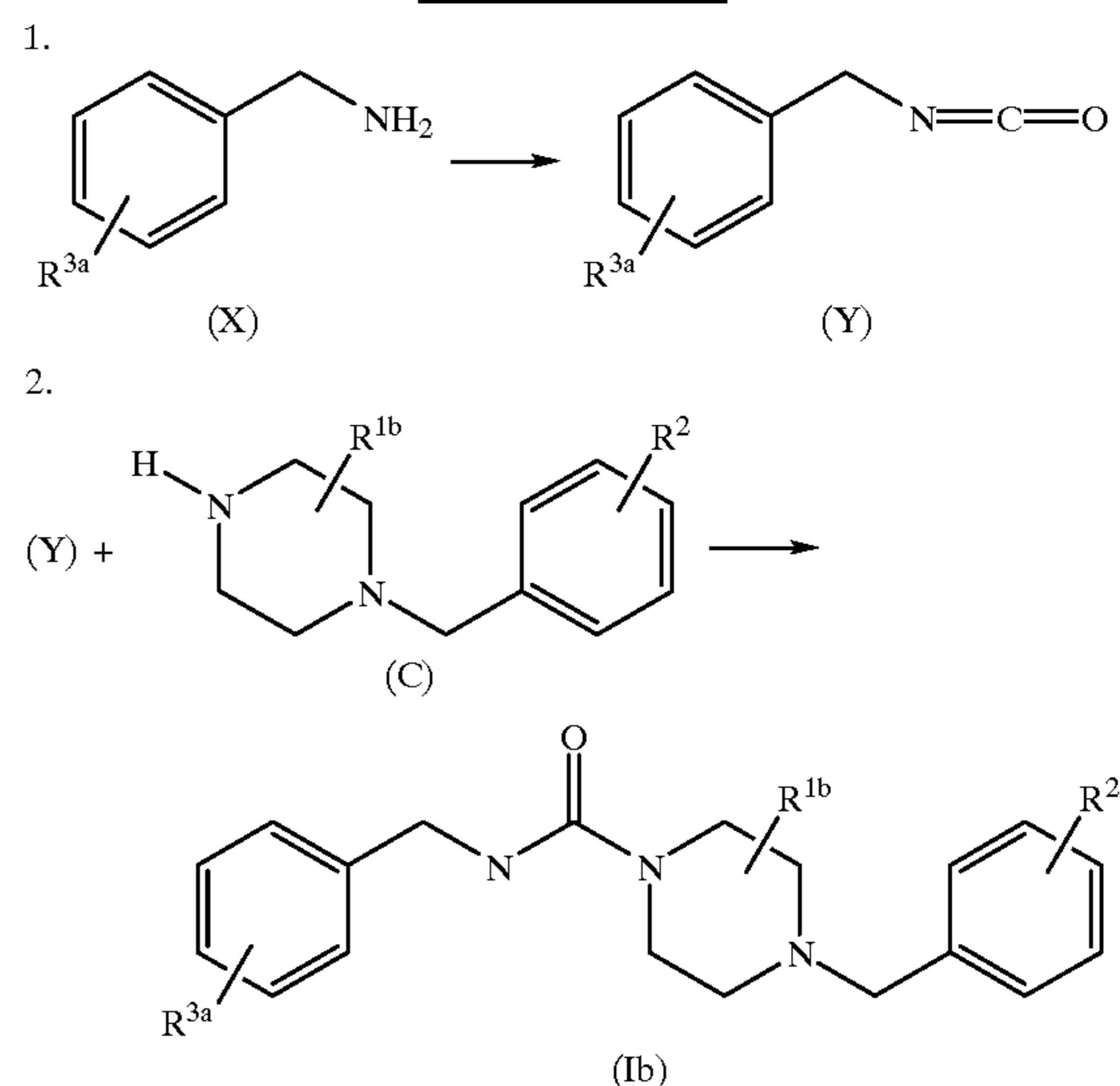
Reaction Scheme 7
