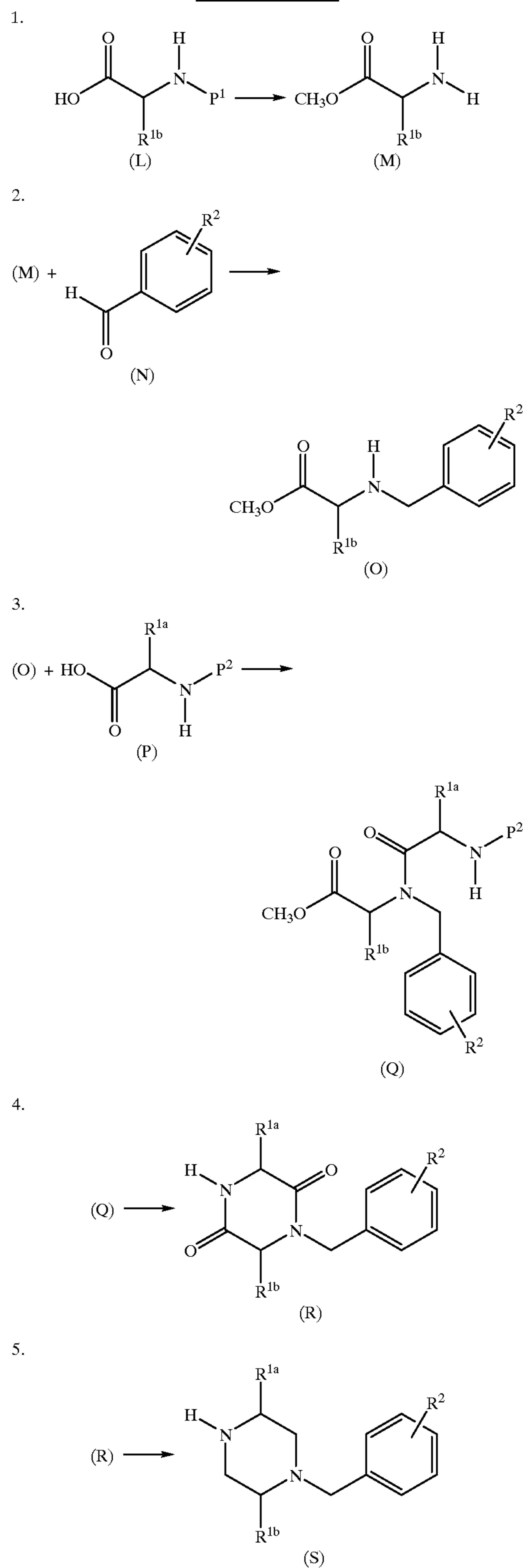
Reaction Scheme 4
