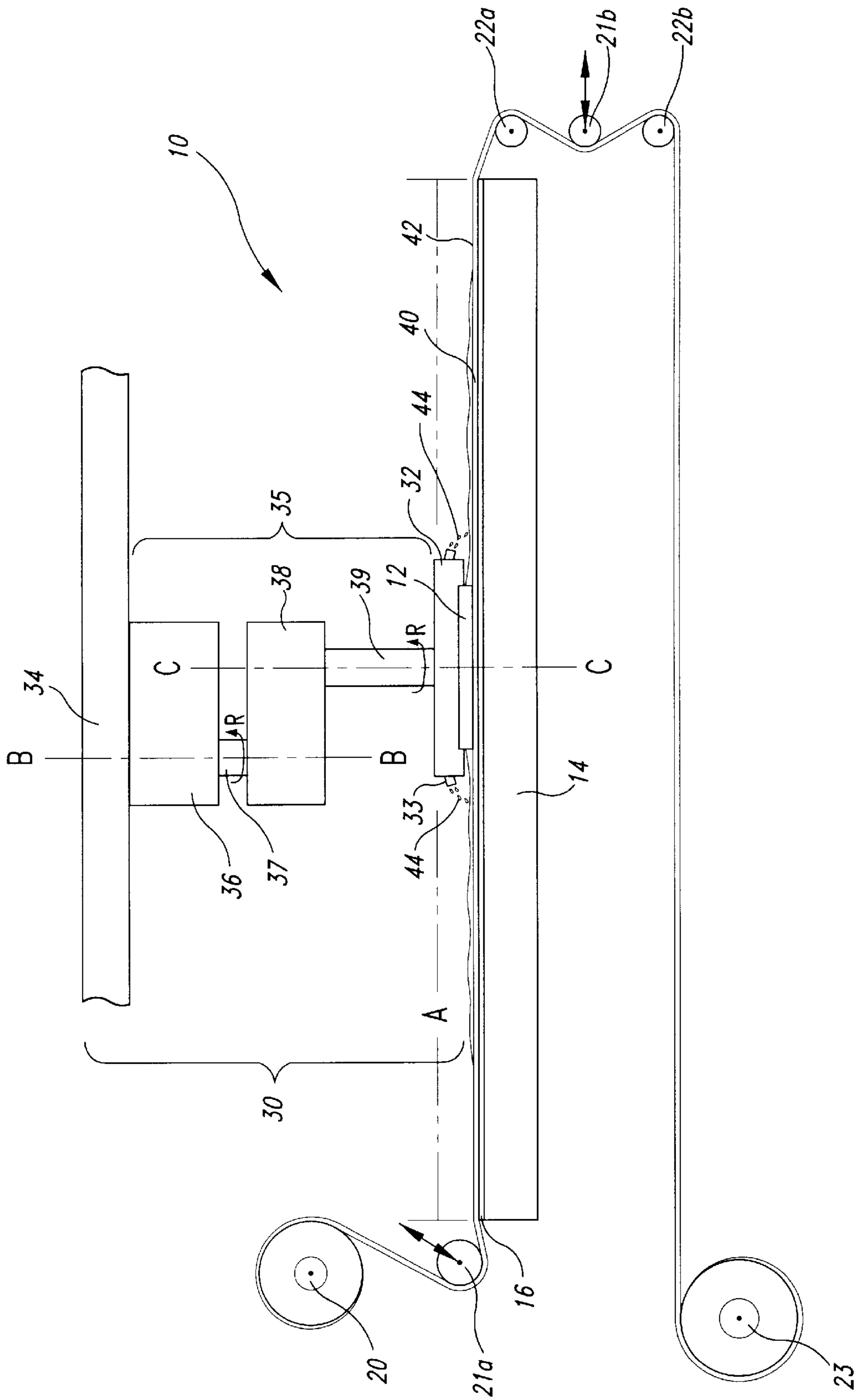
Fig. 1 (PRIOR ART)
