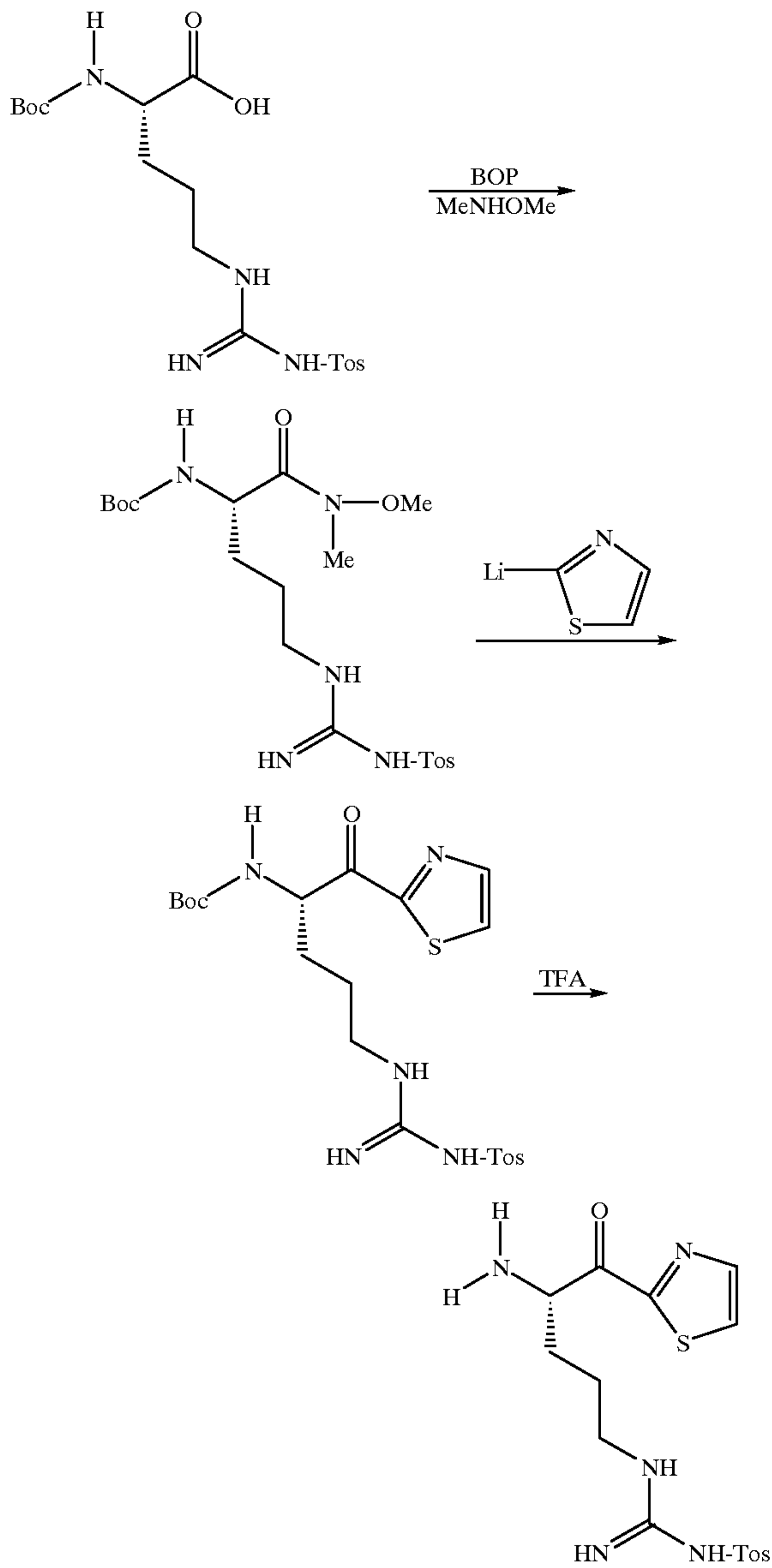
Scheme I
