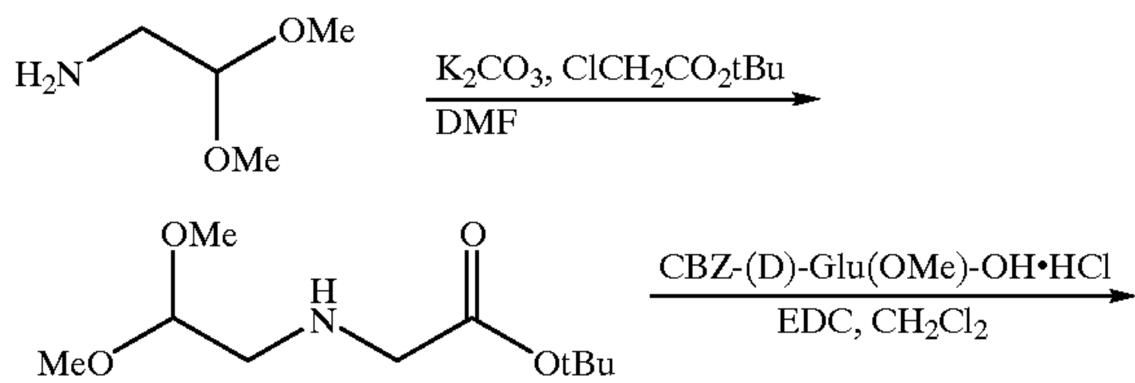
Scheme II
