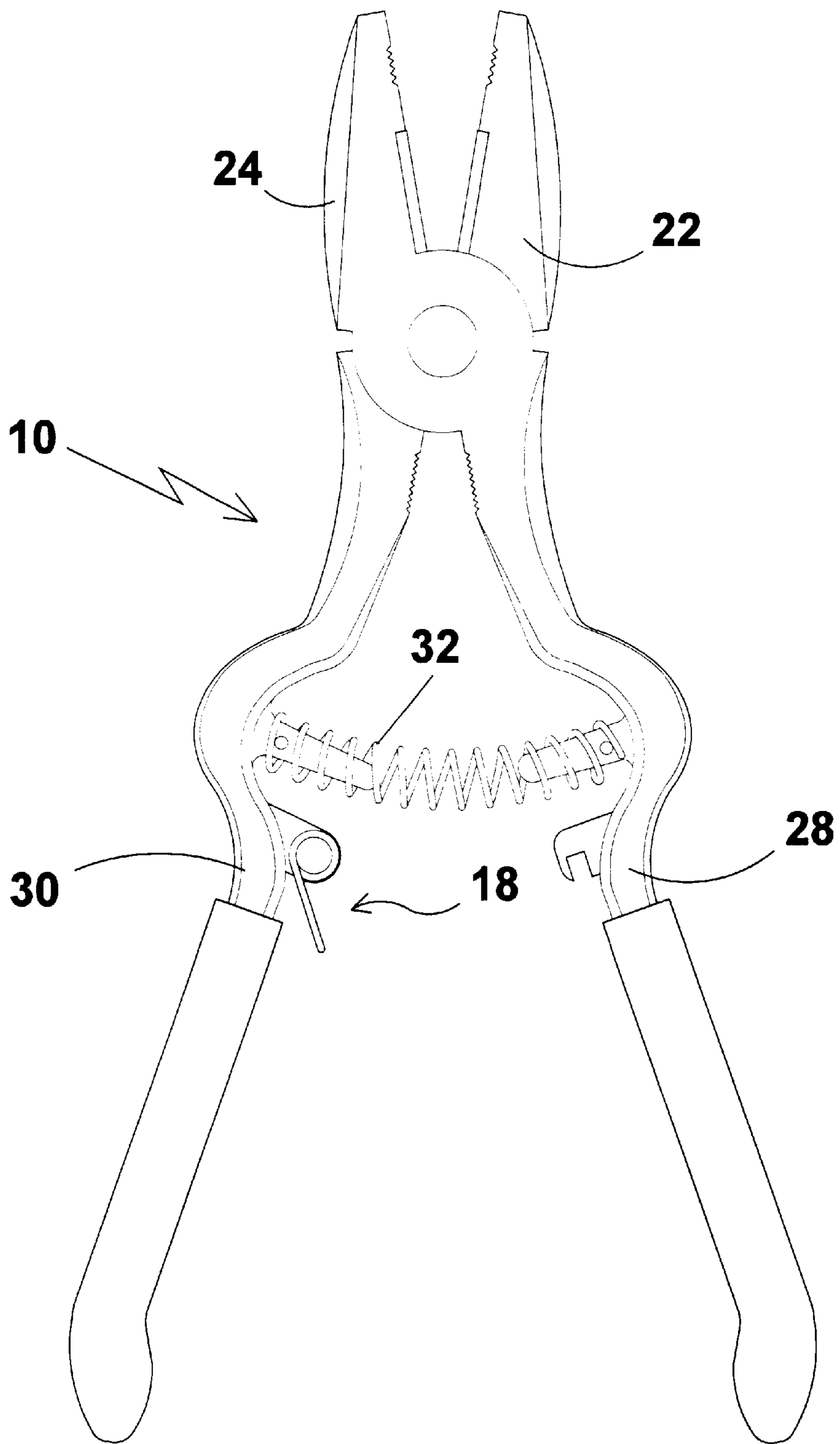
ELECTRICIAN'S PLIERS-OPENED
