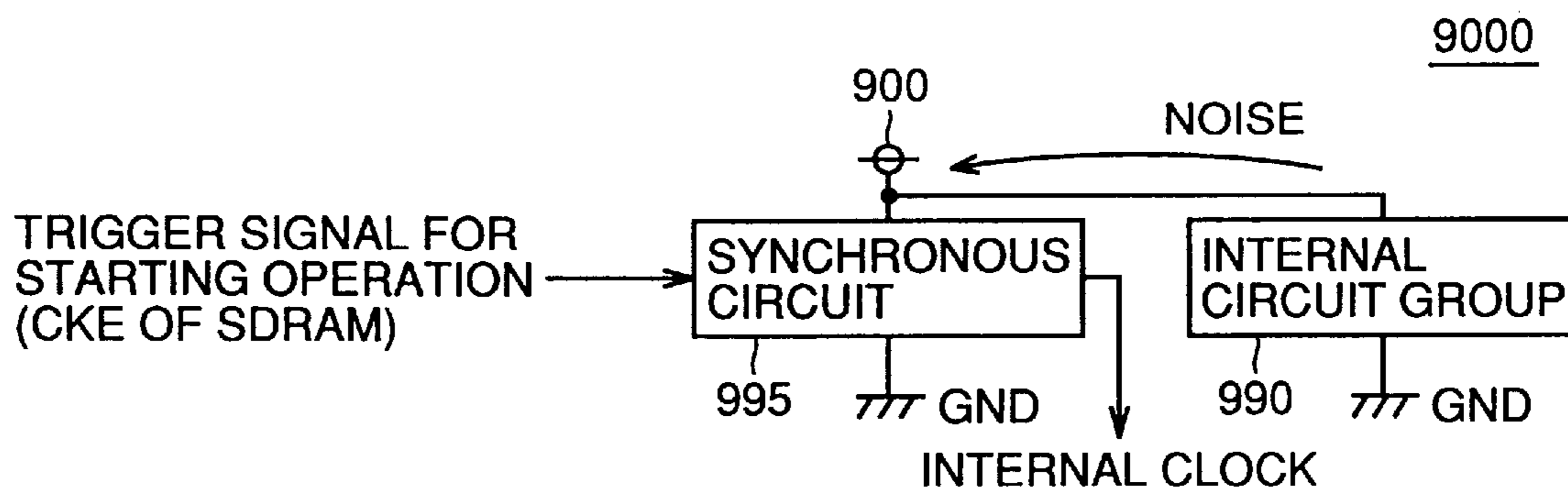
FIG.20 PRIOR ART
