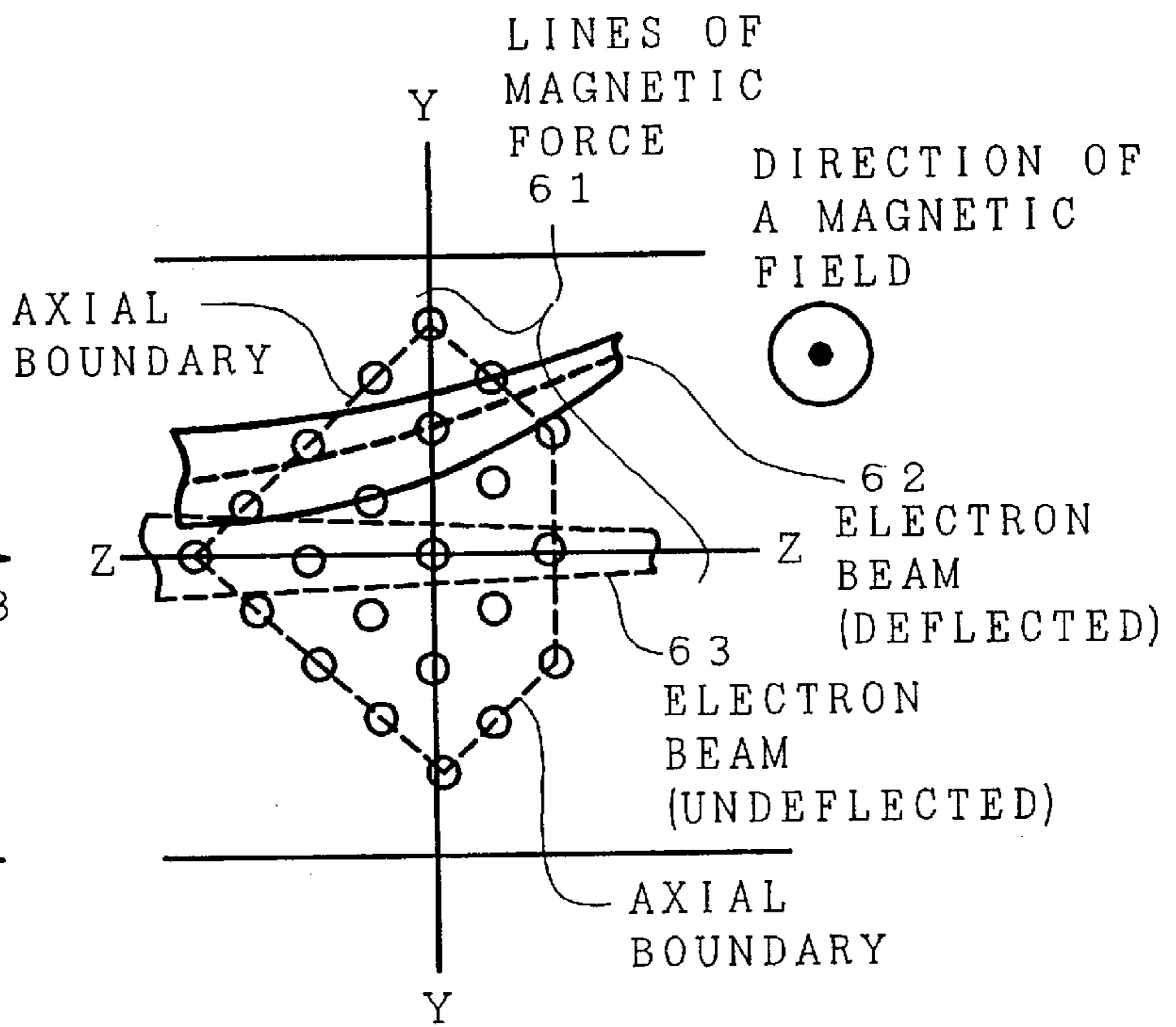
DIRECTION OF AN ELECTRON BEAM TRAVEL
