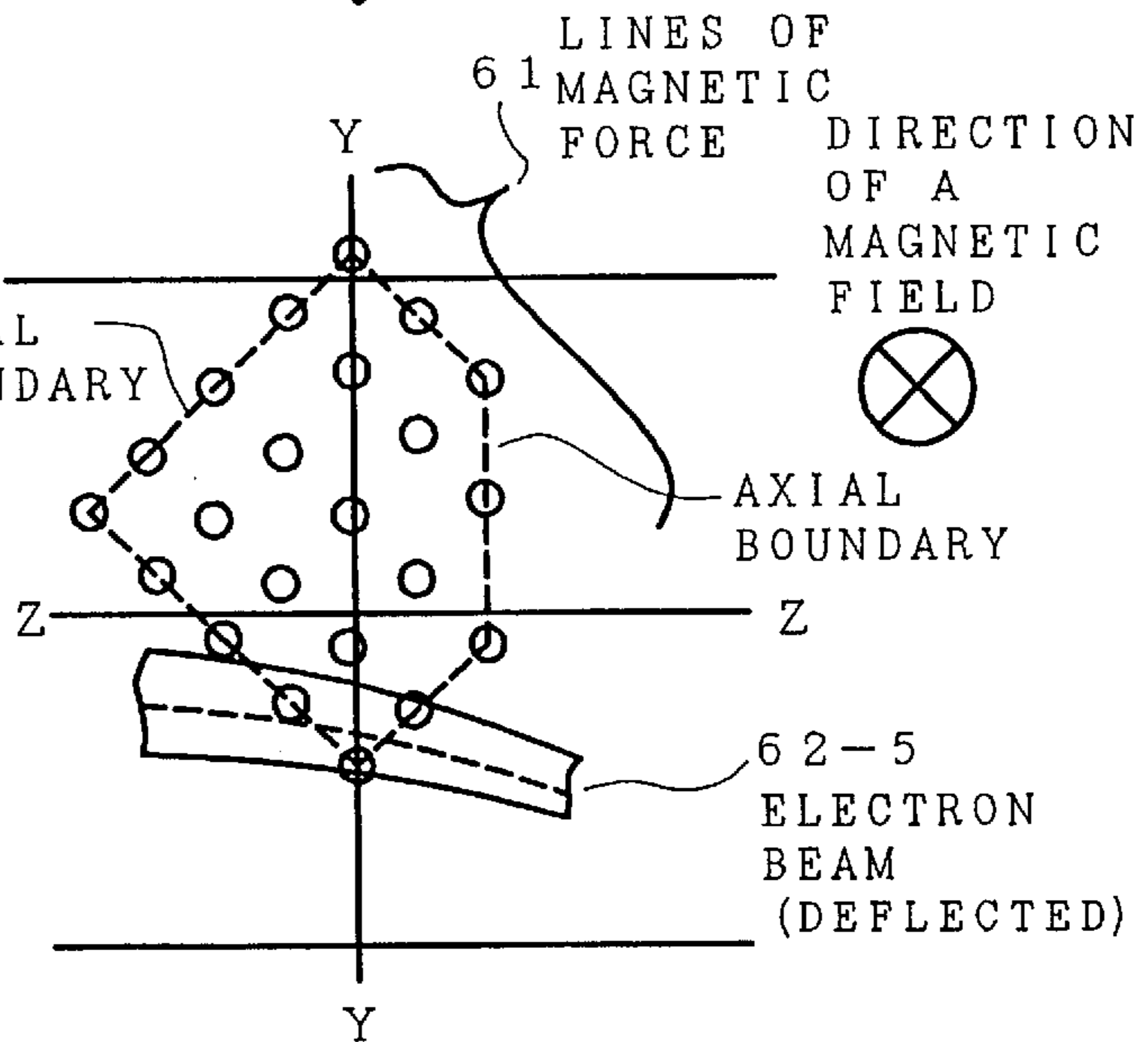
DIRECTION OF AN ELECTRON BEAM TRAVEL
