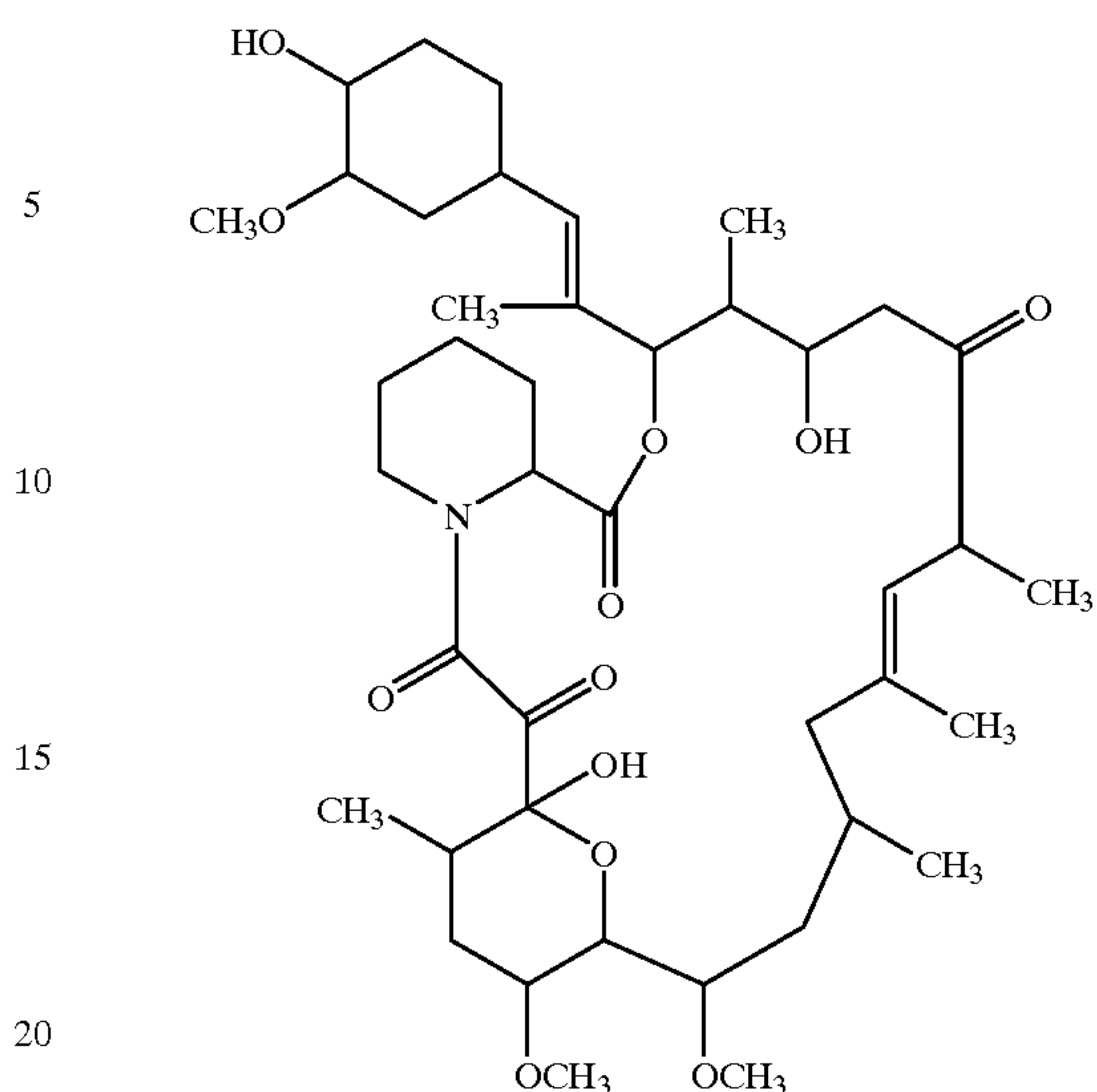
1,14-Dihydroxy-12-(2-(4-hydroxy-3-methoxycyclohexyl)-1-methylvinyl)-23,25-dimethoxy-13,19,17,21,27-pentamethyl-11,18-dioxo-4-azatricyclo[22.3.1.0 4,9 ]-octacos-18-ene-2,3,10,16-tetraone
