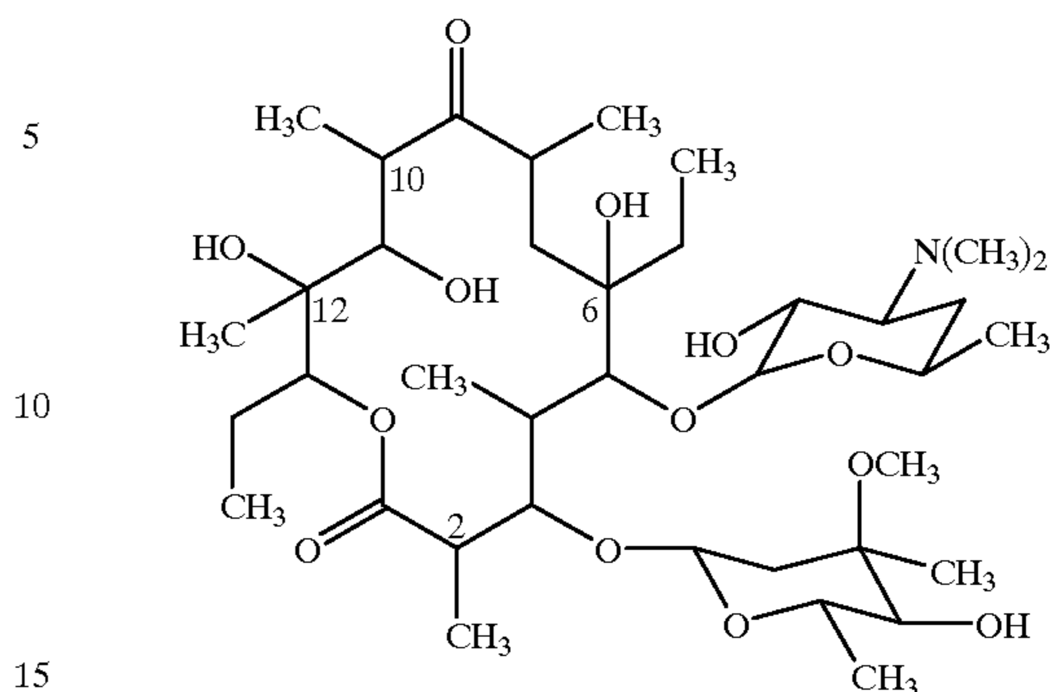
6-desmethyl-6-ethylerythromycin A
