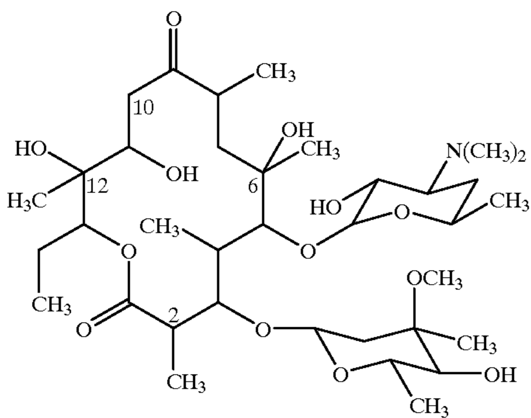
10-desmethylethylerythromycin A
