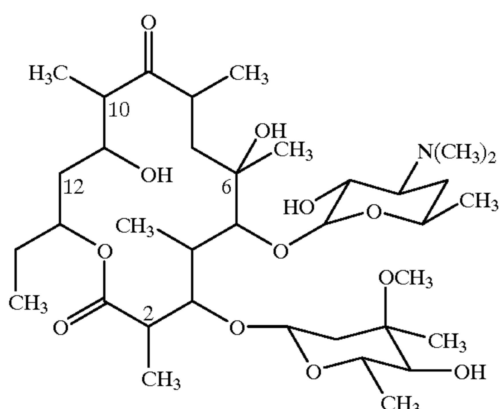
12-desmethyl-12-deoxyerythromycin A
