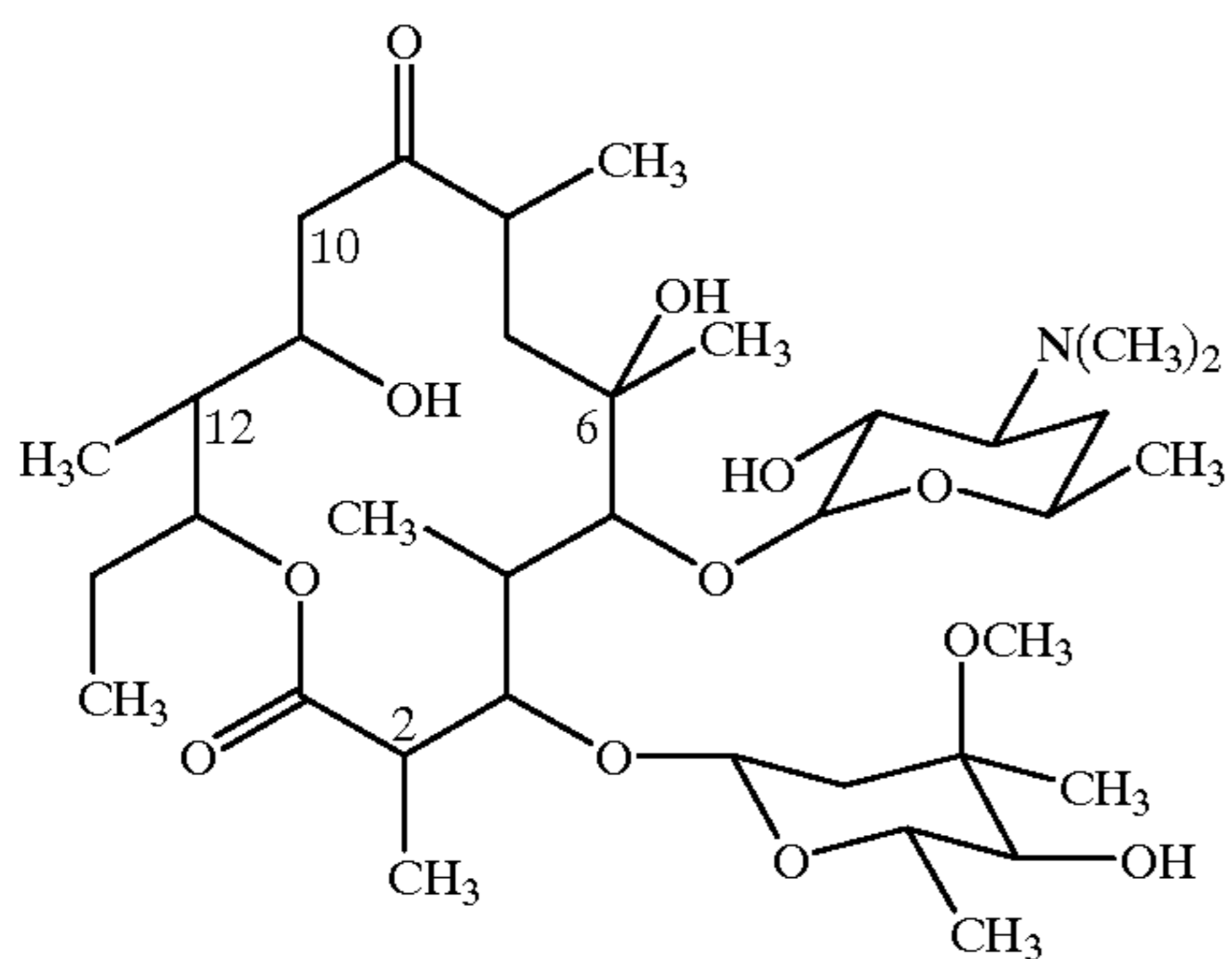
10-desmethyl-12-deoxyerythromycin A
