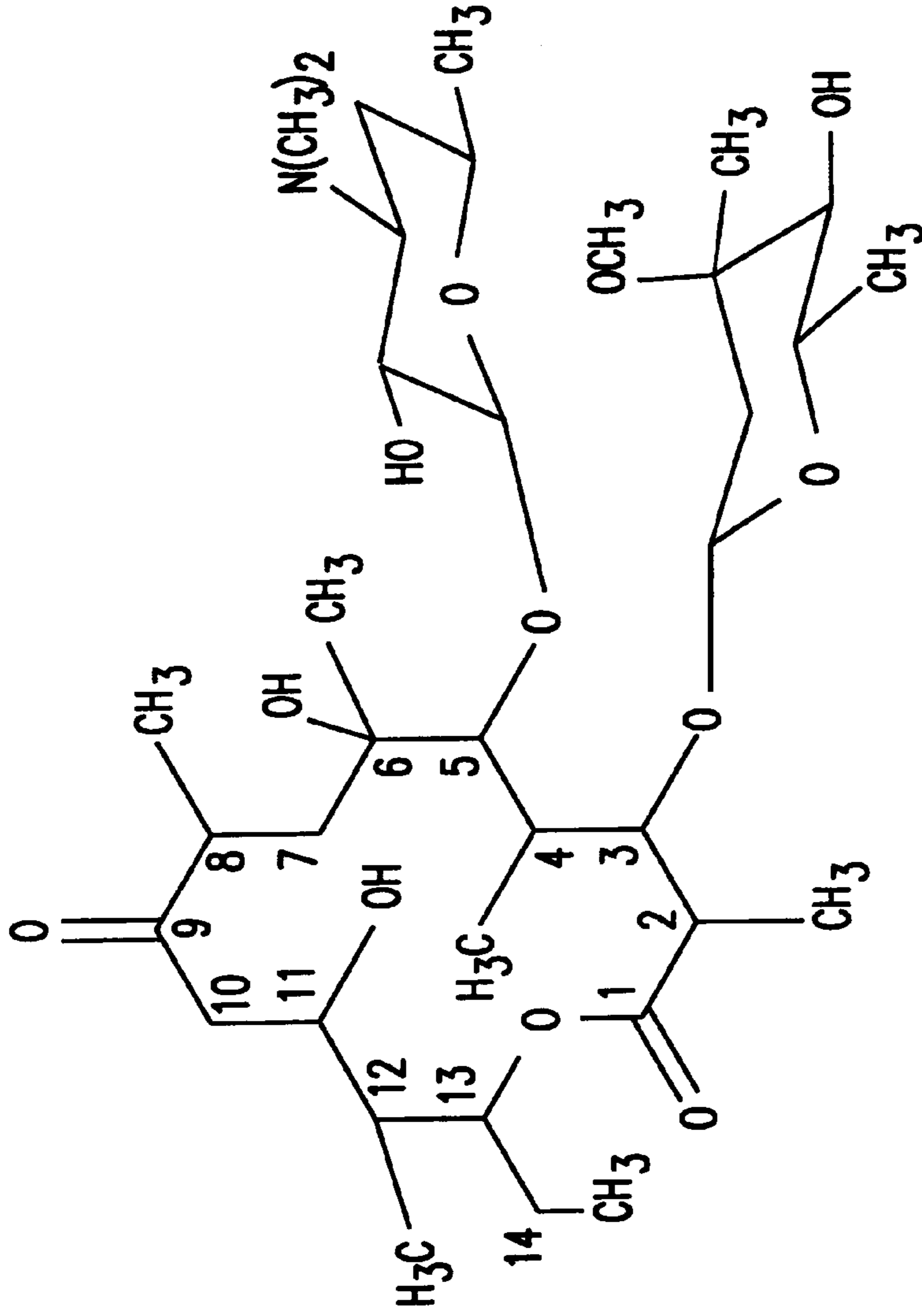
10-DESMETHYL-12-DEOXYERYTHROMYCIN A
