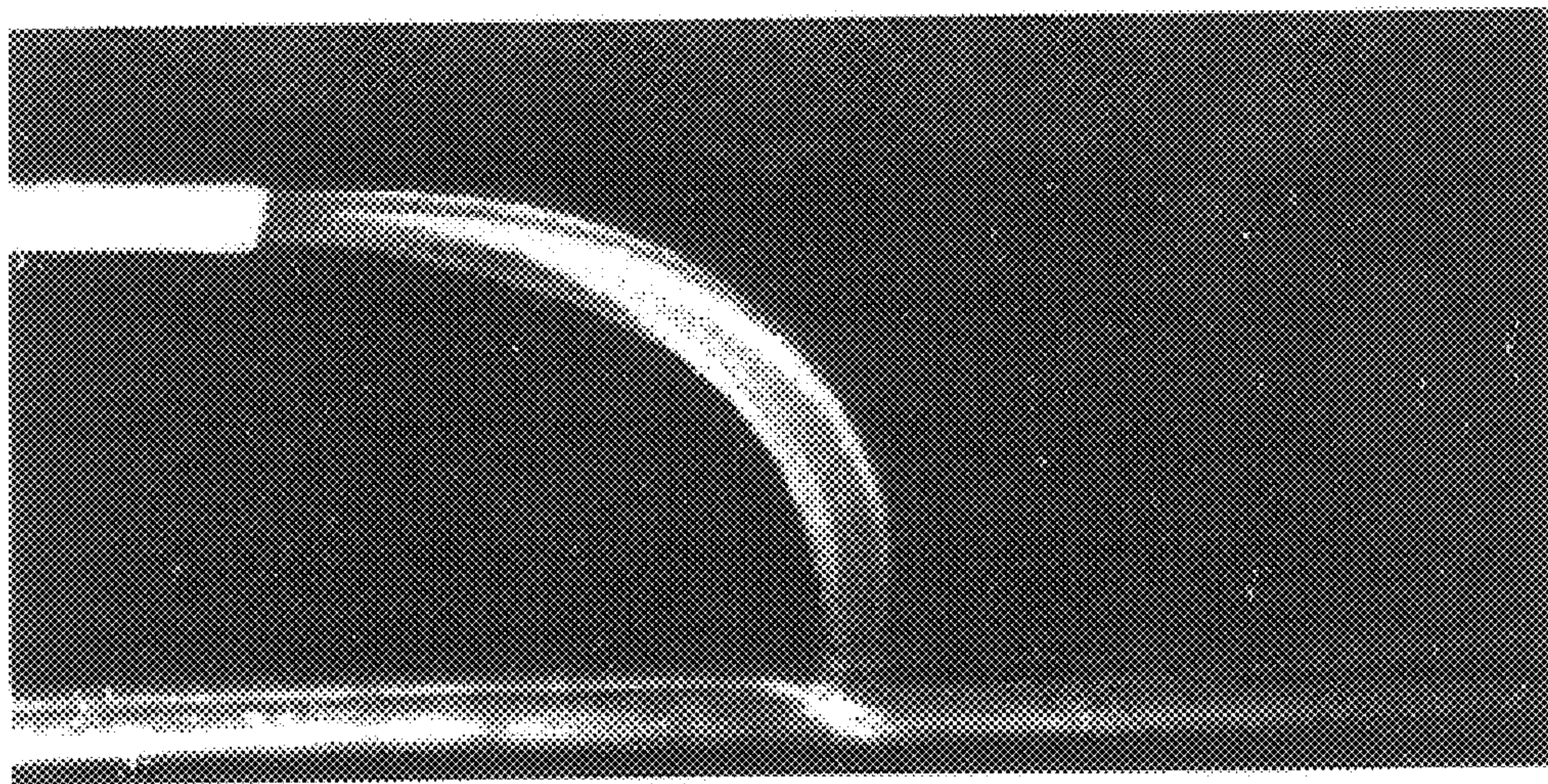
(b) Plasma On, E ~ 4.5 kV rms, F = 3 kHz
