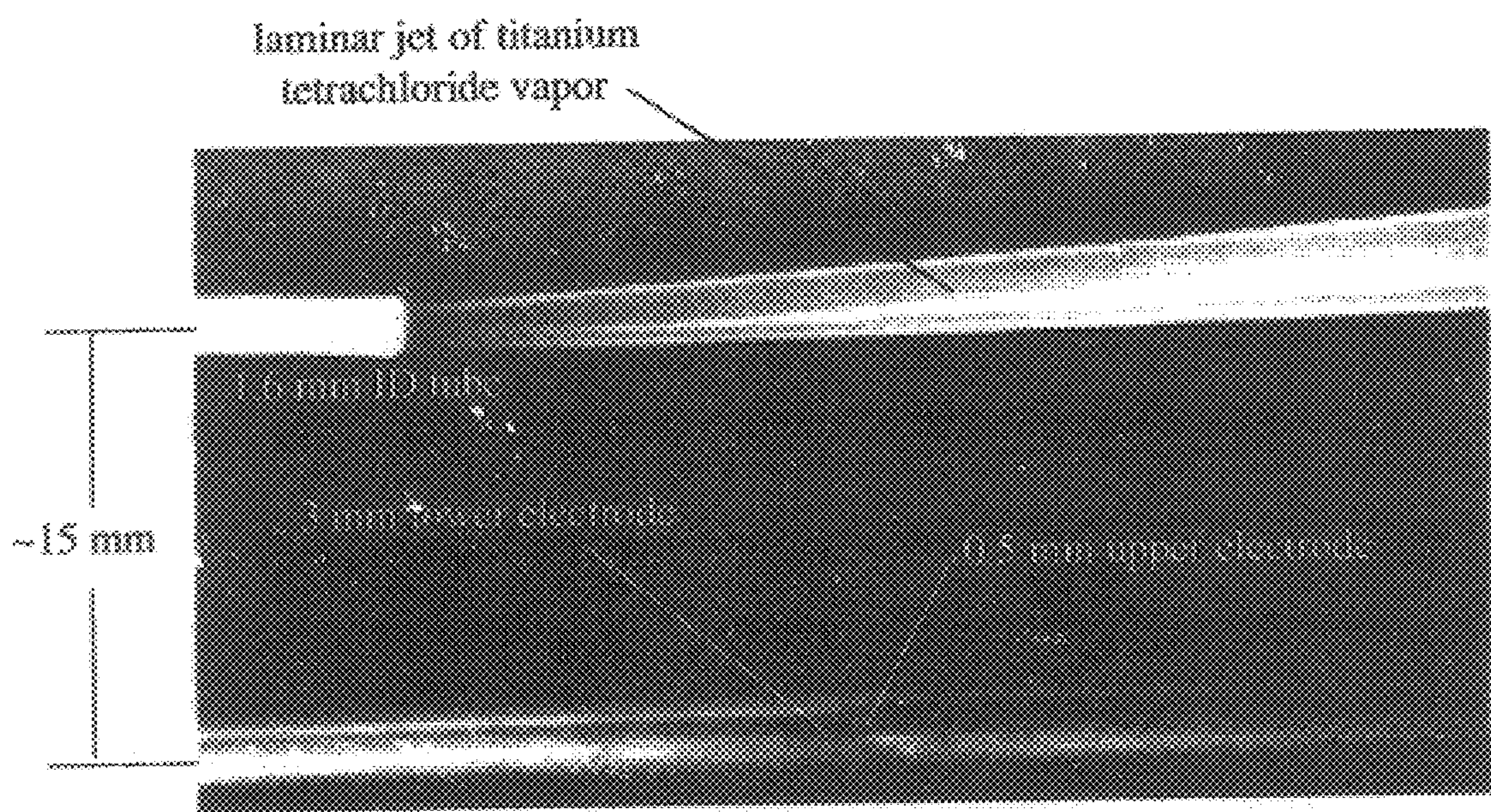
(a) Plasma Off
