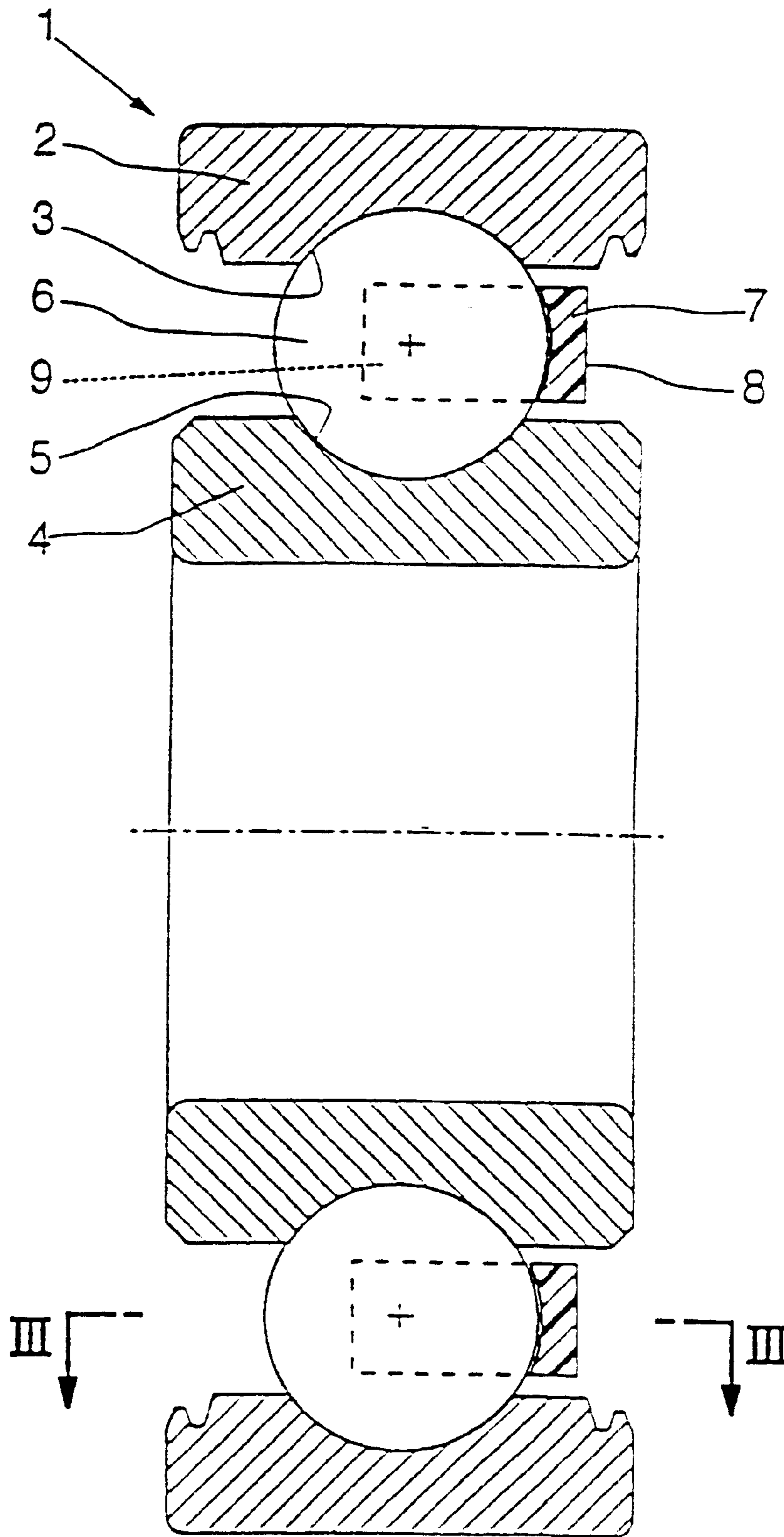
FIG. 1 (PRIOR ART)
