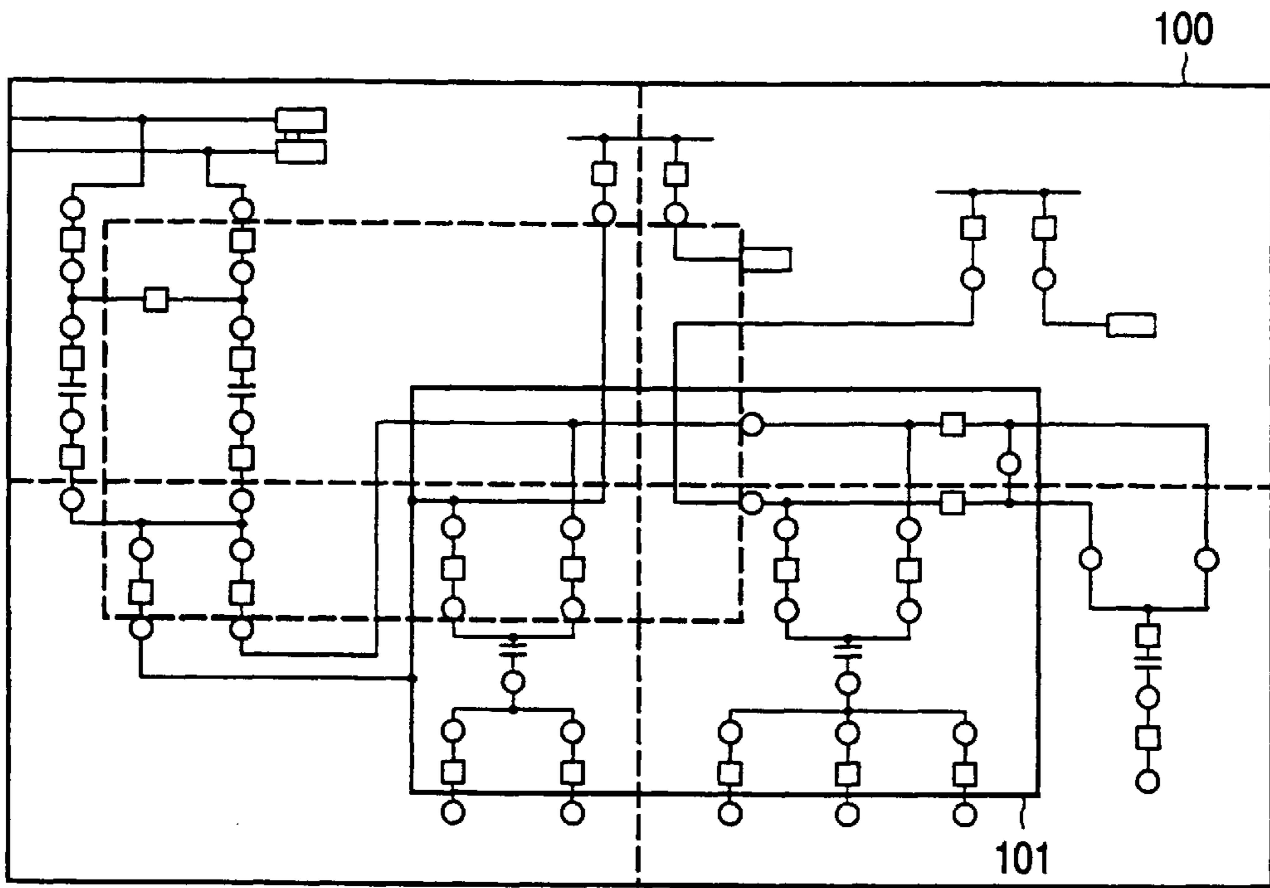
BACKGROUND ART FIG. 20
