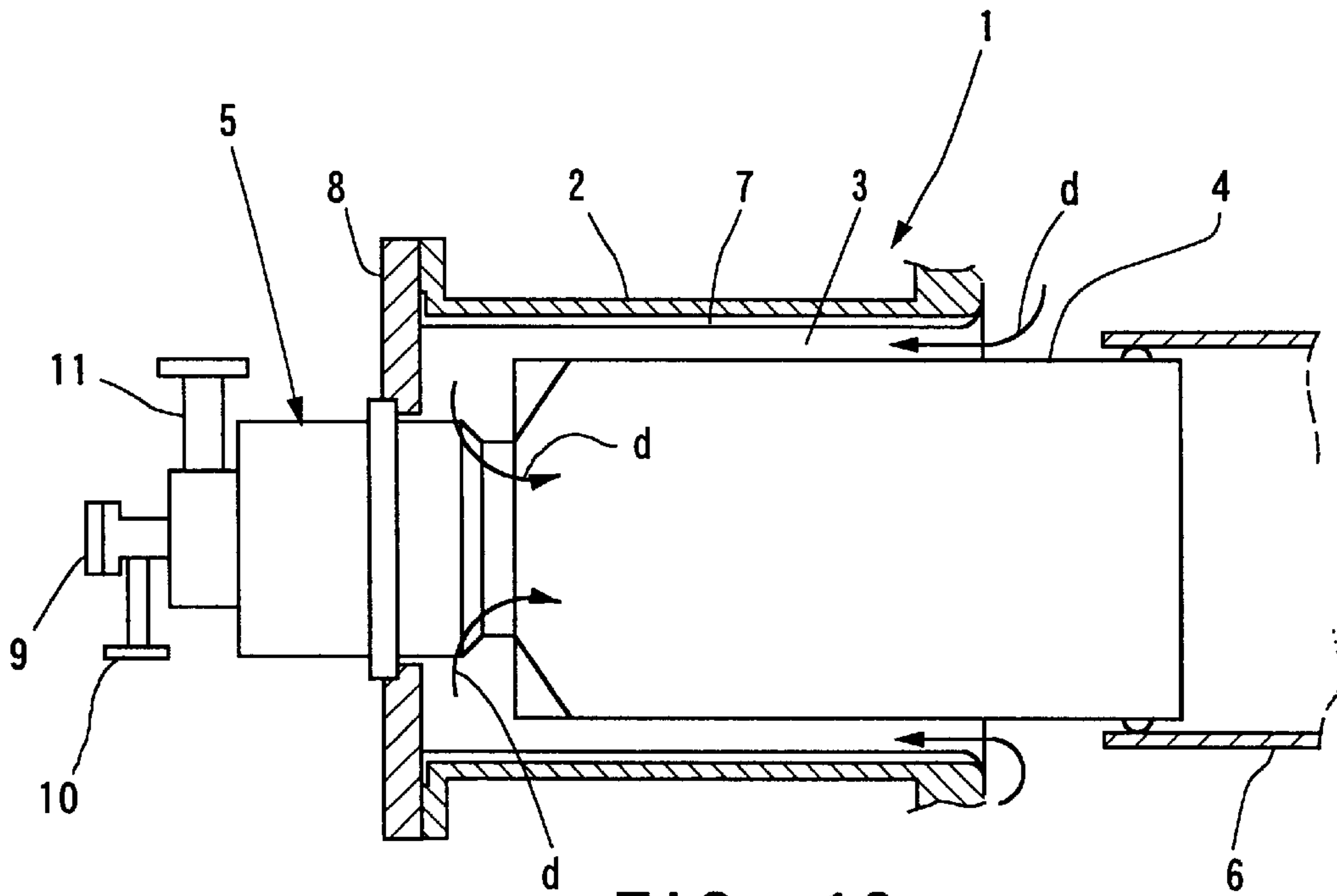
FIG. 10 PRIOR ART
