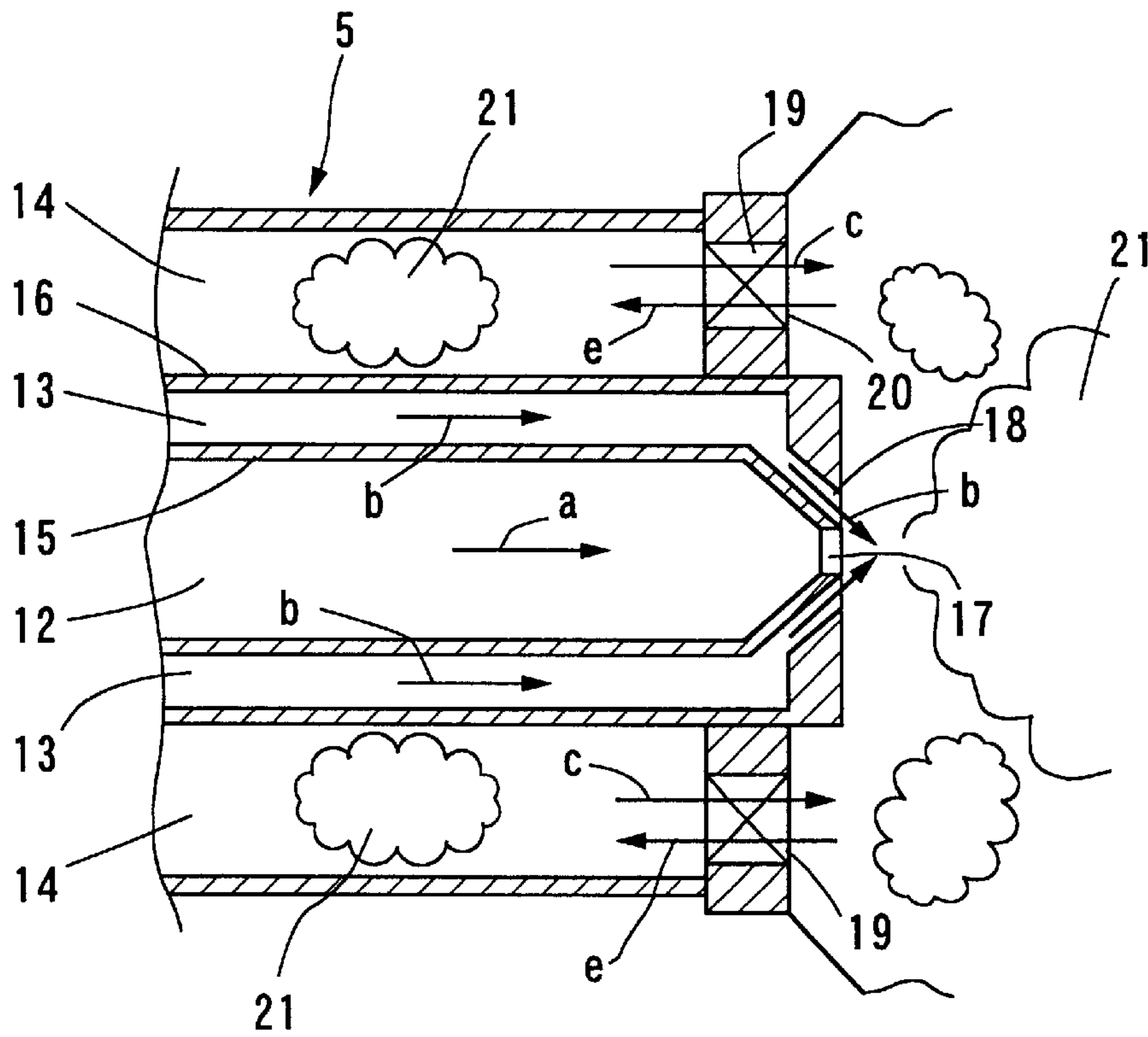
FIG. 11 PRIOR ART
