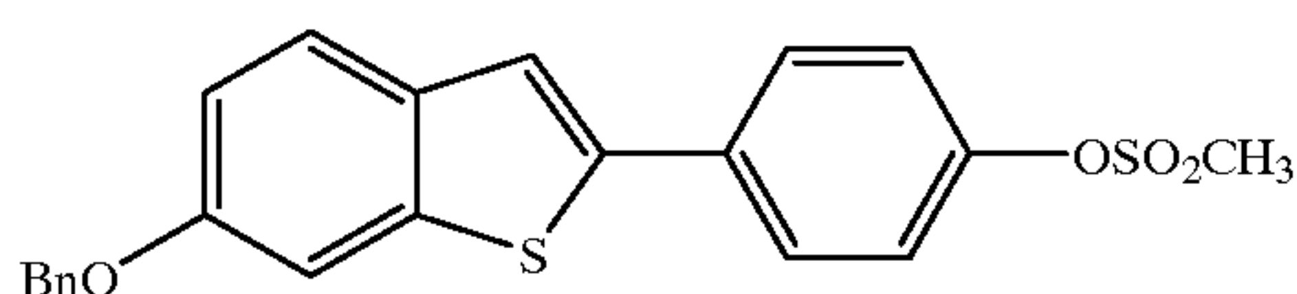
[6-Benzyloxy-2-(4-methanesulfonyloxyphenyl)]benzo[b]thiophene
