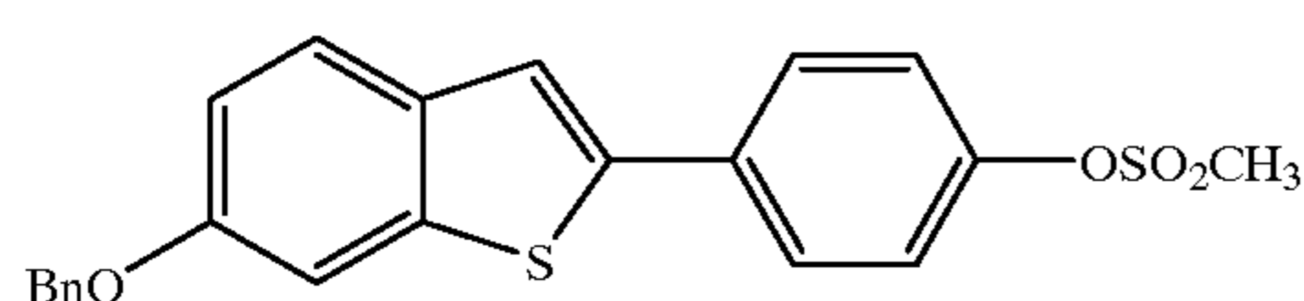
[6-Benzyloxy-2-(4-methanesulfonyloxyphenyl)]benzo[b]thiophene
