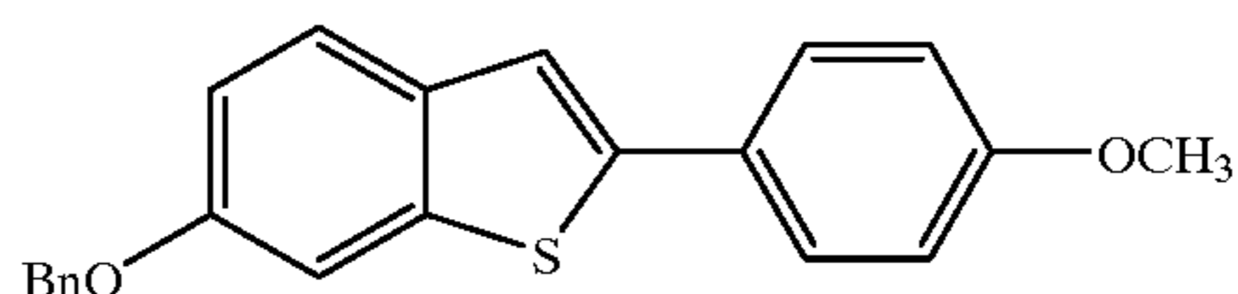
[6-Benzyloxy-2-(4-methoxyphenyl)]benzo[b]thiophene
