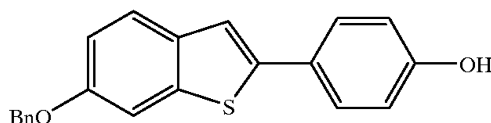
[6-Benzyloxy-2-(4-hydroxyphenyl)]benzo[b]thiophene
