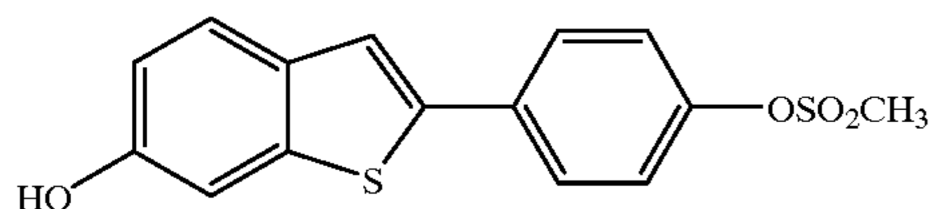
[6-Hydroxy-2-(4-methanesulfonyloxyphenyl)]benzo[b]thiophene
