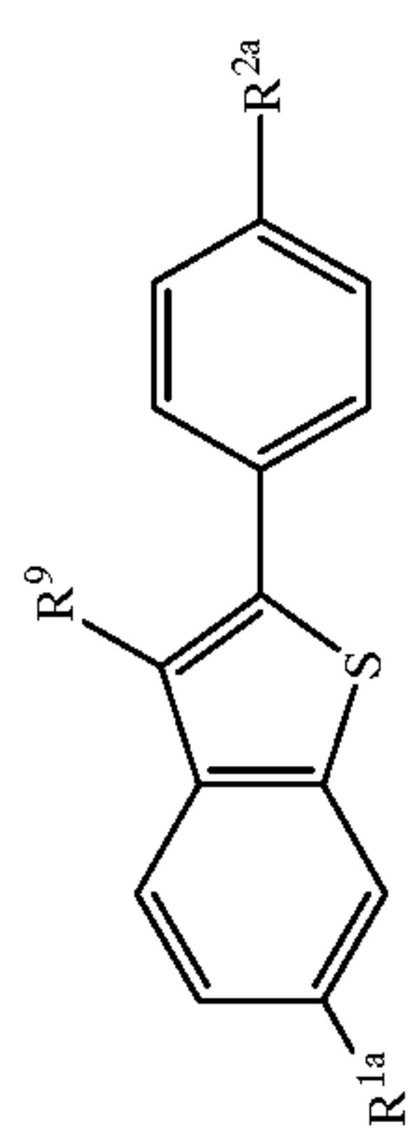
Scheme V
