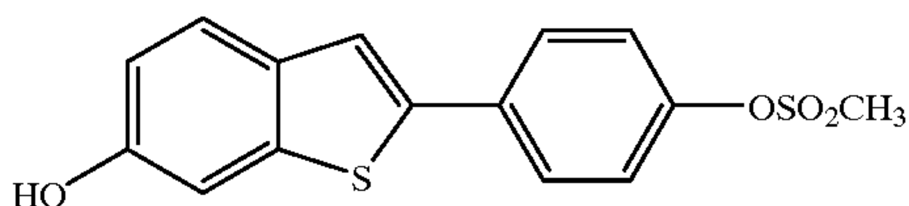
[6-Hydroxy-2-(4-methanesulfonyloxyphenyl)]benzo[b]thiophene
