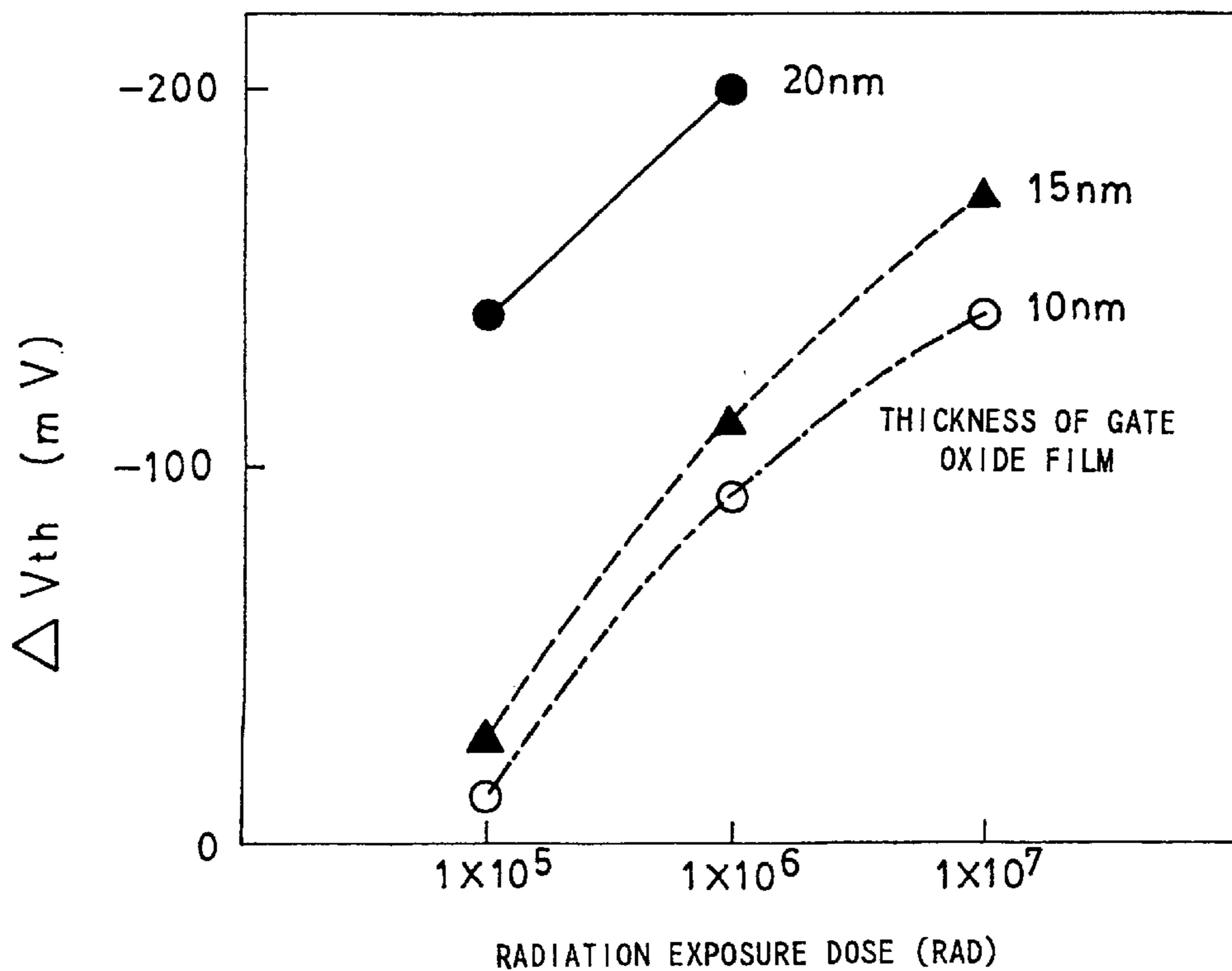
FIG. 52 PRIOR ART
