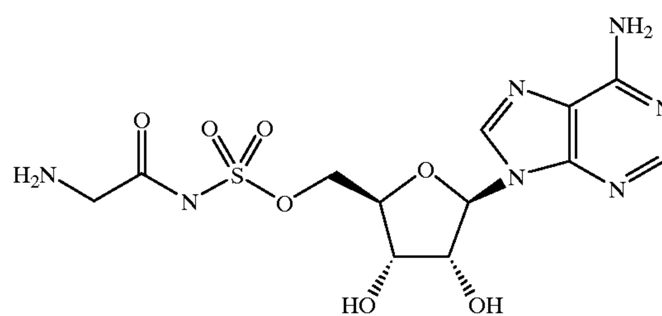
Glycylsulfamoyladenine
