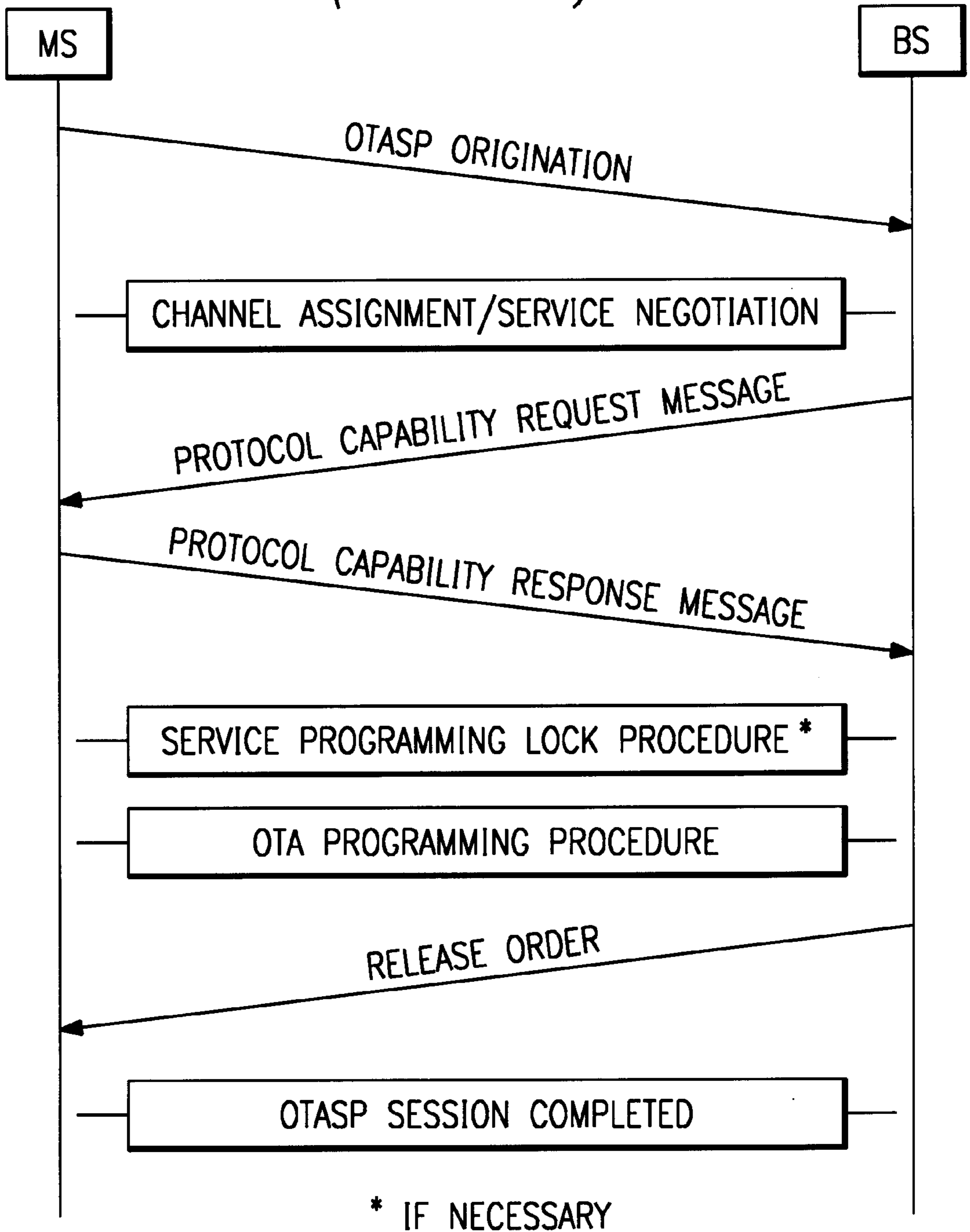
FIG. 2 (PRIOR ART)
