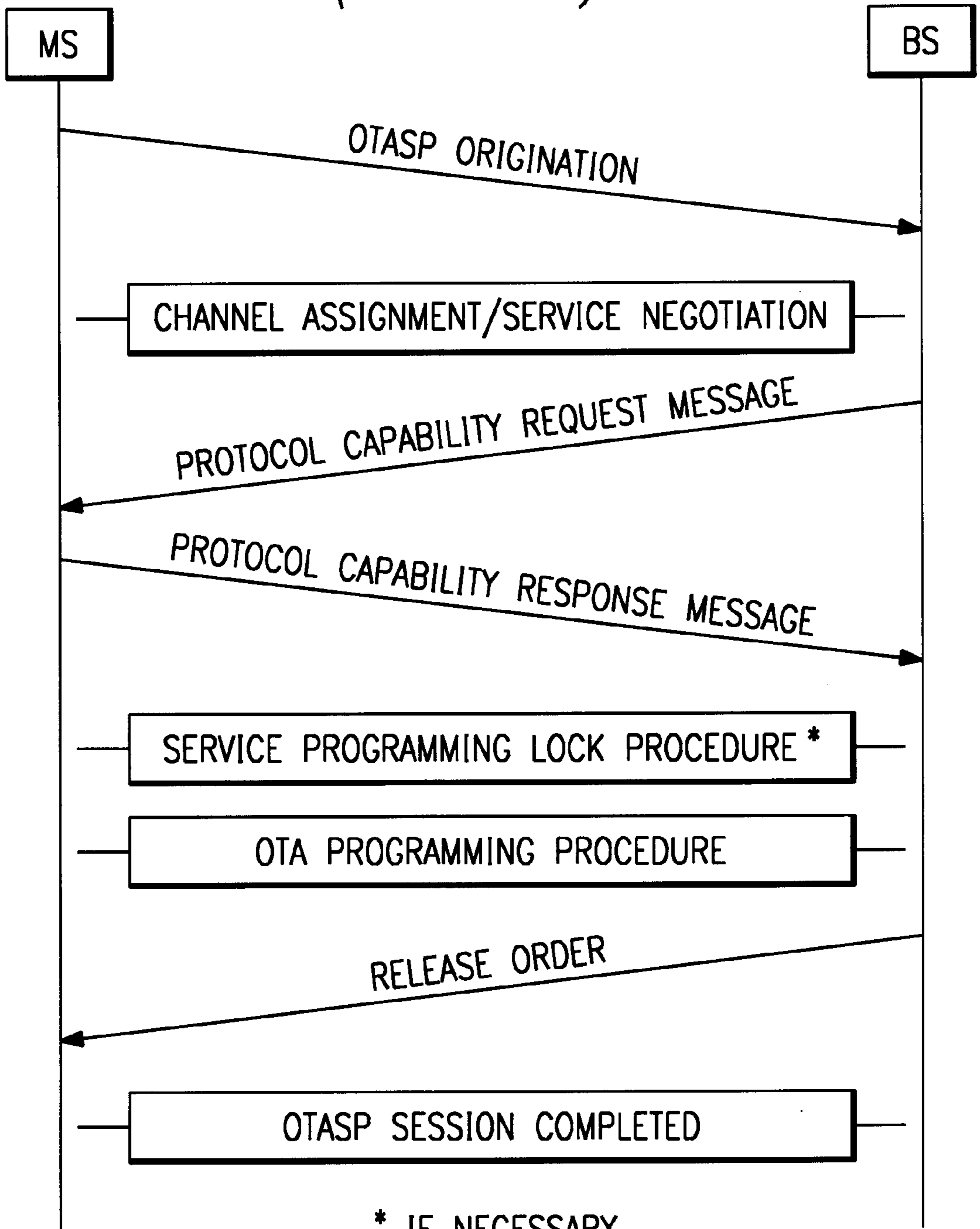
FIG. 2 (PRIOR ART)
