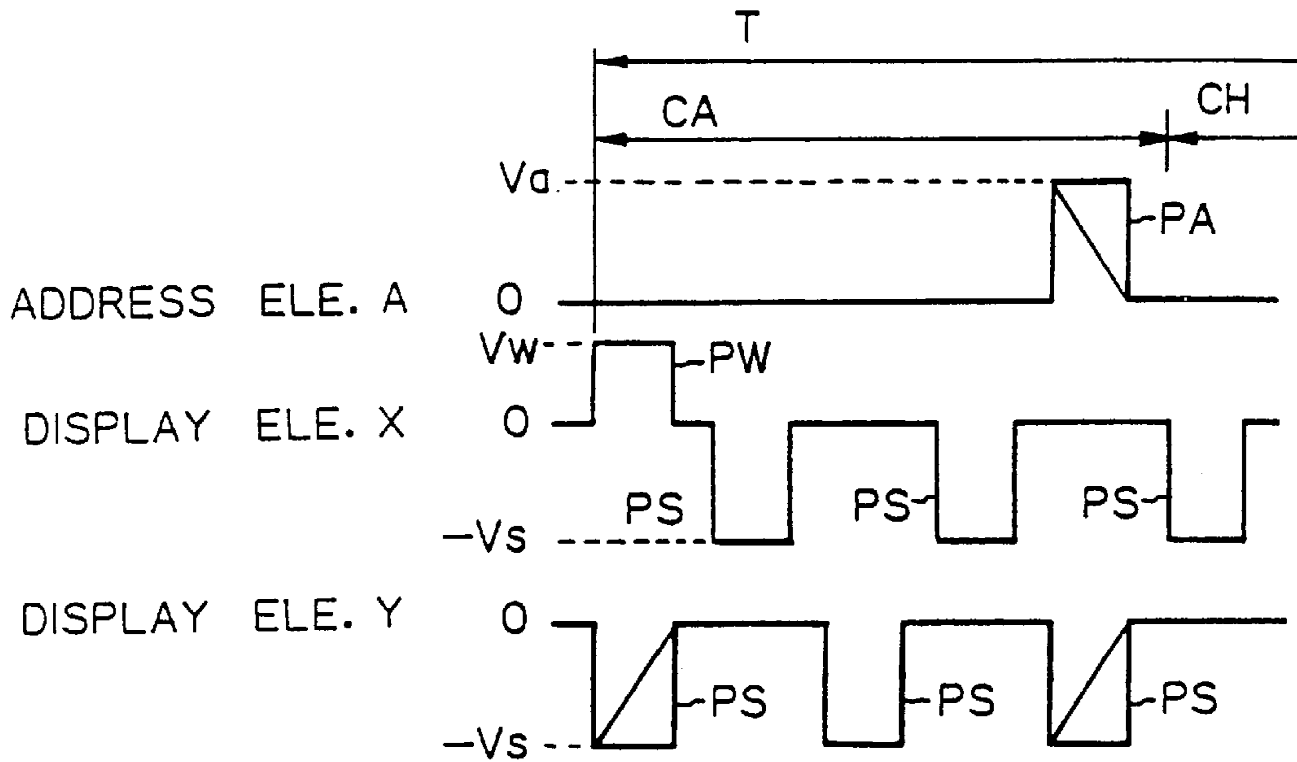
Fig. 5 PRIOR ART
