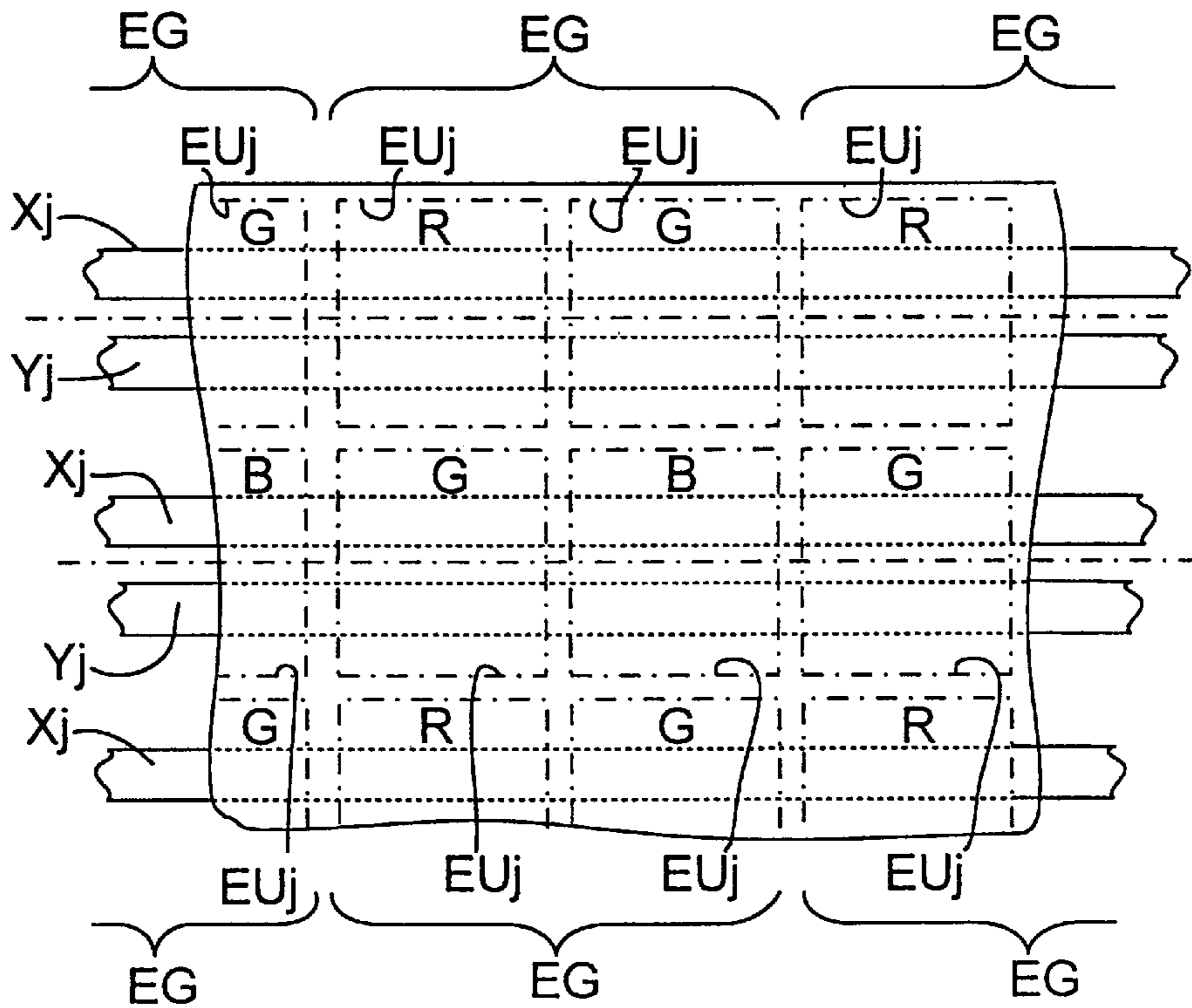
Fig. 6 PRIOR ART
