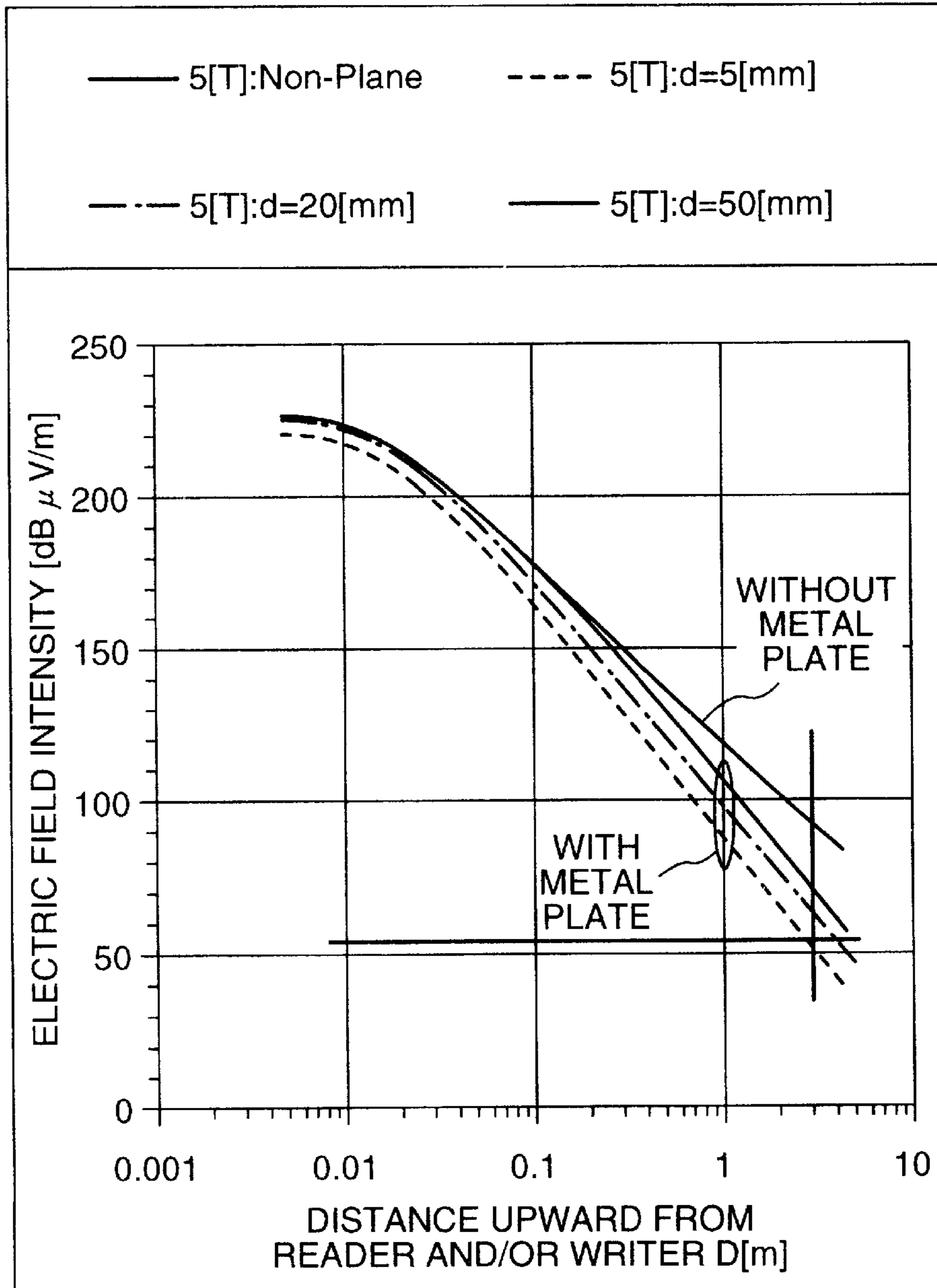
ELECTRIC FIELD INTENSITY VS. VERTICAL DISTANCE FROM READER AND/OR WRITER ANTENNA
