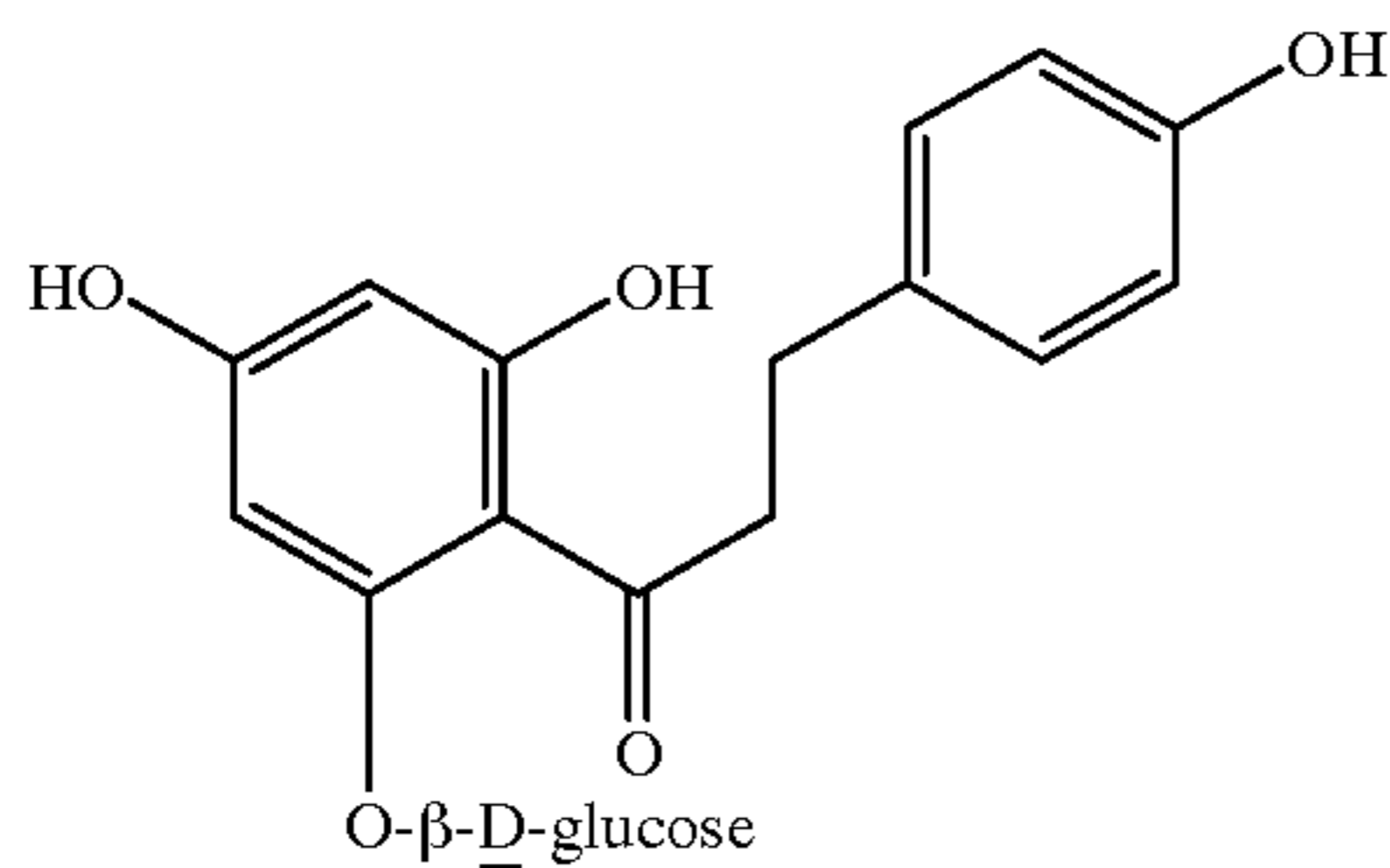
Phloretin
