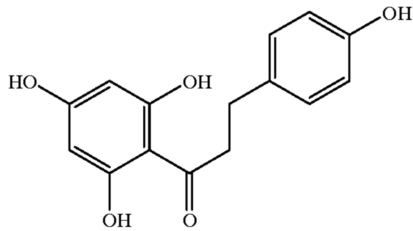
Phloretin
