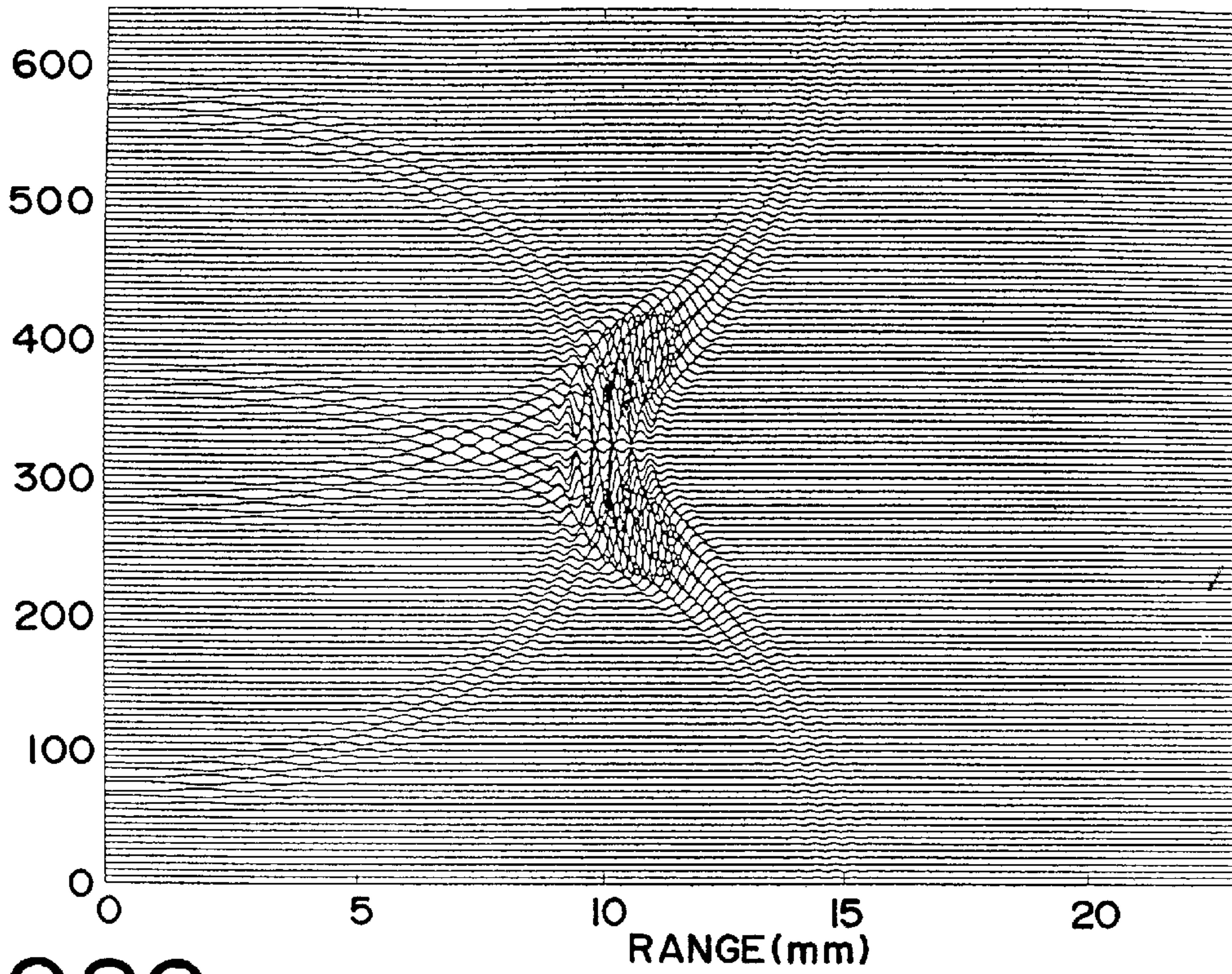
PULSE STRUCTURE AT t=10.0\text{mm}/1.54\text{mm}/\text{us}
