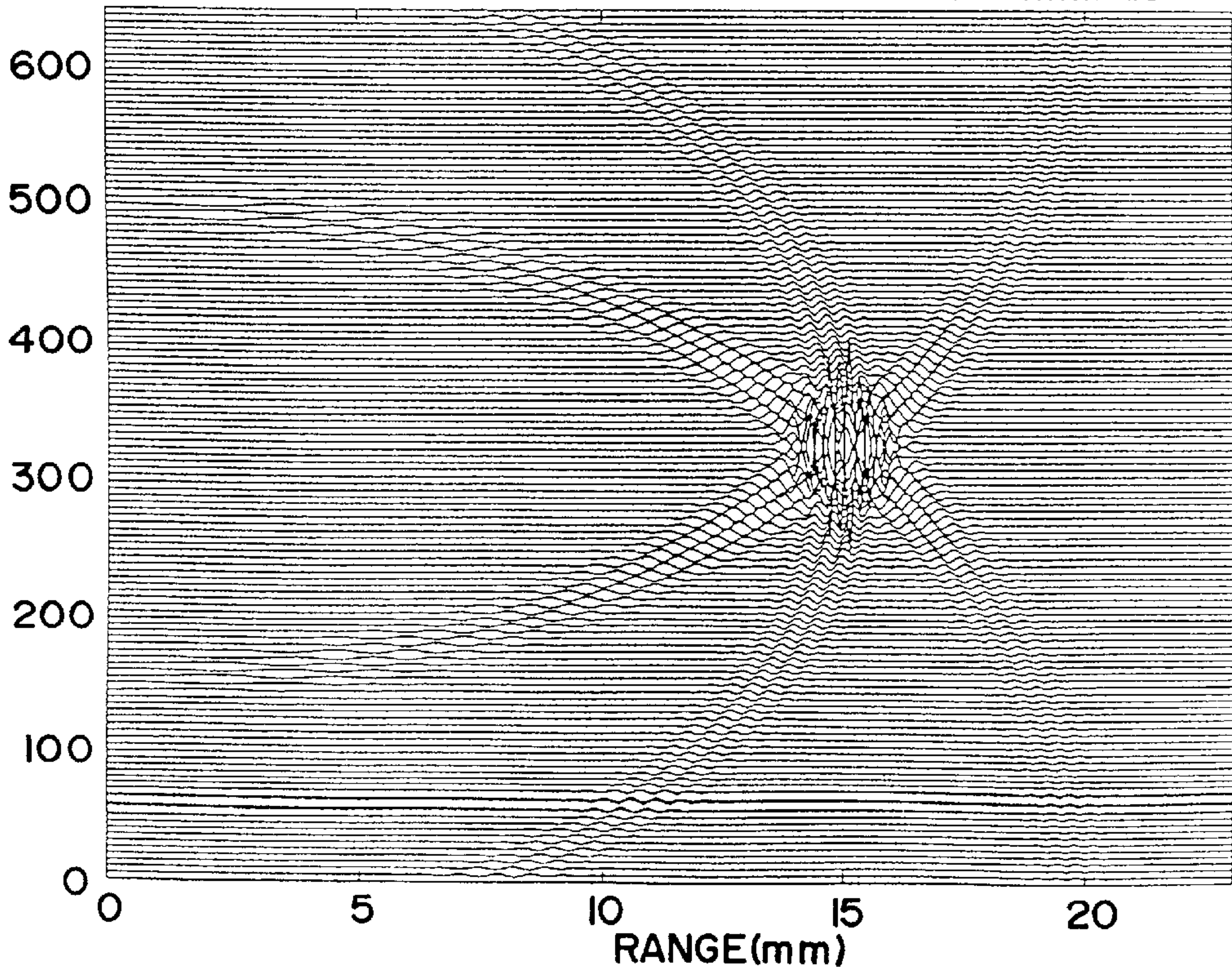
PULSE STRUCTURE AT t=15.0\text{mm}/1.54\text{mm}/\text{us}
