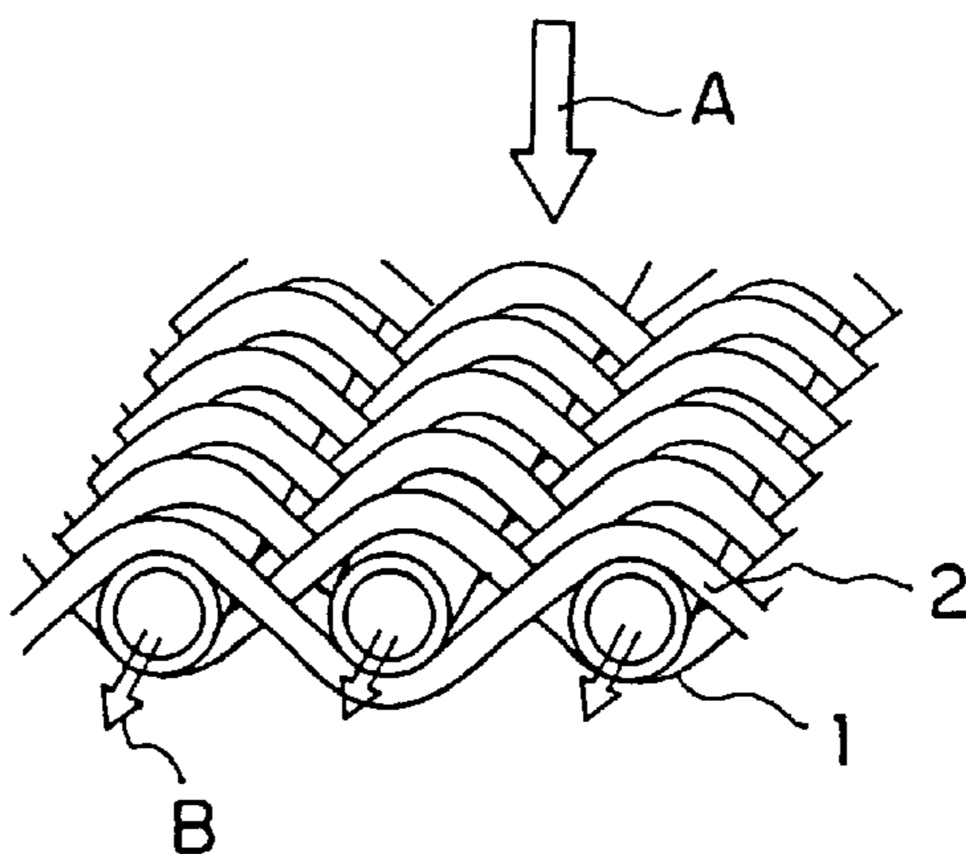
FIG. 65 (PRIOR ART)
