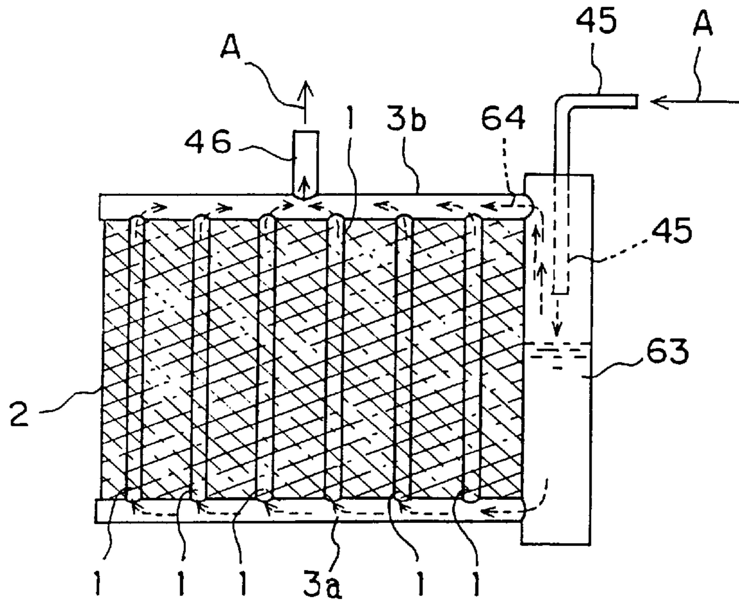
FIG. 68 (PRIOR ART)
