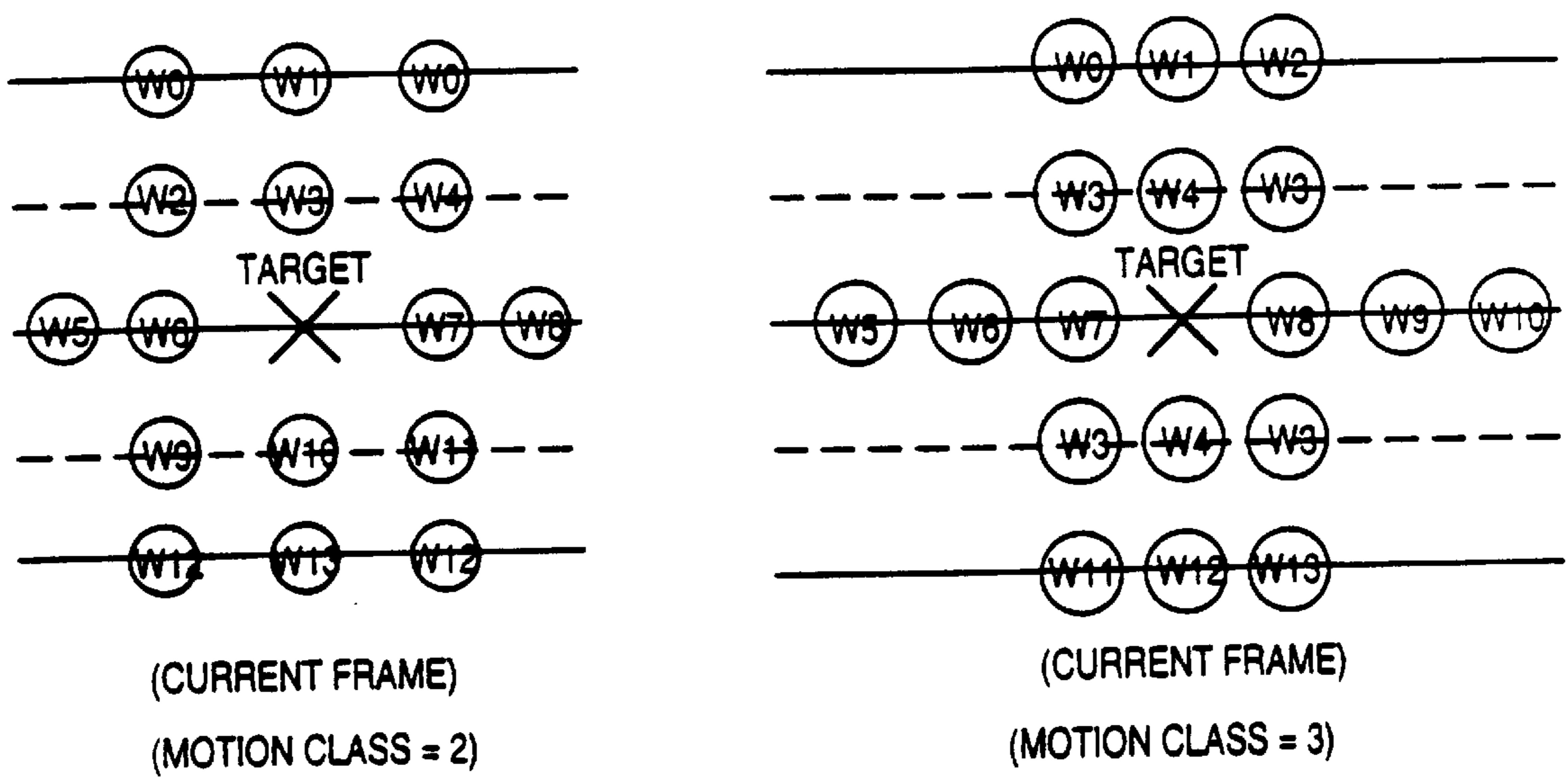
FIGURE 12 : ADAPTIVE FILTER TAP (ERROR CLASS0)
