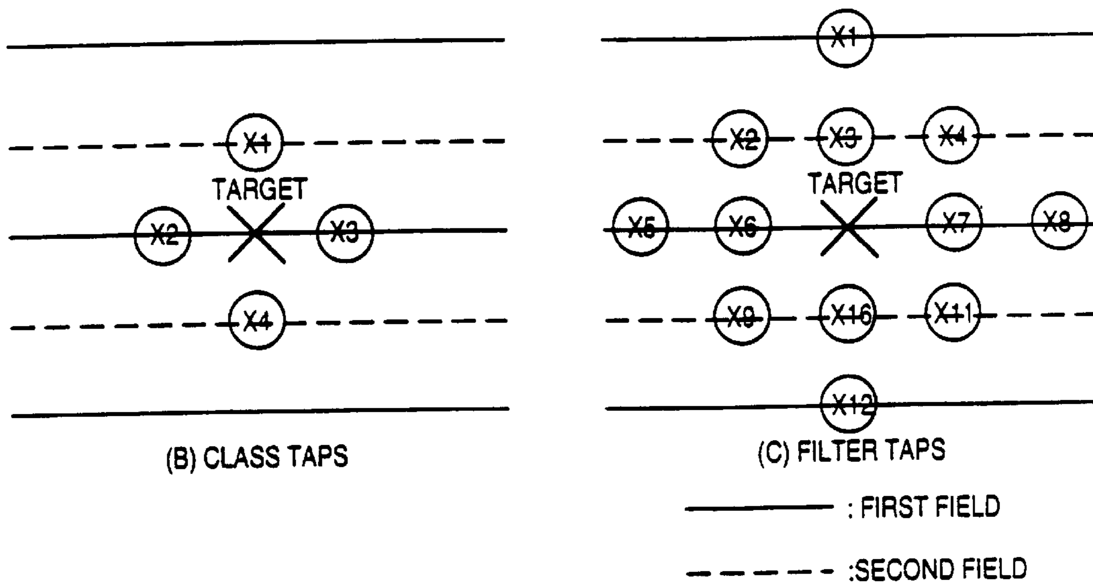
FIGURE 2 : CLASSIFIED ADAPTIVE ERROR RECOVERY METHOD
