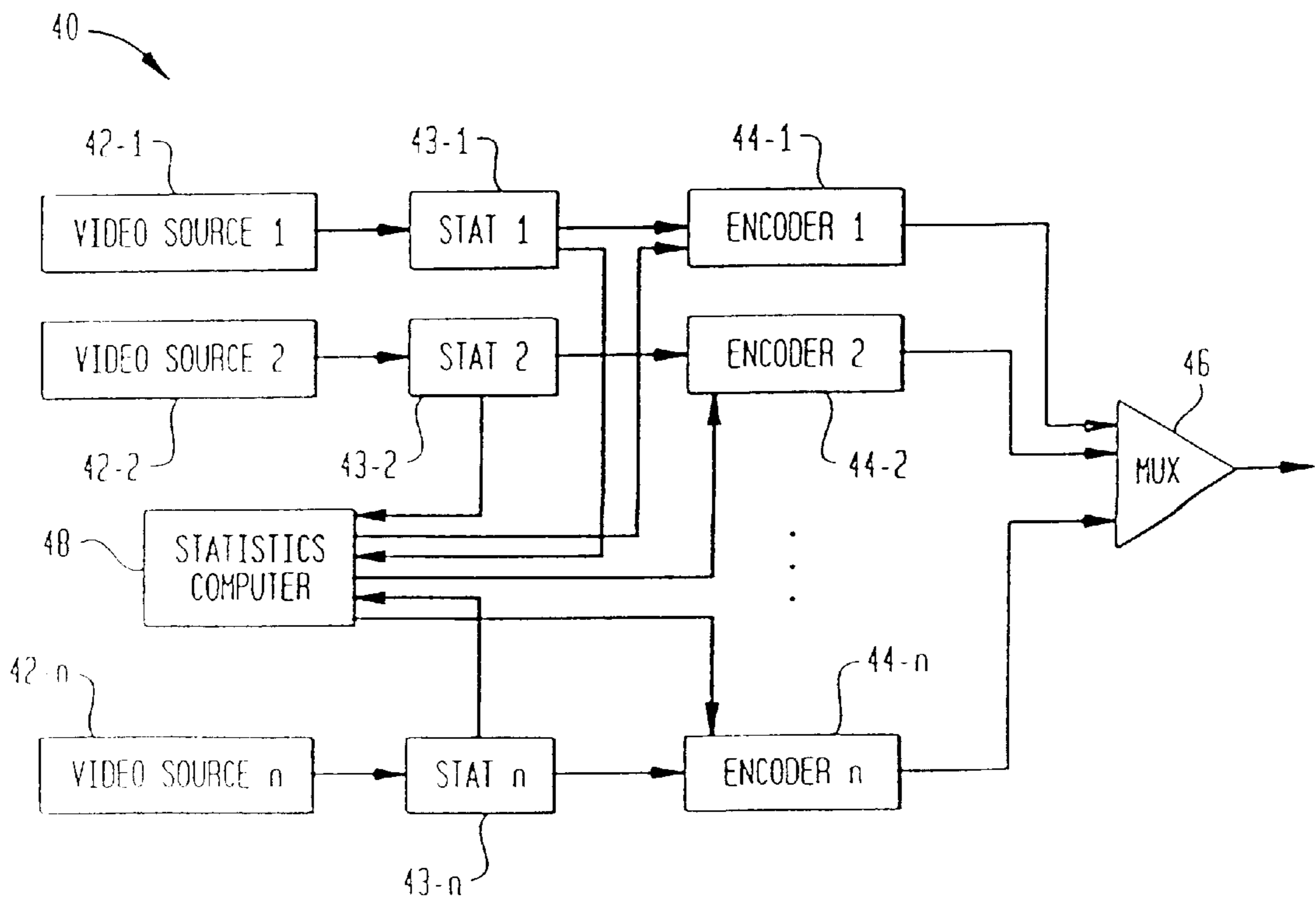
FIG. 2 (PRIOR ART)
