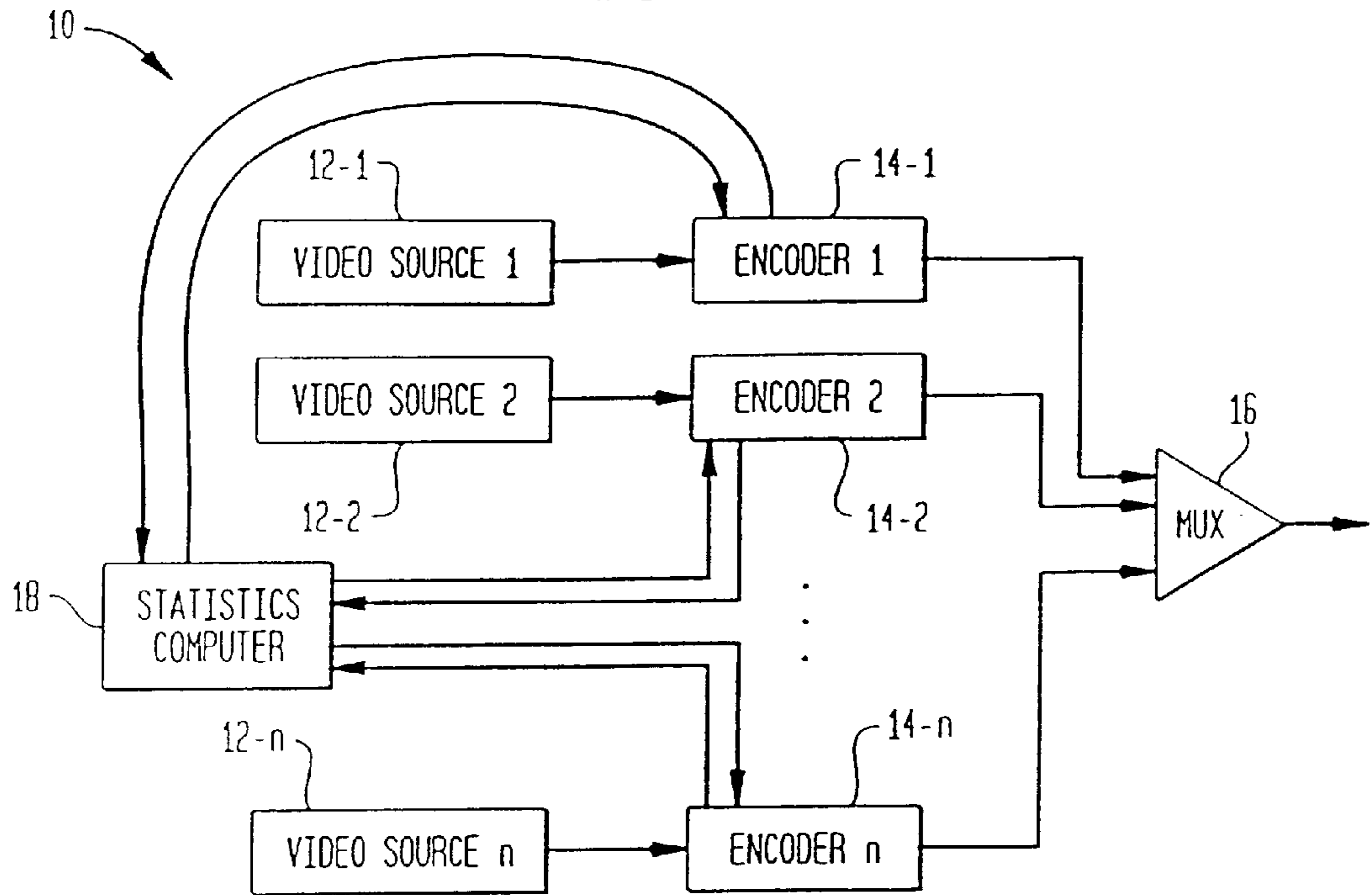
FIG. 1 (PRIOR ART)
