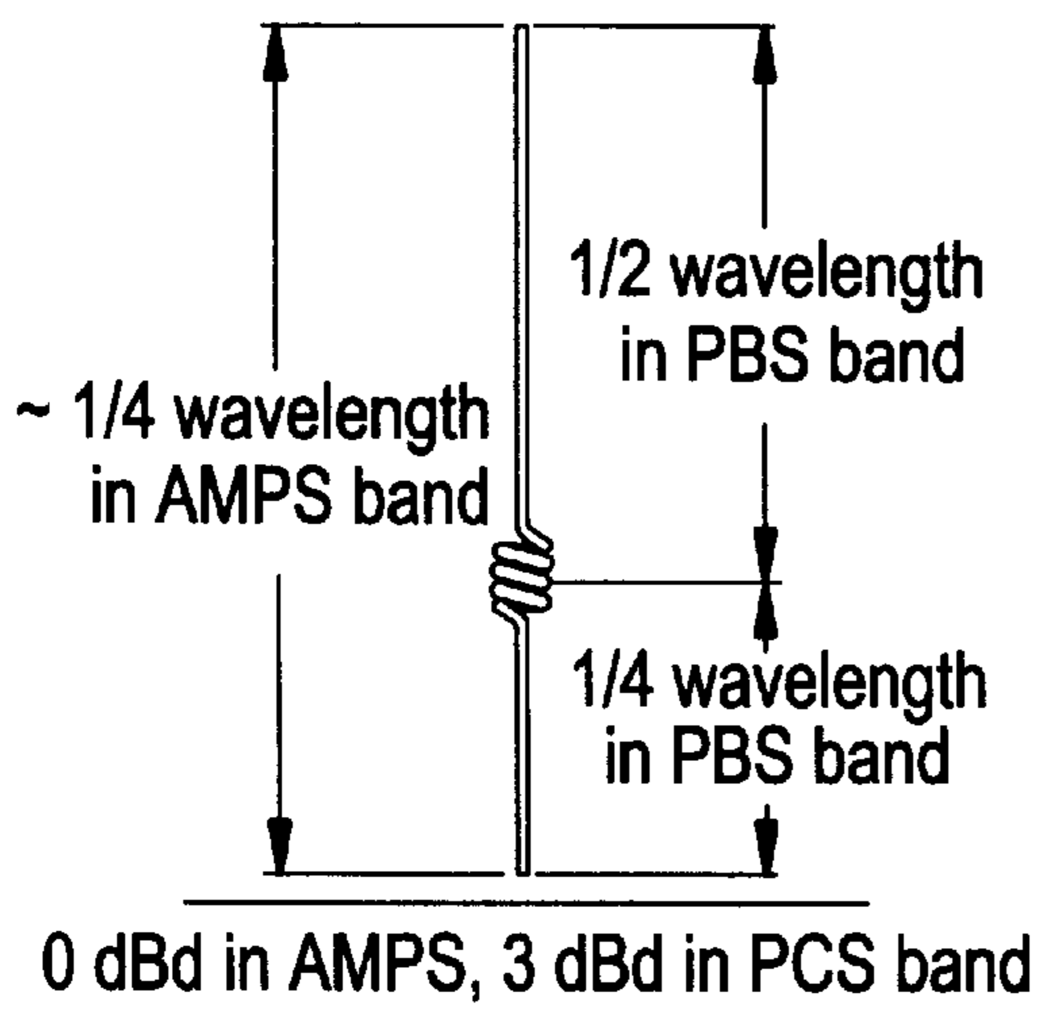
FIG. 3 PRIOR ART
