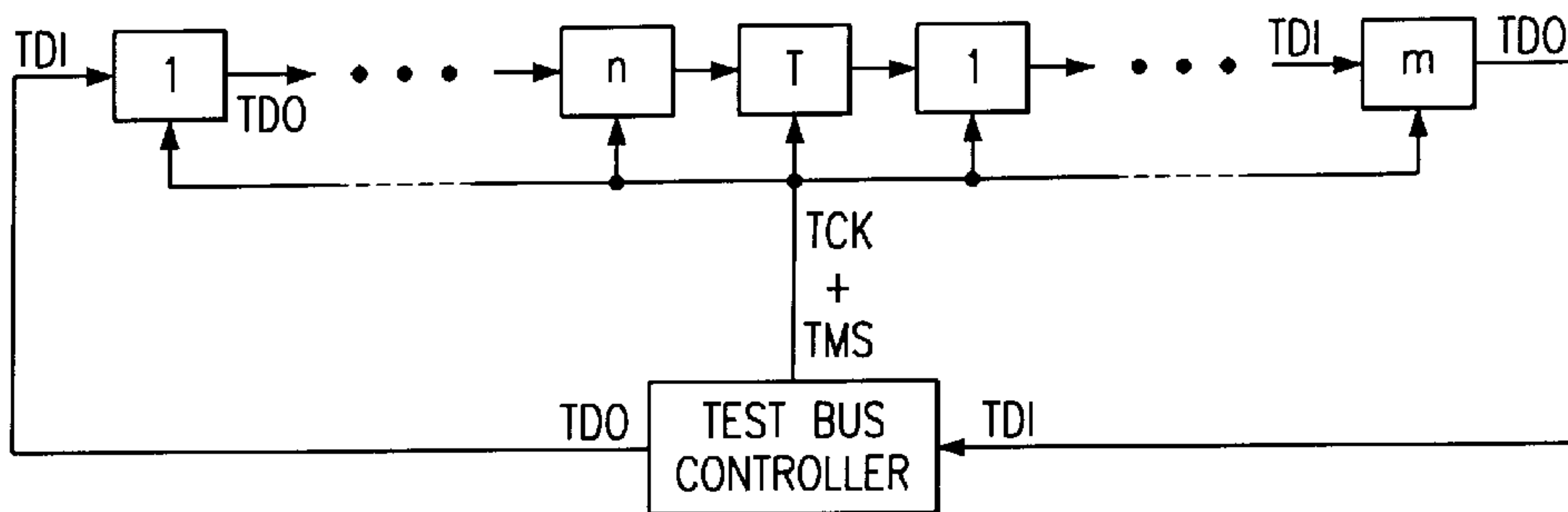
FIG. 7 (PRIOR ART)
