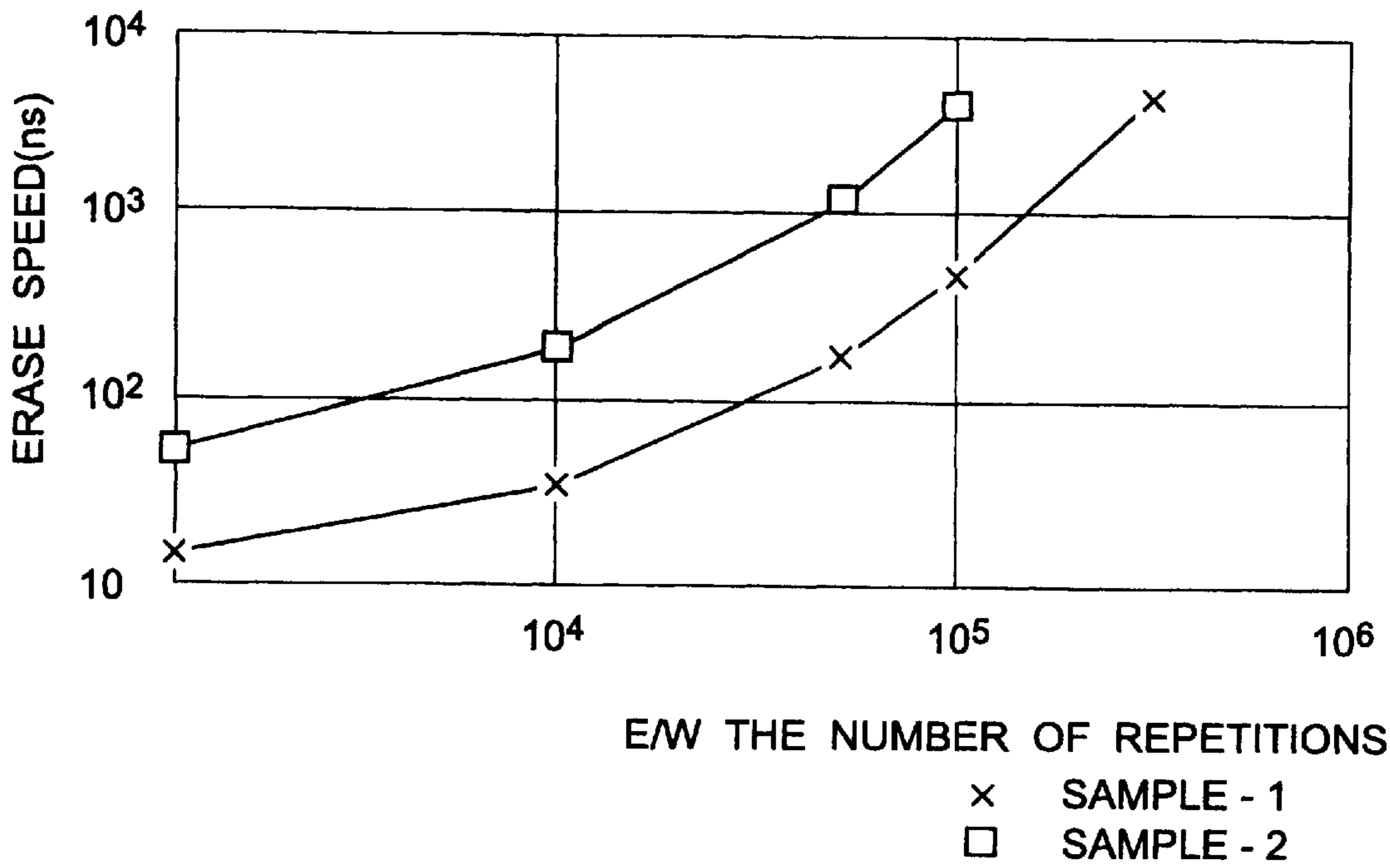
FIG.8A
