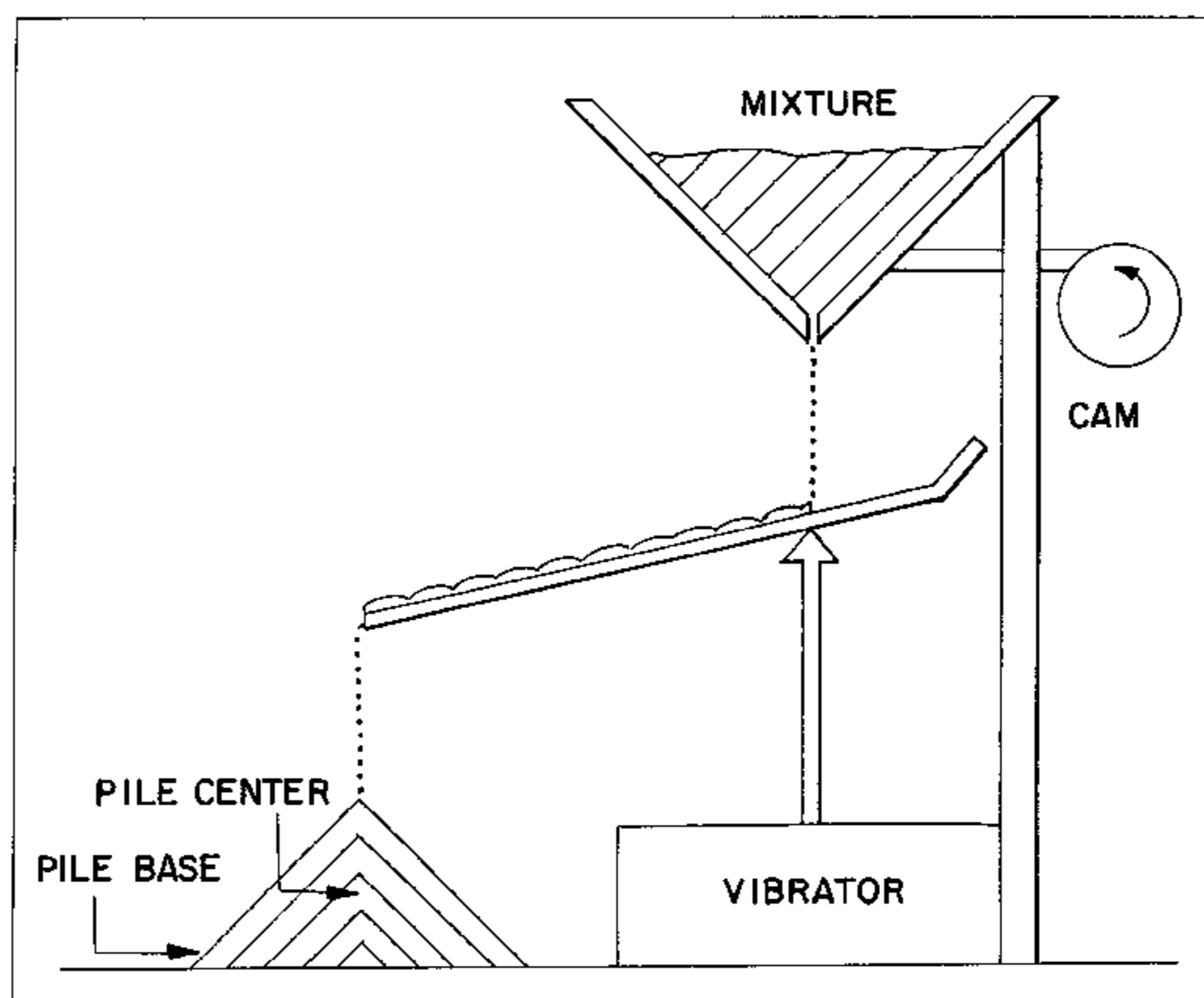
SEPARATION TEST
