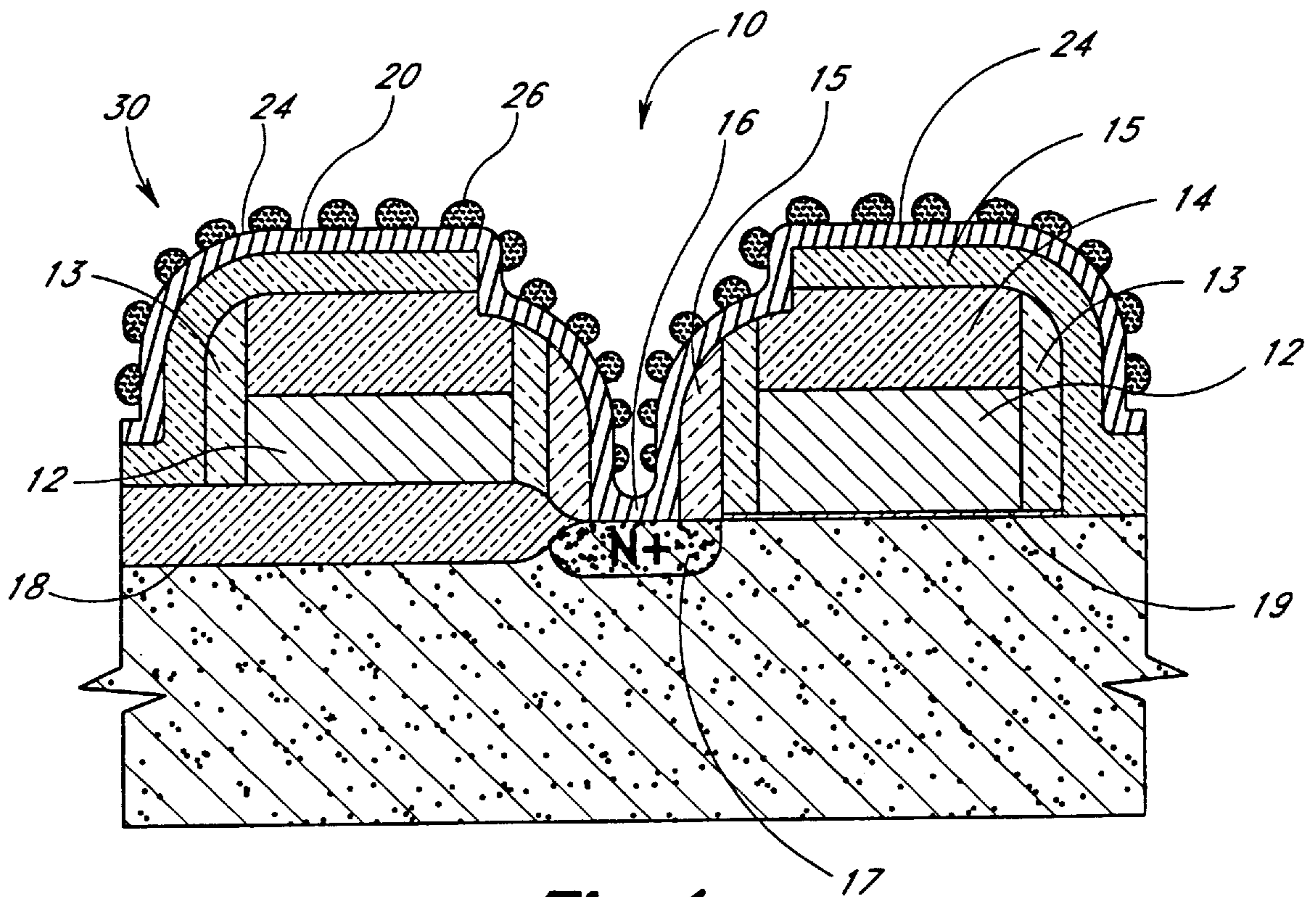
Fig. 1 (PRIOR ART)
