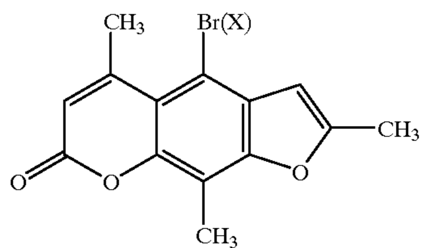
Compound #10 X = I, Compound #10b
