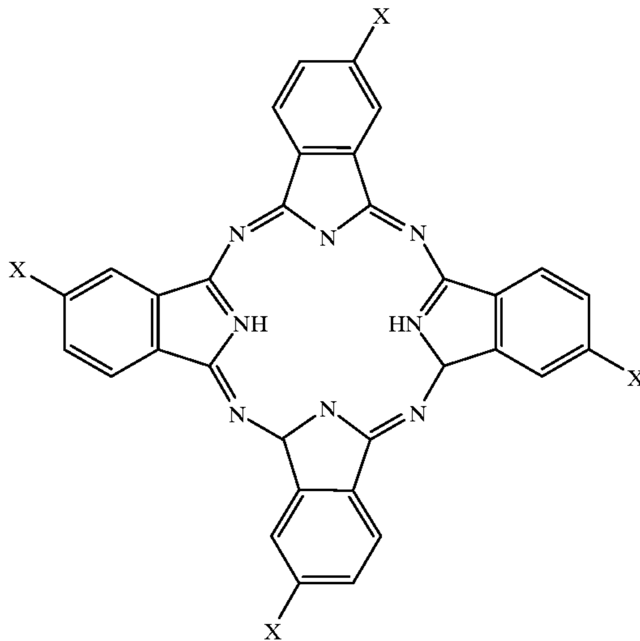
X = Br PHTH-Br Compound #11 X = I PHTH-I Compound #12
