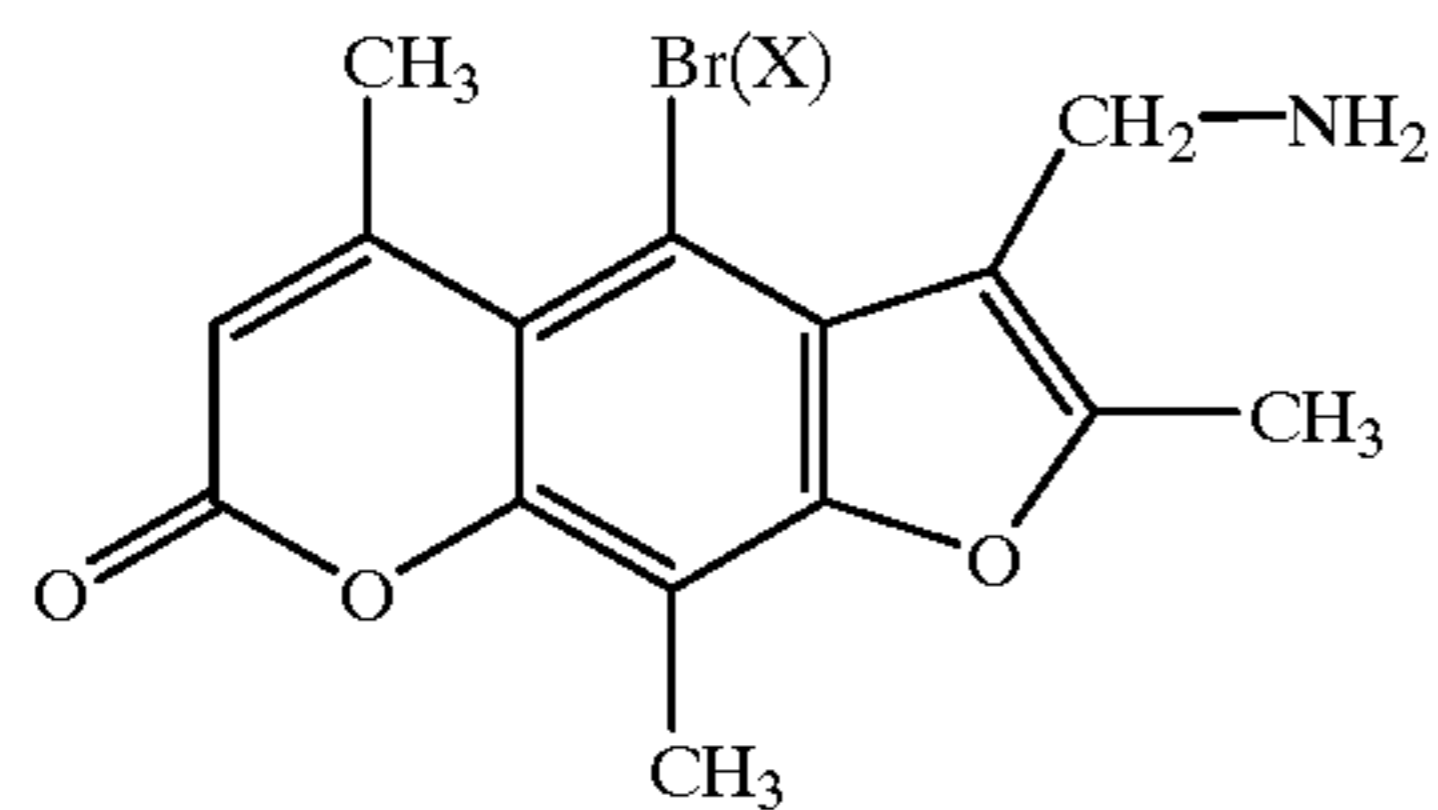
Compound #10 X = I, Compound #10b
