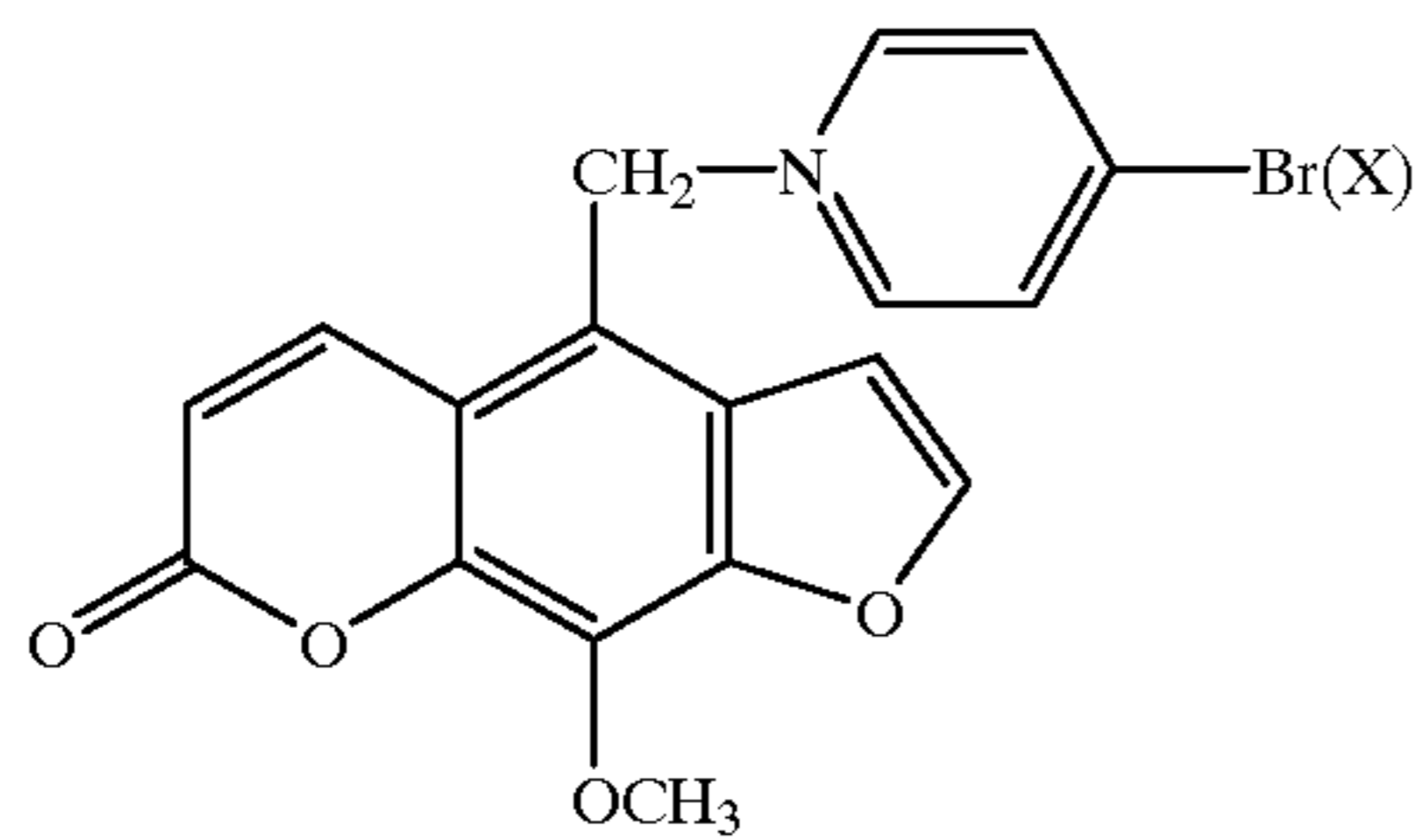
Compound #6 X = I Compound 6b
