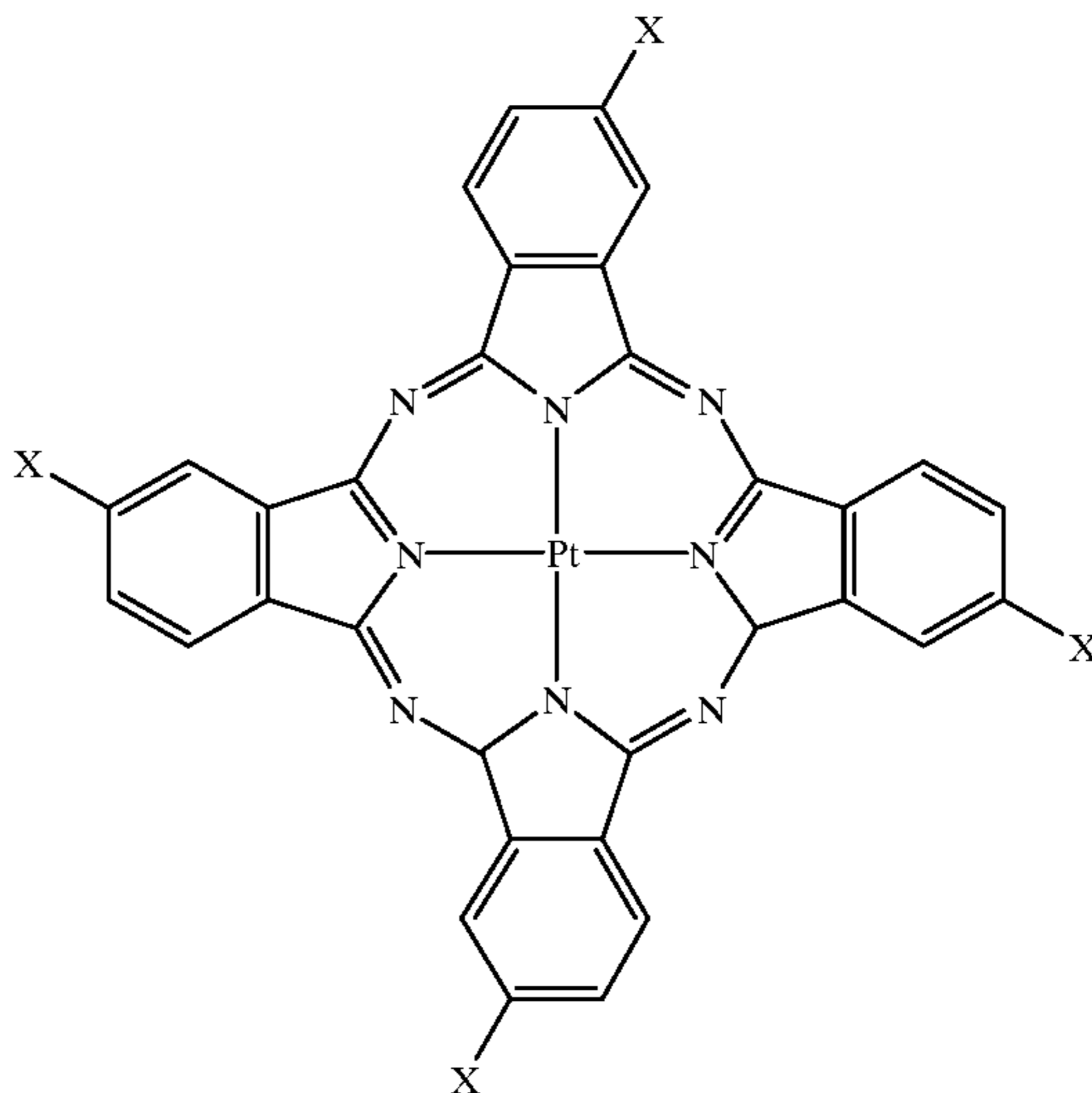
X = H PT-PHTH-H Compound #13 X = I PT-PHTH-I Compound #14 X = Br PT-PHTH-Br Compound #15
