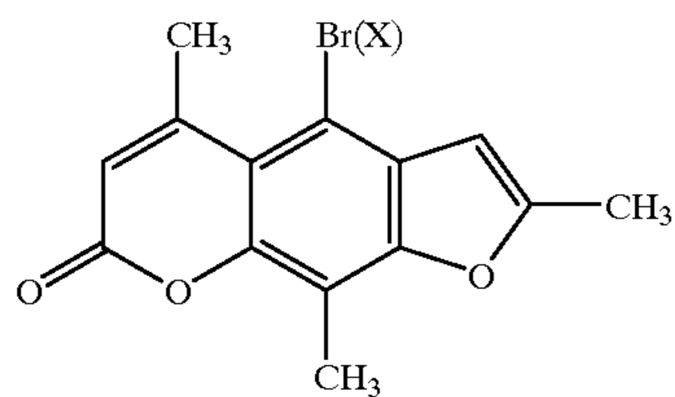
Compound #10 X = I, Compound #10b
