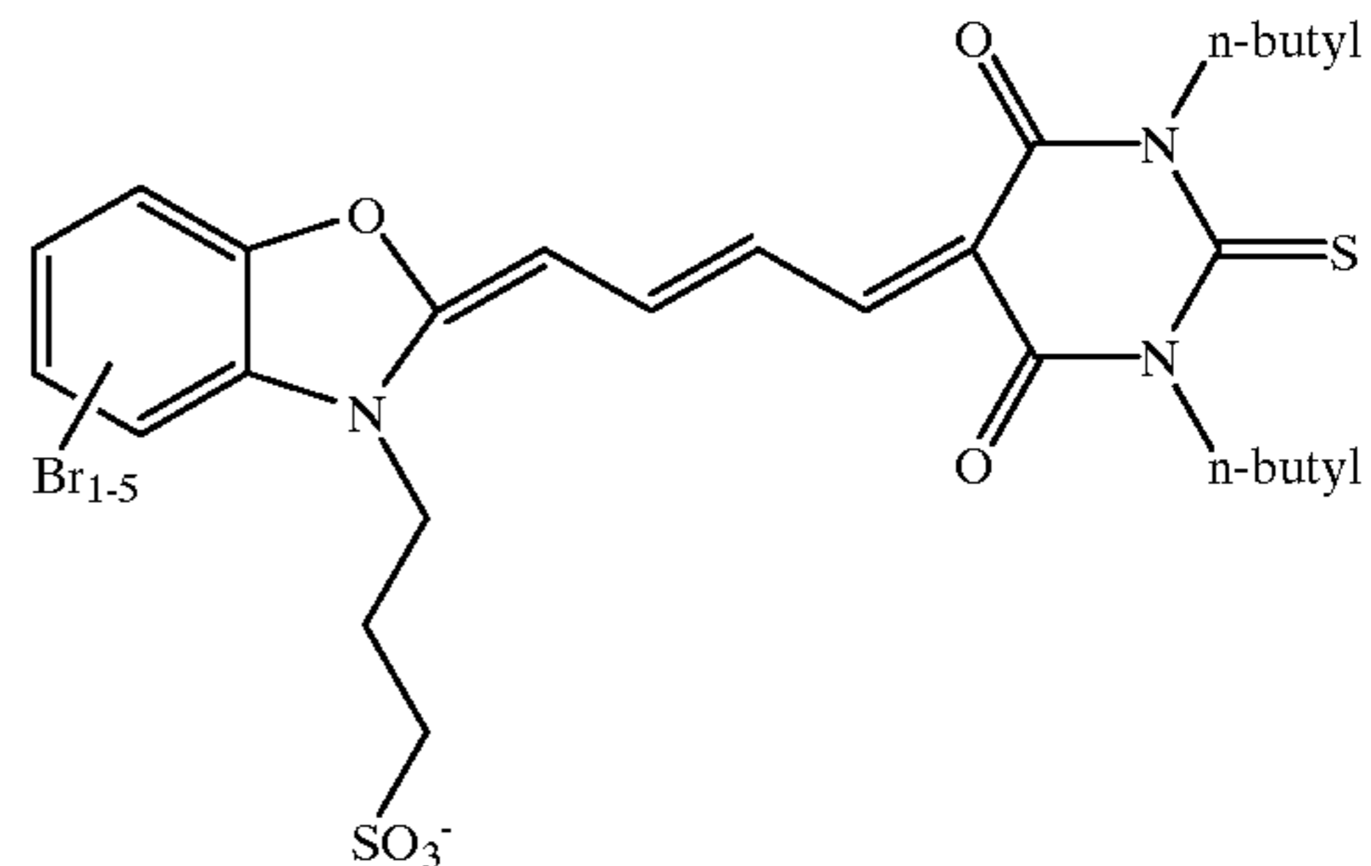
X = H PT-PHTH-H Compound #13 X = I PT-PHTH-I Compound #14 X = Br PT-PHTH-Br Compound #15
