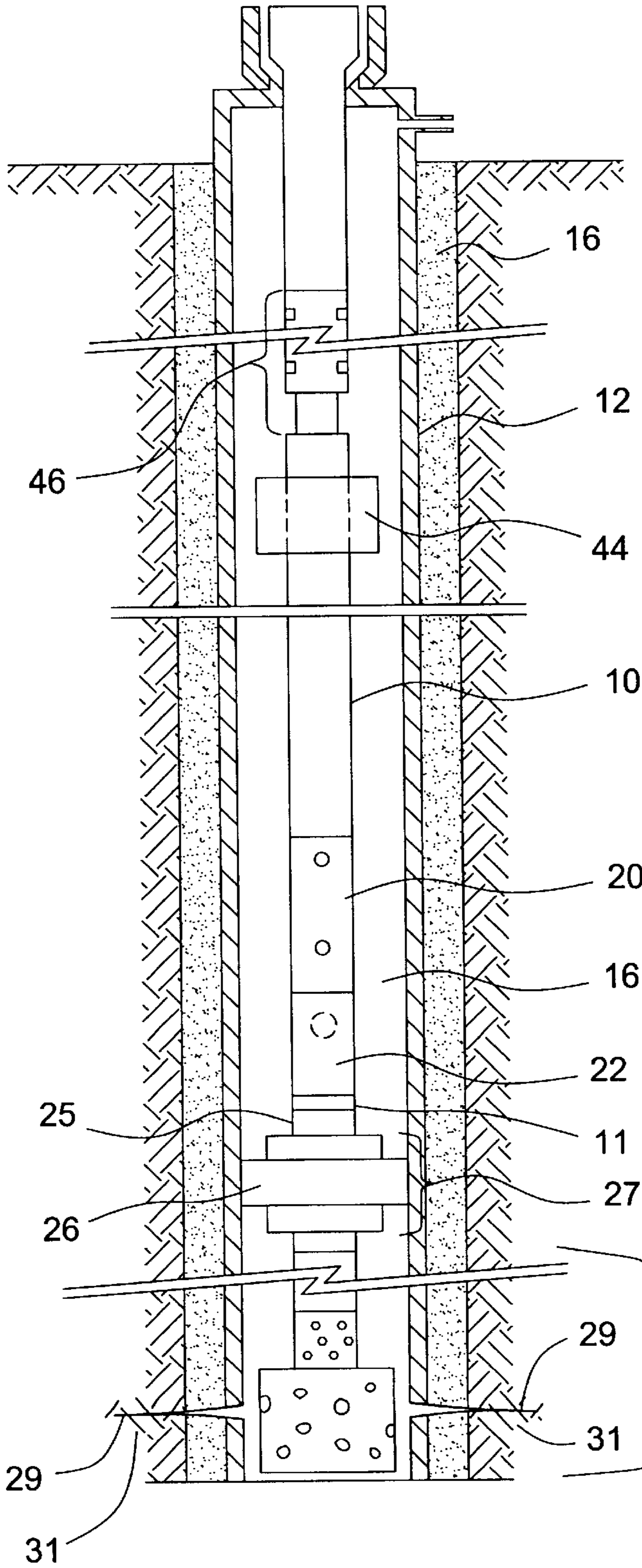
ANNULUS 16 PRESSURE
