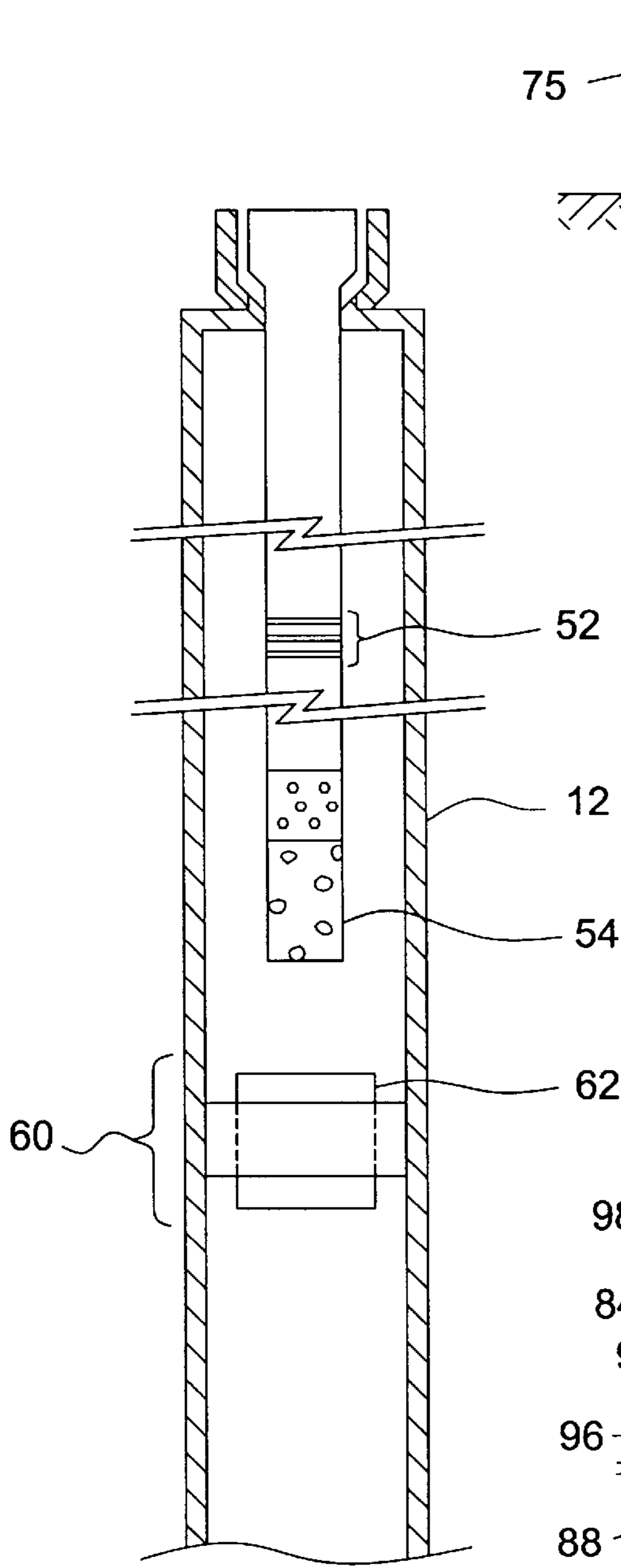
FIG. 3 (PRIOR ART)
