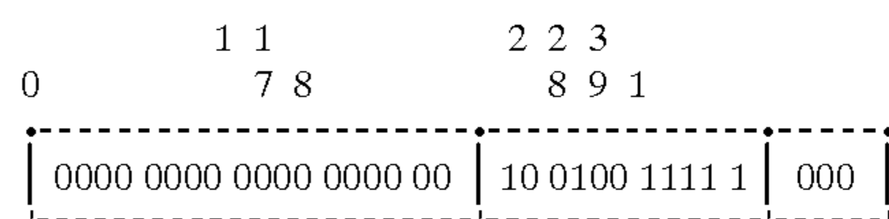
CHANNEL 32 BIT TIME VALUE
