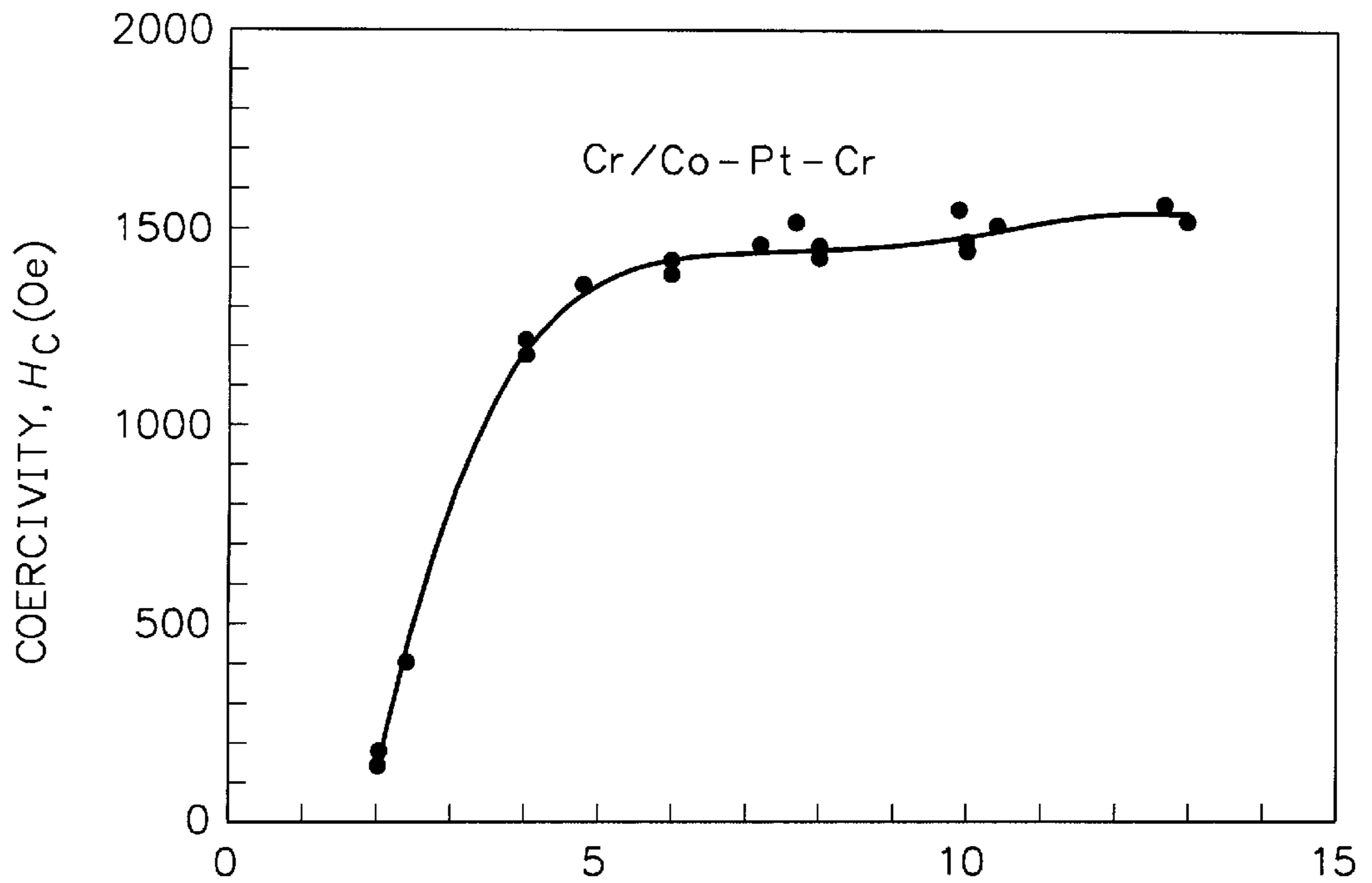
FIG. 13 Cr/Co-Pt-Cr FILM THICKNESS (nm)
