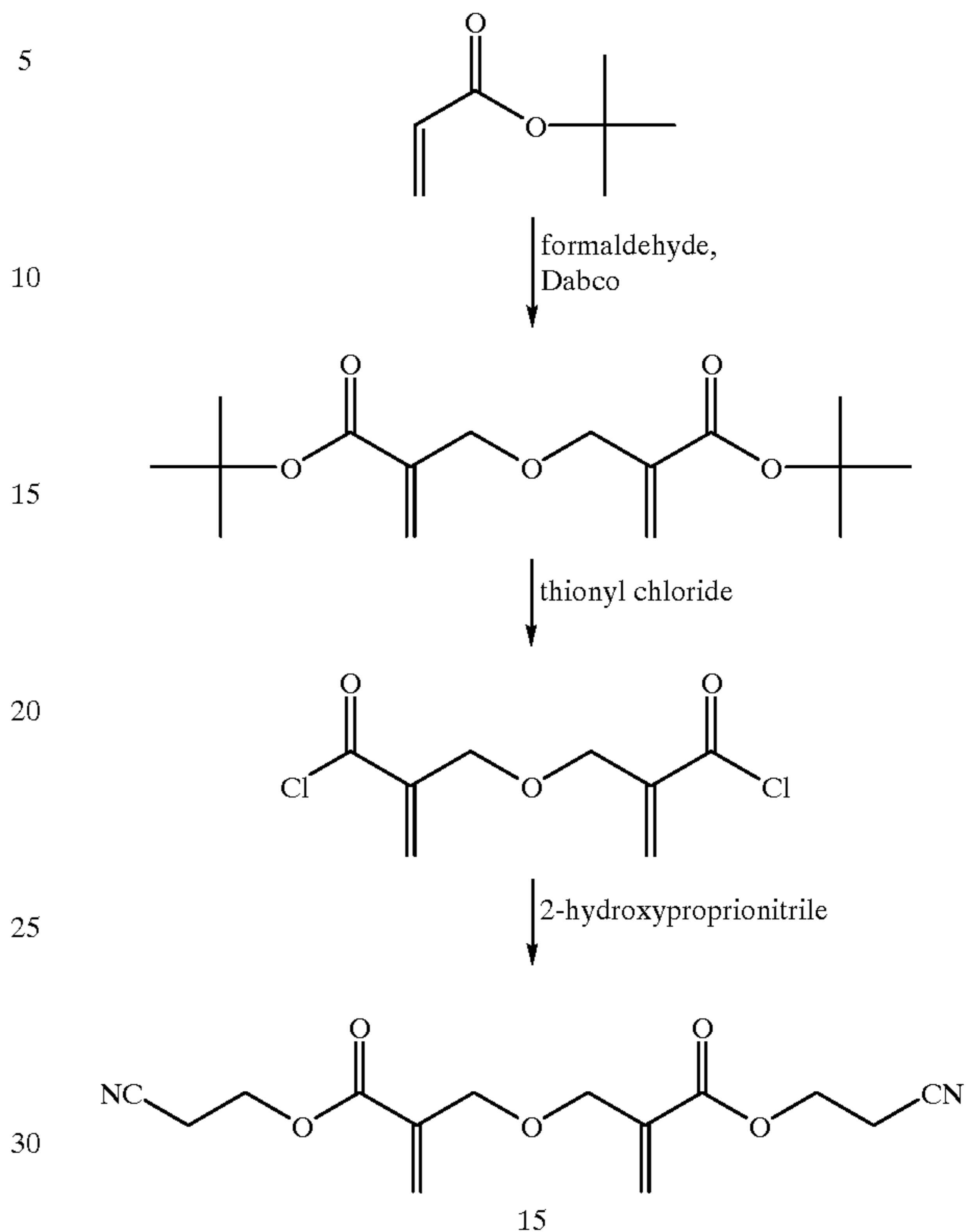
Scheme 7 Alternative synthesis of di(2-cyanoethyl) oxybismethacrylate
