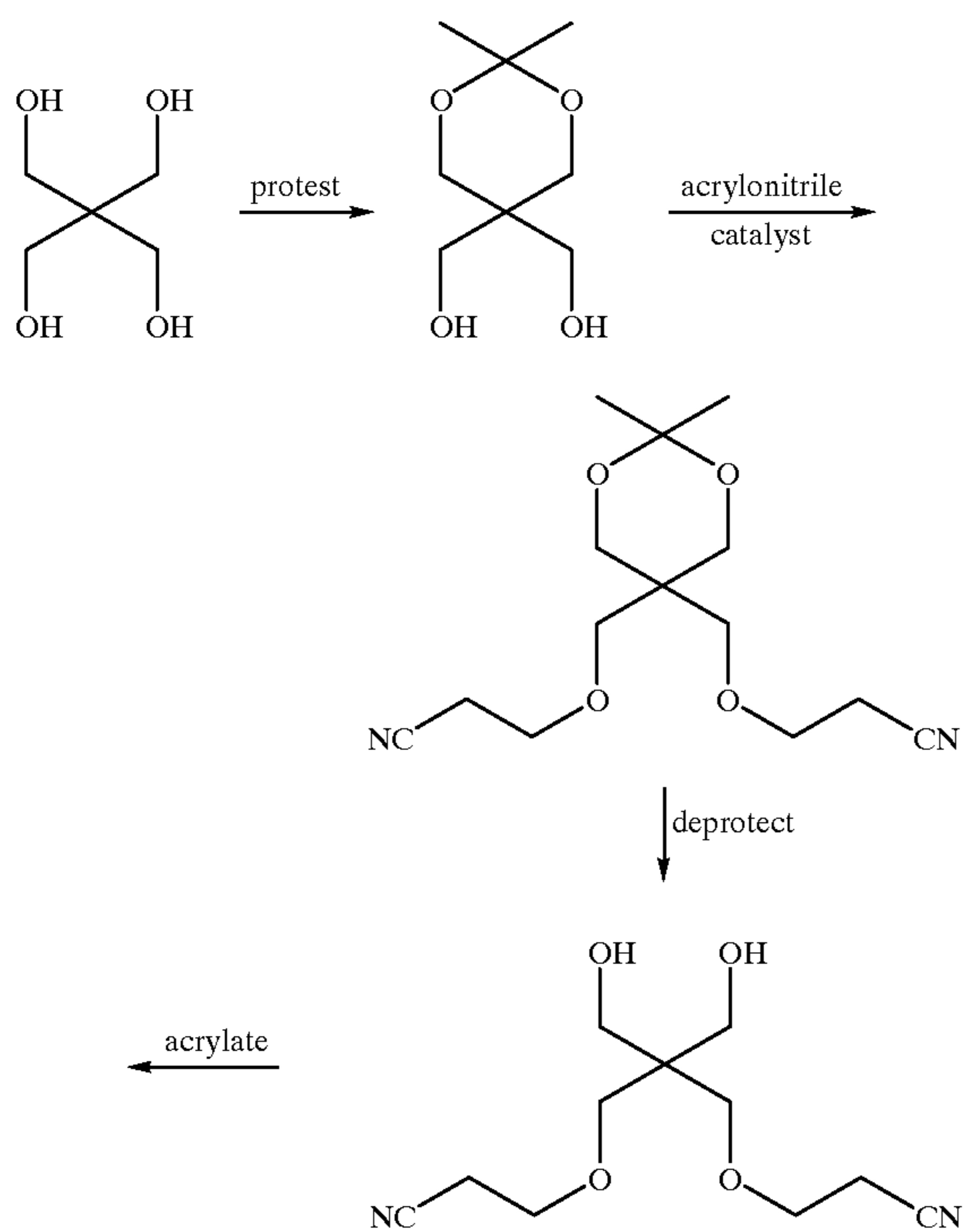
Scheme 4 Synthesis of a monomer based on cyanoethylated pentaerythritol
