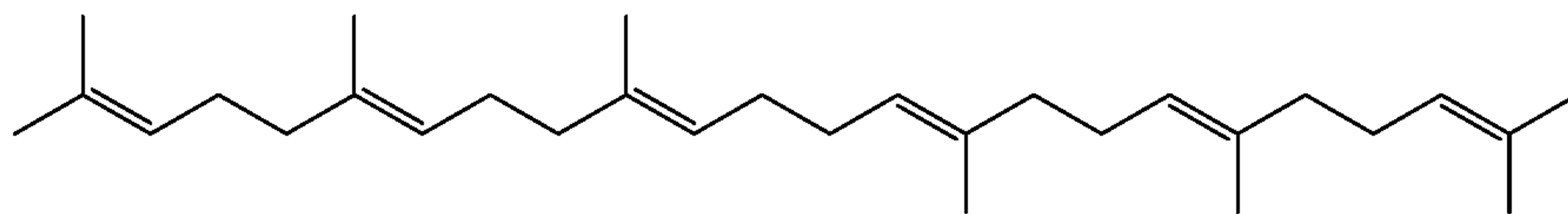
mevalonate
