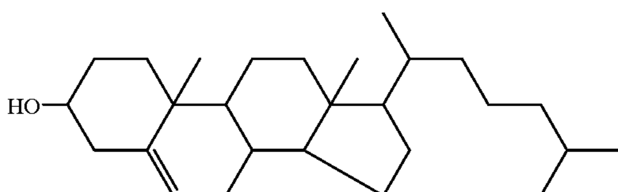
cholesterol
