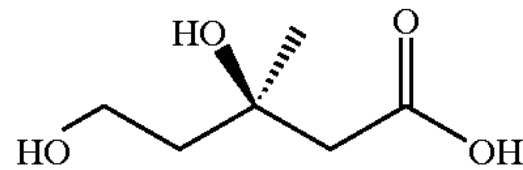
mevalonate
