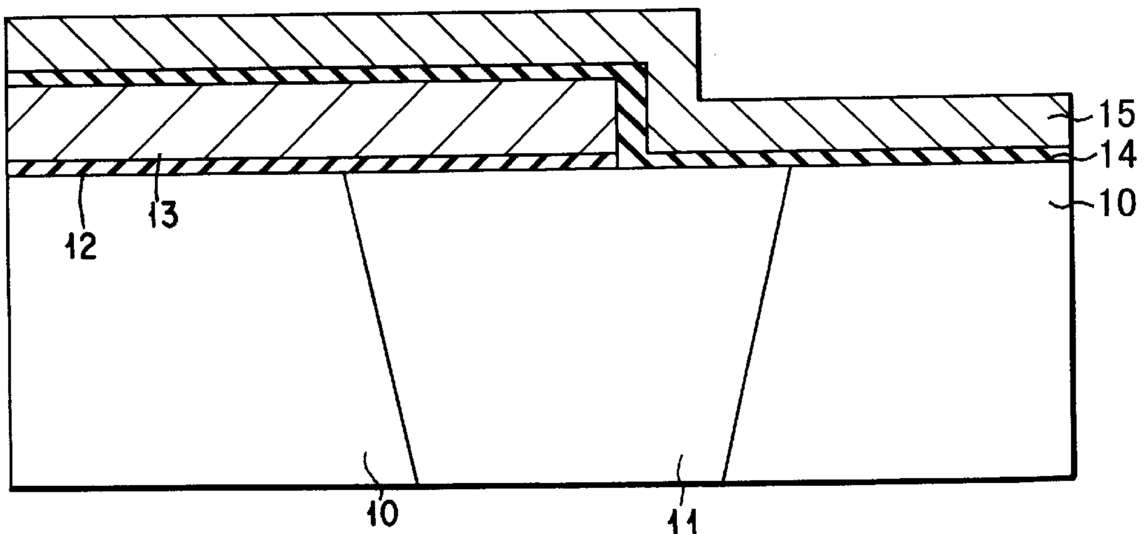
FIG. 3C (PRIOR ART)
