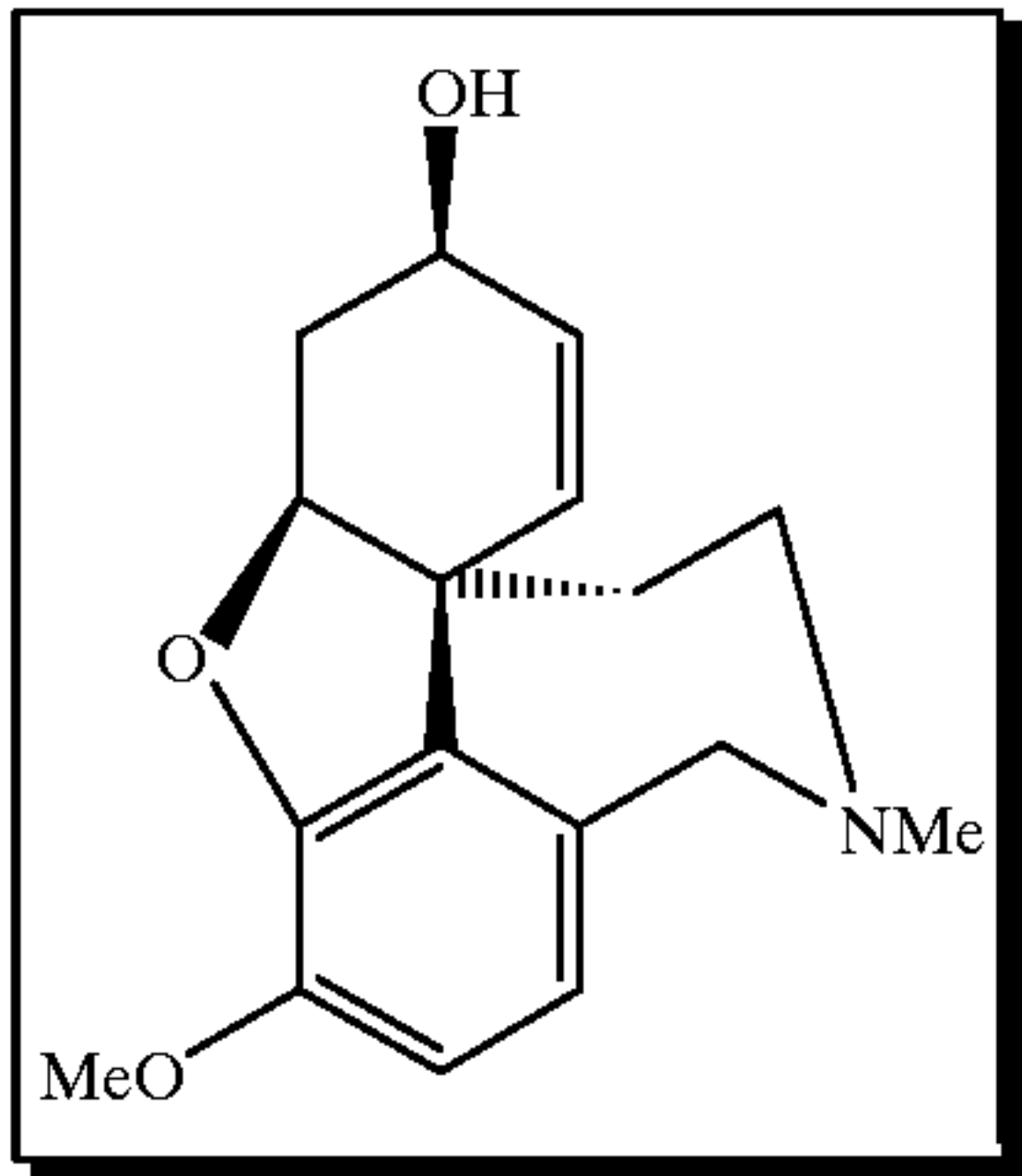
(-)-Galanthamine
