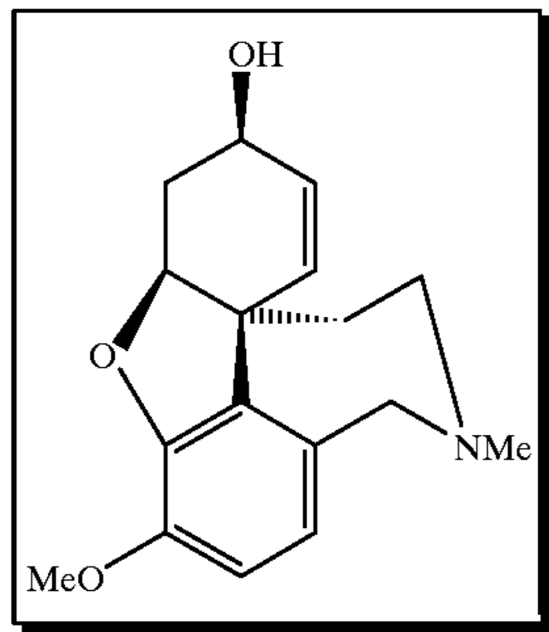
(-)-Galanthamine
