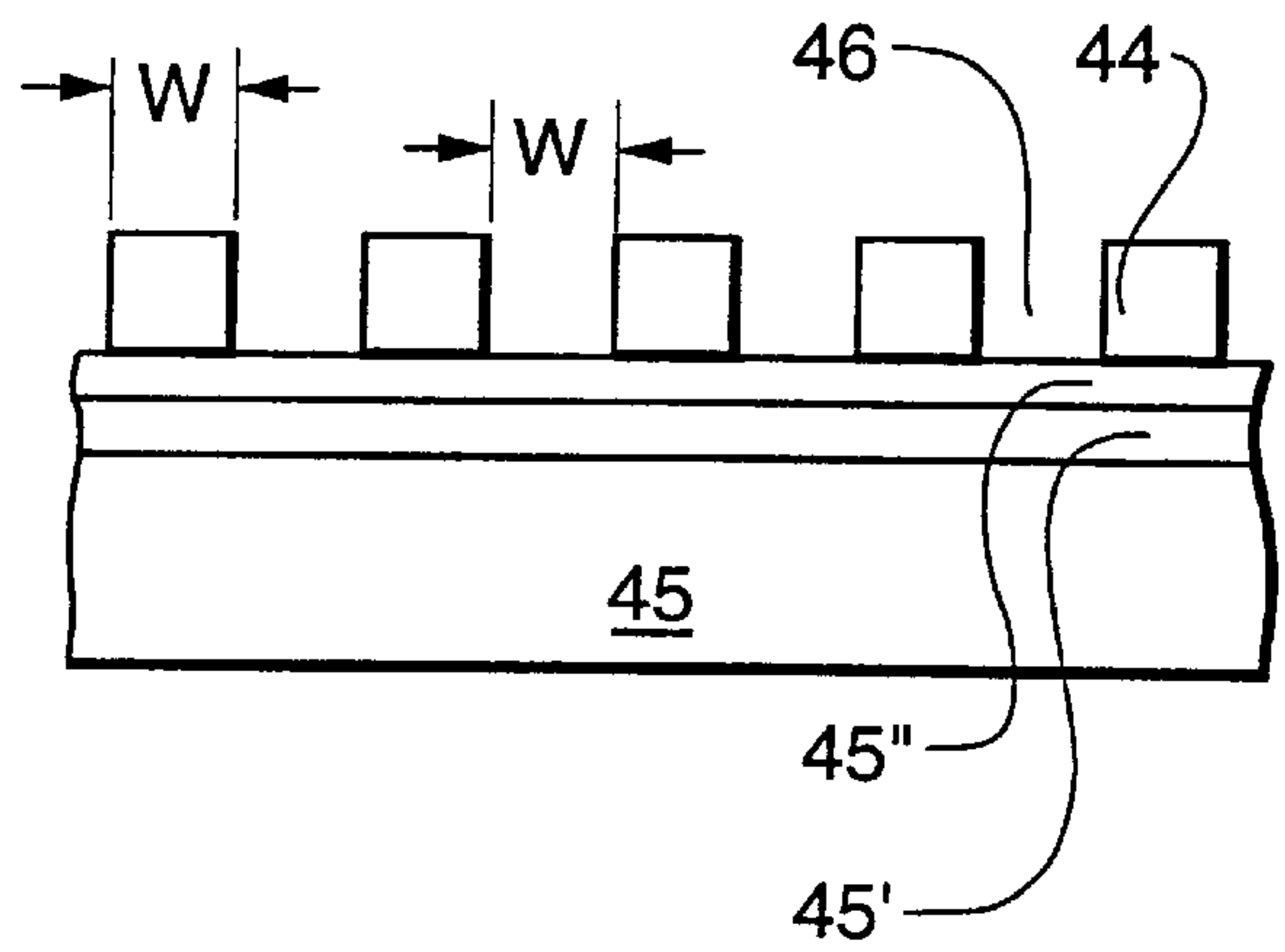
FIG. 2 (PRIOR ART)
