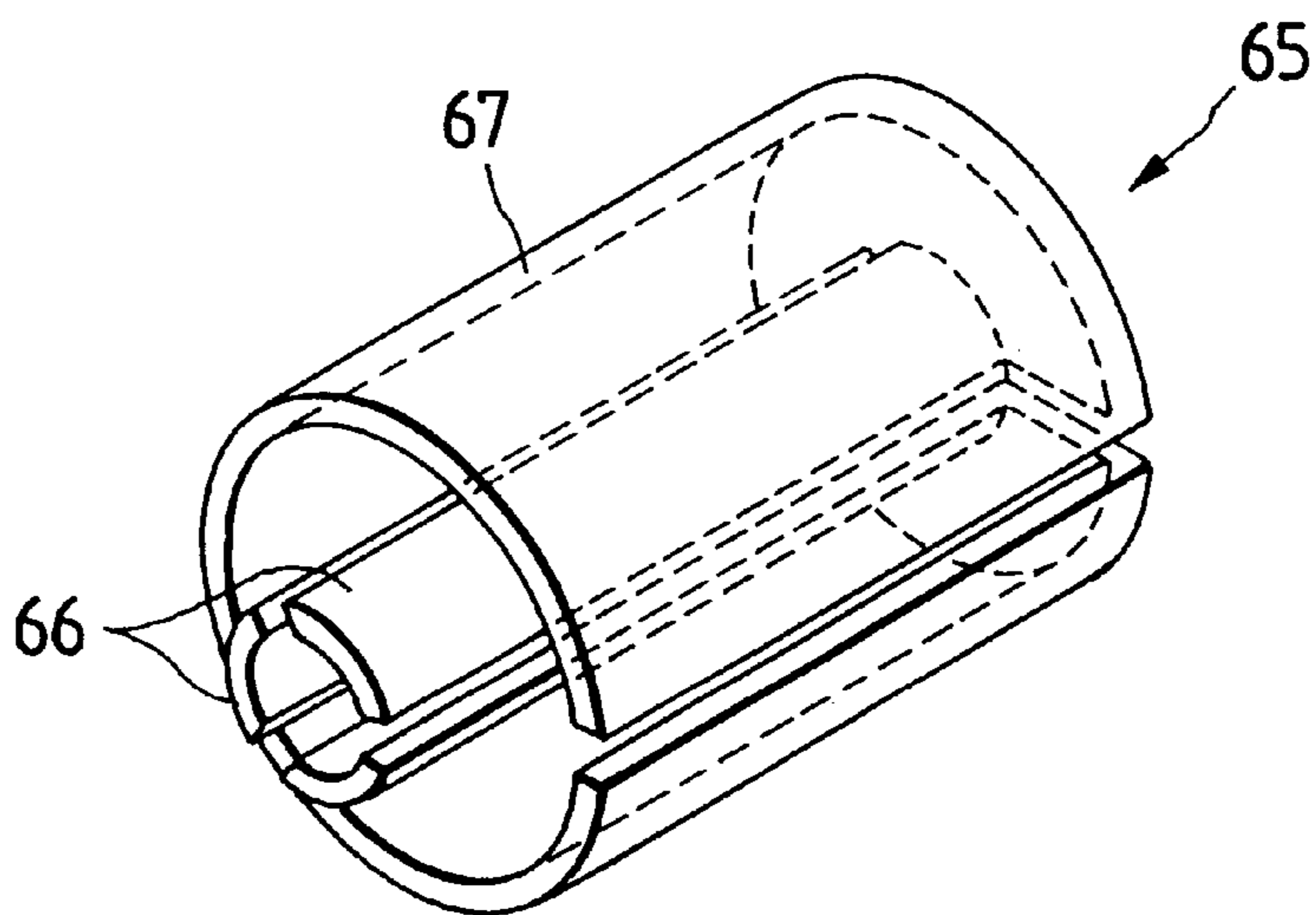
FIG. 15 PRIOR ART
