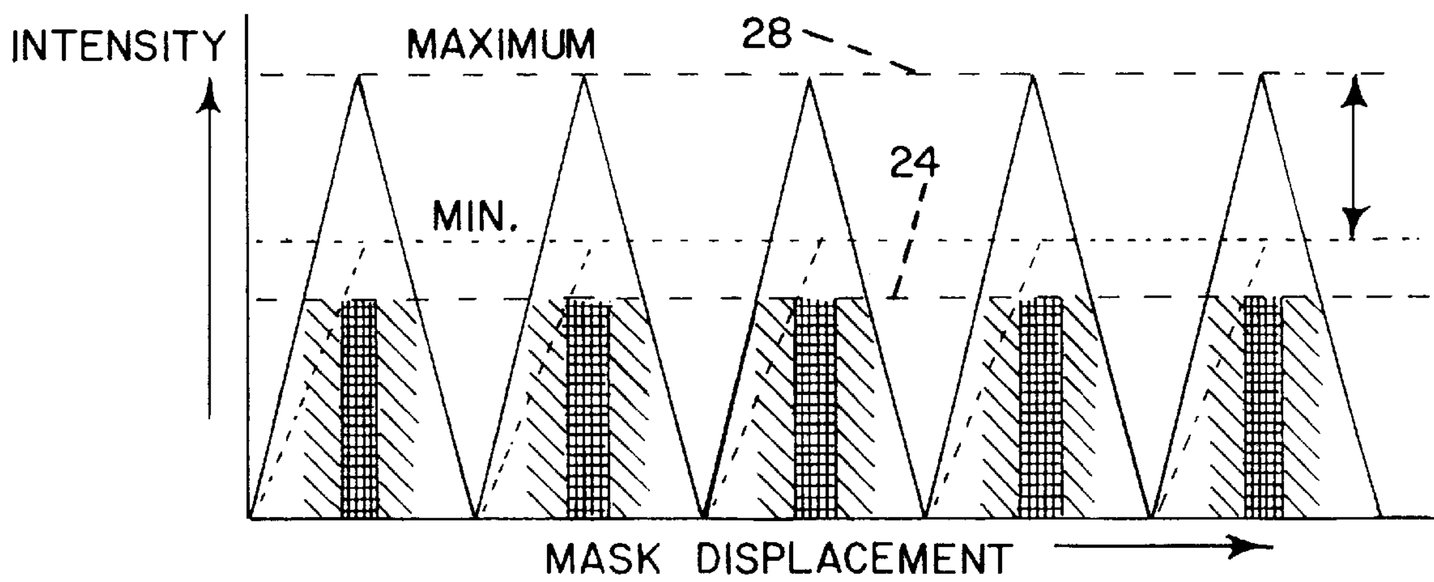
FIG 4(PRIOR ART)
