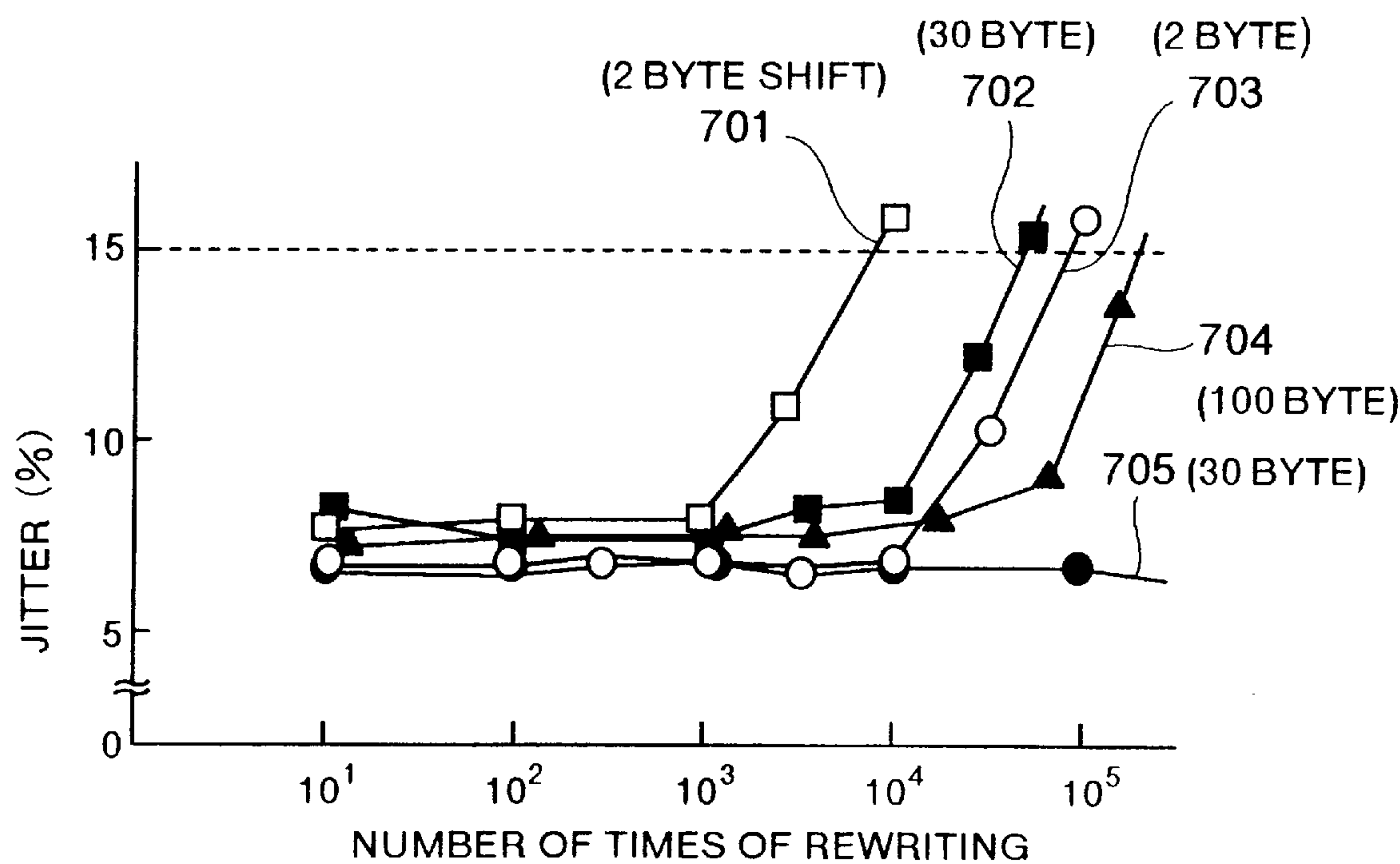
FIG.7 PRIOR ART
