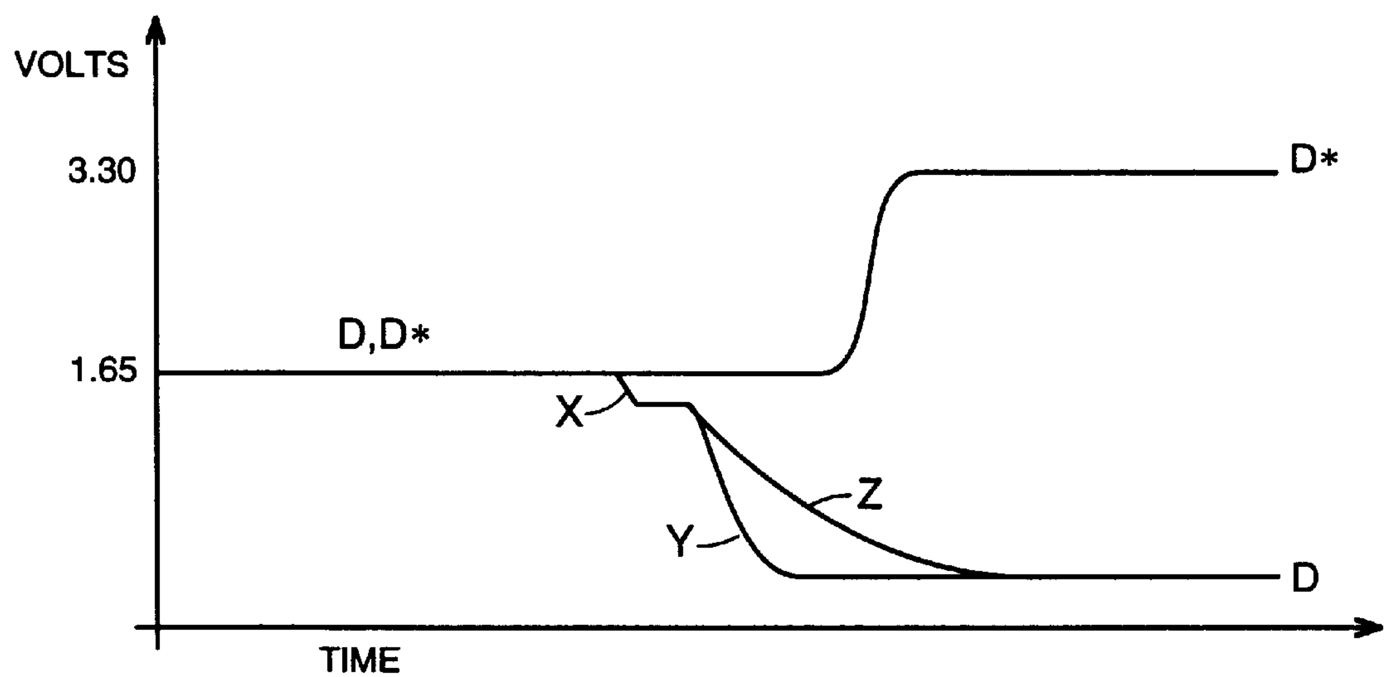
FIG. 2 (PRIOR ART)
