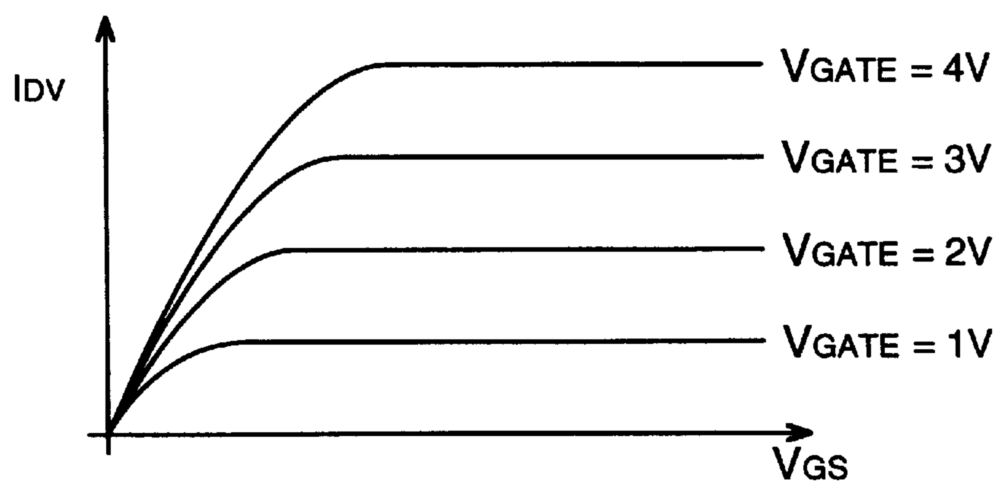
FIG. 3 (PRIOR ART)
