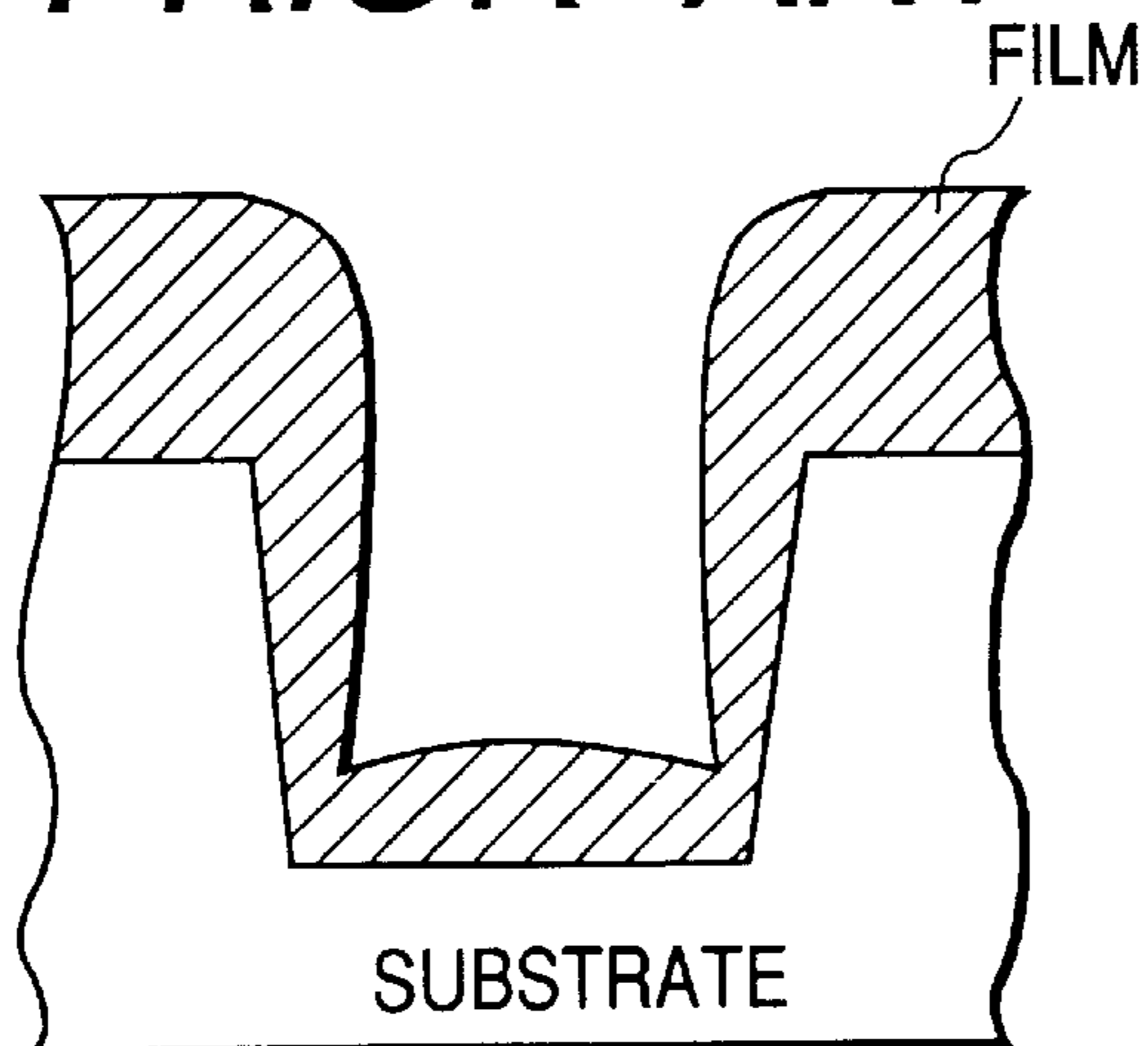
FIG. 14C PRIOR ART
